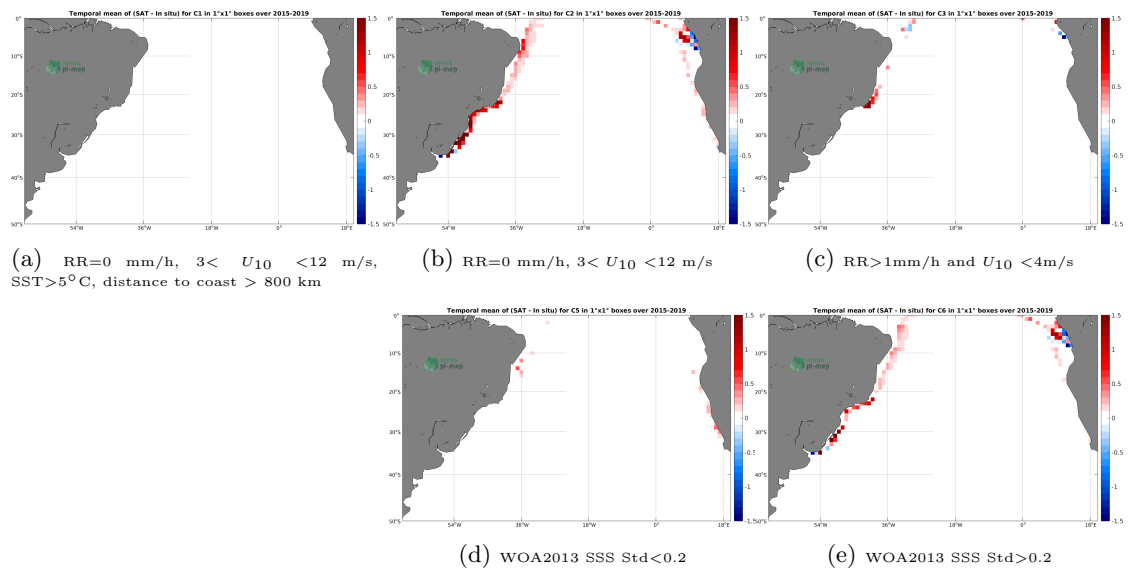
Figure 12: Temporal mean gridded over spatial boxes of size 1^\circ \times 1^\circ of \Delta SSS (SMAP SSS L3 v5.0 - Monthly (JPL) - TSG (LEGOS-DM)) for 5 different subdatasets corresponding to: RR=0 mm/h, 3 < U_{10} < 12 m/s, SST > 5°C, distance to coast > 800 km (a), RR=0 mm/h, 3 < U_{10} < 12 m/s (b), RR > 1mm/h and U_{10} < 4 m/s (c), WOA2013 SSS Std < 0.2 (d), WOA2013 SSS Std > 0.2 (e).
