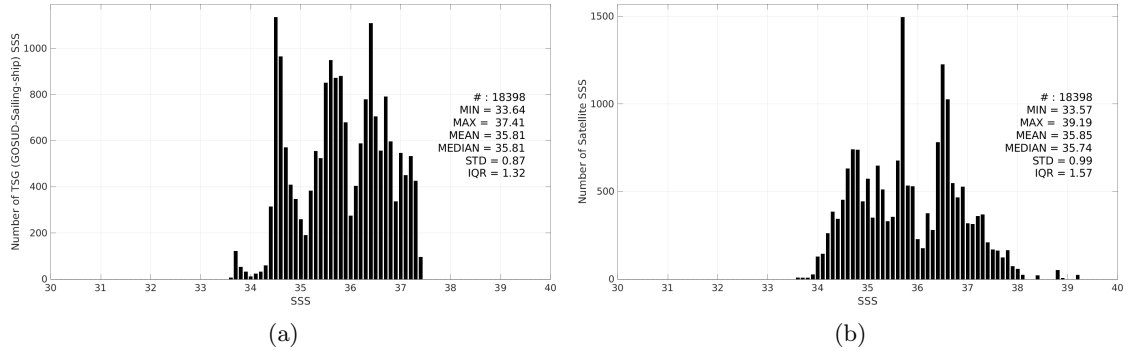
Figure 3: Histograms of SSS from TSG (GOSUD-Sailing-ship) (a) and SMAP SSS L3 v5.0 - Monthly (JPL) (b) considering all match-up pairs per bins of 0.1 over the South Atlantic Ocean Pi-MEP region and for the full satellite product period.
