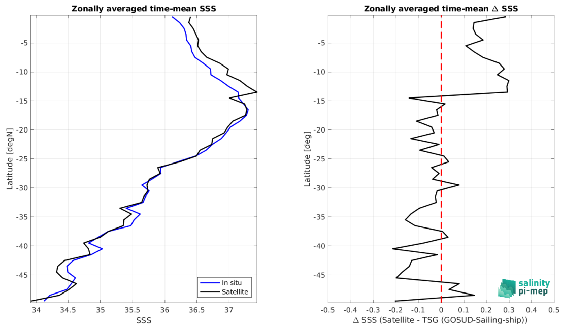
Figure 9: Left panel: Zonal mean SSS from SMAP SSS L3 v5.0 - Monthly (JPL) satellite product (black) and from TSG (GOSUD-Sailing-ship) (blue). Right panel: Zonal mean of \Delta SSS (Satellite - TSG (GOSUD-Sailing-ship)) for all the collected Pi-MEP match-up pairs estimated over the full satellite product period.
