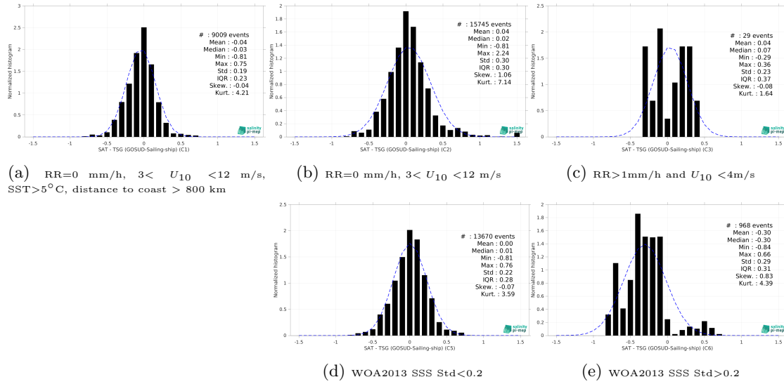
Figure 15: Normalized histogram of \Delta SSS (SMAP SSS L3 v5.0 - Monthly (JPL) - TSG (GOSUD-Sailing-ship)) for 5 different subdatasets corresponding to: RR=0 mm/h, 3 < U_{10} < 12 m/s, SST>5°C, distance to coast > 800 km (a), RR=0 mm/h, 3 < U_{10} < 12 m/s (b), RR>1mm/h and U_{10} < 4 m/s (c), WOA2013 SSS Std<0.2 (d), WOA2013 SSS Std>0.2 (e).
