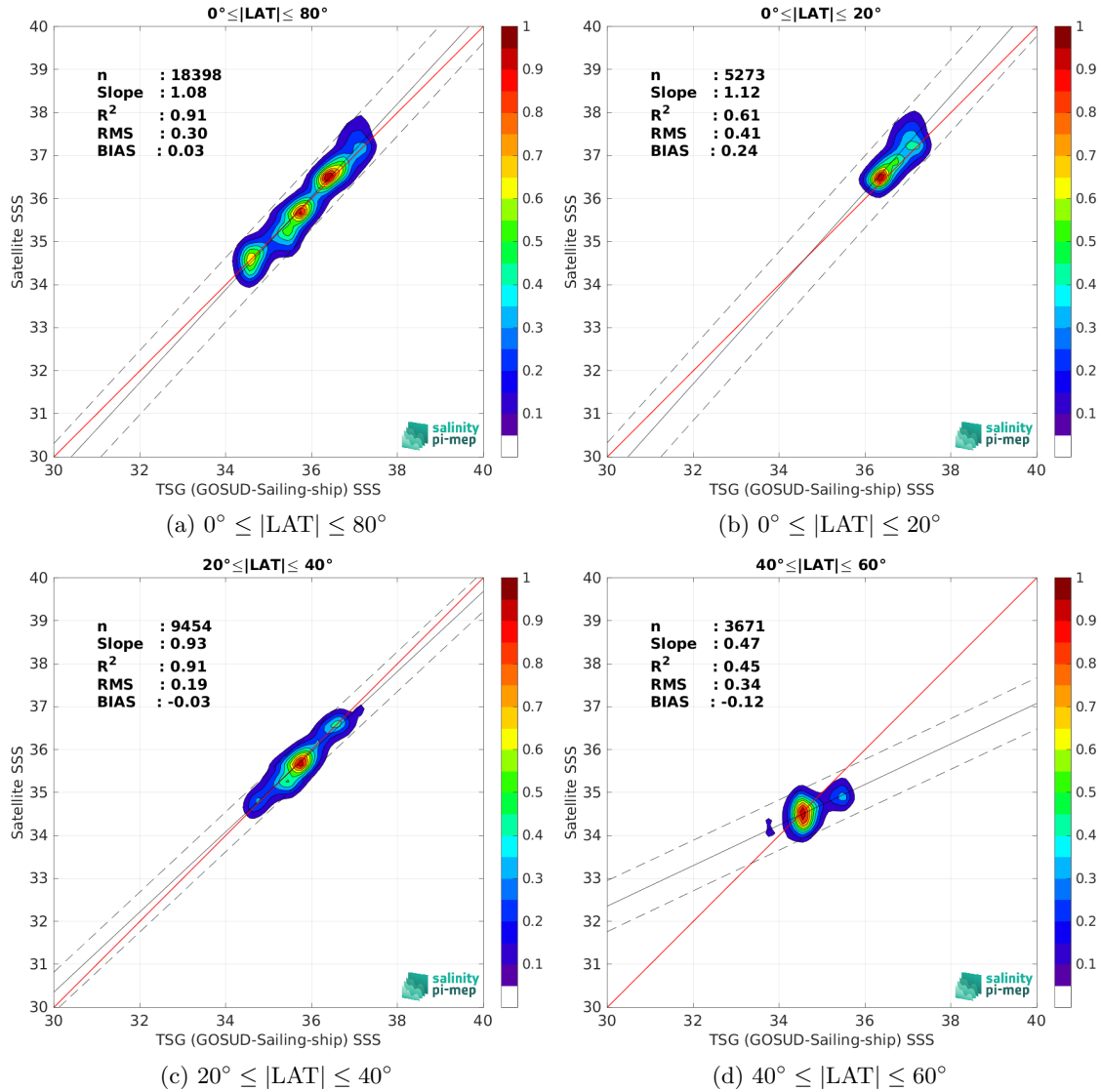
Figure 10: Contour maps of the concentration of SMAP SSS L3 v5.0 - Monthly (JPL) SSS (y-axis) versus TSG (GOSUD-Sailing-ship) SSS (x-axis) at match-up pairs for different latitude bands. For each plot, the red line shows x=y . The black thin and dashed lines indicate a linear fit through the data cloud and the \pm 95\% confidence levels, respectively. The number match-up pairs n , the slope and R^2 coefficient of the linear fit, the root mean square (RMS) and the mean bias between satellite and in situ data are indicated for each latitude band in each plots.
