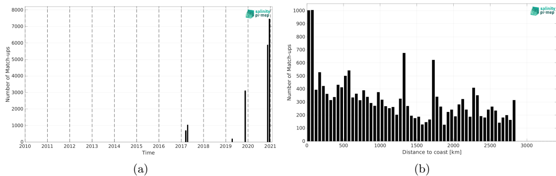
Figure 2: Number of match-ups between TSG (GOSUD-Sailing-ship) and SMAP SSS L3 v5.0 - Monthly (JPL) SSS as a function of time (a) and as function of the distance to coast (b) over the South Atlantic Ocean Pi-MEP region and for the full satellite product period.
