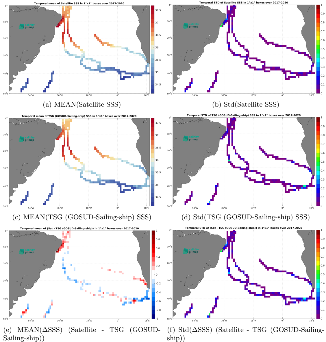
Figure 7: Temporal mean (left) and Std (right) of SSS from SMAP SSS L3 v5.0 - Monthly (JPL) (top), TSG (GOSUD-Sailing-ship) (middle), and of \Delta SSS (Satellite - TSG (GOSUD-Sailing-ship)). Only match-up pairs are used to generate these maps.
