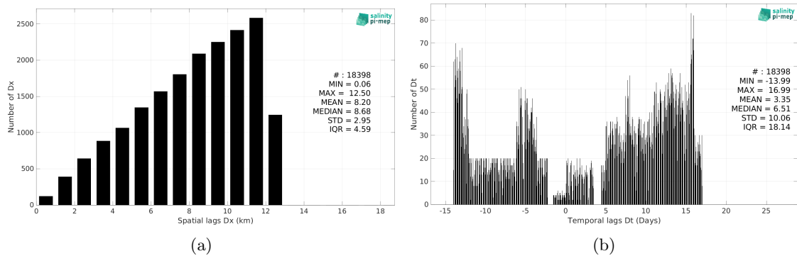
Figure 6: Histograms of the spatial (a) and temporal (b) lags between the location/time of the TSG (GOSUD-Sailing-ship) measurement and the date of the corresponding SMAP SSS L3 v5.0 - Monthly (JPL) SSS pixel.
