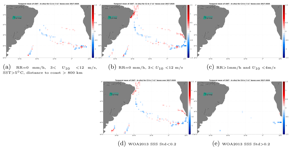
Figure 14: Temporal mean gridded over spatial boxes of size 1^\circ \times 1^\circ of \Delta SSS (SMAP SSS L3 v5.0 - Monthly (JPL) - TSG (GOSUD-Sailing-ship)) for 5 different subdatasets corresponding to:RR=0 mm/h, 3 < U_{10} < 12 m/s, SST >5^\circ\text{C} , distance to coast > 800 km (a), RR=0 mm/h, 3 < U_{10} < 12 m/s (b), RR >1 mm/h and U_{10} < 4 m/s (c), WOA2013 SSS Std <0.2 (d), WOA2013 SSS Std >0.2 (e).
