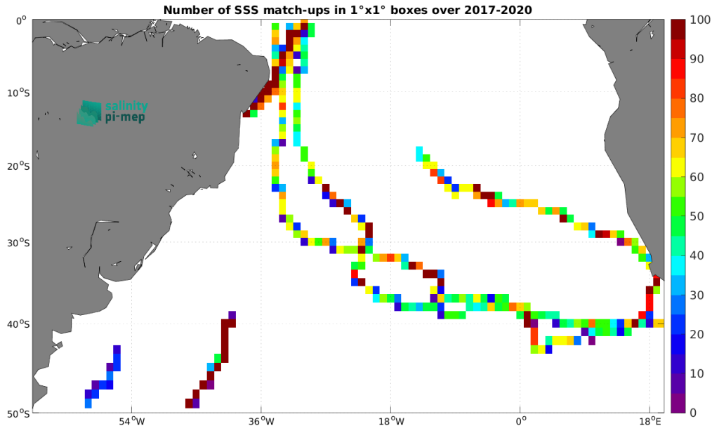
Figure 5: Number of SSS match-ups between TSG (GOSUD-Sailing-ship) SSS and the SMAP SSS L3 v5.0 - Monthly (JPL) SSS product for the South Atlantic Ocean Pi-MEP region over 1^\circ \times 1^\circ boxes and for the full satellite product period.
