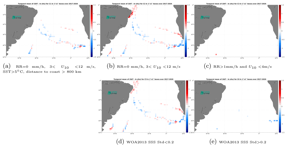
Figure 12: Temporal mean gridded over spatial boxes of size 1^\circ \times 1^\circ of \Delta\text{SSS} (SMAP SSS L3 v5.0 - Monthly (JPL) - TSG (GOSUD-Sailing-ship)) for 5 different subdatasets corresponding to:RR=0 mm/h, 3 < U_{10} < 12 m/s, SST >5^\circ\text{C} , distance to coast > 800 km (a), RR=0 mm/h, 3 < U_{10} < 12 m/s (b), RR >1 mm/h and U_{10} < 4 m/s (c), WOA2013 SSS Std <0.2 (d), WOA2013 SSS Std >0.2 (e).
