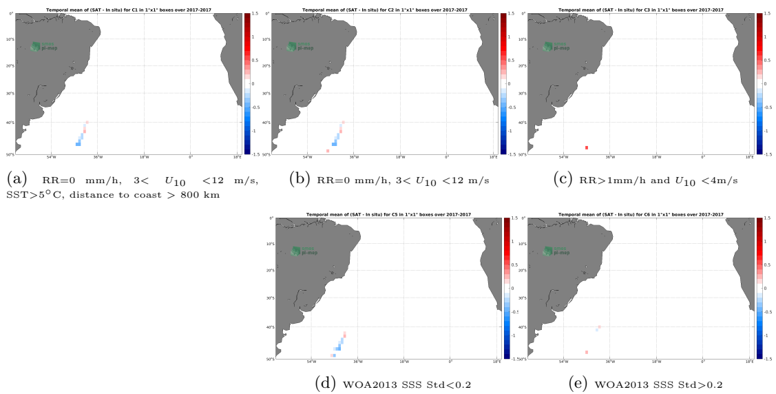
Figure 12: Temporal mean gridded over spatial boxes of size 1°x1° of \Delta SSS (SMAP SSS L3 v5.0 - Monthly (JPL) - TSG (GOSUD-Sailing-ship)) for 5 different subdatasets corresponding to: RR=0 mm/h, 3 < U_{10} < 12 m/s, SST > 5°C, distance to coast > 800 km (a), RR=0 mm/h, 3 < U_{10} < 12 m/s (b), RR > 1mm/h and U_{10} < 4 m/s (c), WOA2013 SSS Std < 0.2 (d), WOA2013 SSS Std > 0.2 (e).
