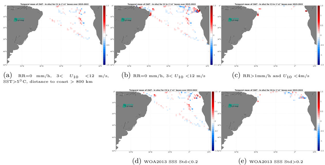
Figure 14: Temporal mean gridded over spatial boxes of size 1^\circ \times 1^\circ of \Delta\text{SSS} (SMAP SSS L3 v5.0 - Monthly (JPL) - TSG (GOSUD-Research-vessel)) for 5 different subdatasets corresponding to:RR=0 mm/h, 3 < U_{10} < 12 m/s, SST >5^\circ\text{C} , distance to coast > 800 km (a), RR=0 mm/h, 3 < U_{10} < 12 m/s (b), RR >1 mm/h and U_{10} < 4 m/s (c), WOA2013 SSS Std <0.2 (d), WOA2013 SSS Std >0.2 (e).
