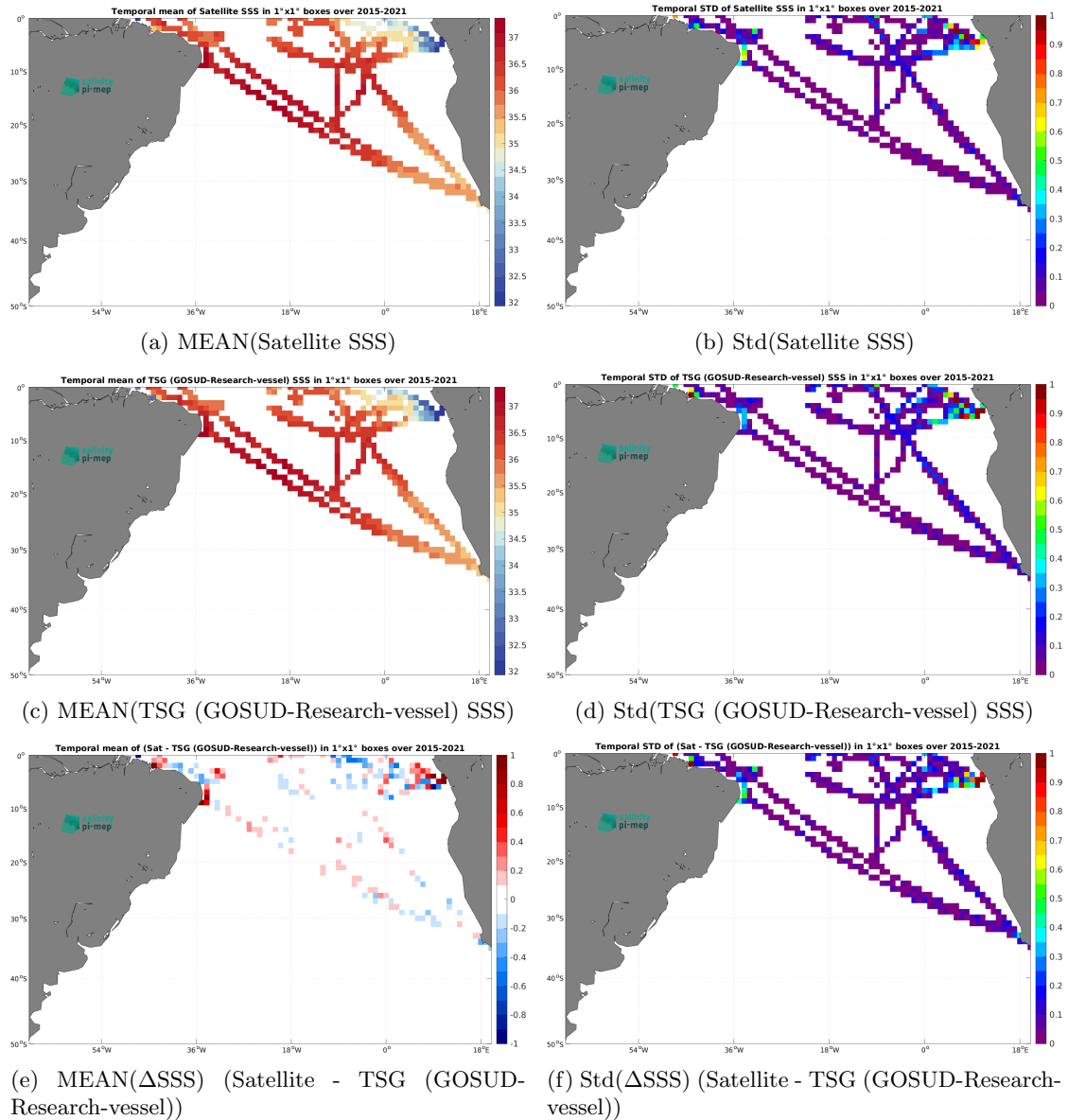
Figure 7: Temporal mean (left) and Std (right) of SSS from SMAP SSS L3 v5.0 - Monthly (JPL) (top), TSG (GOSUD-Research-vessel) (middle), and of \Delta SSS (Satellite - TSG (GOSUD-Research-vessel)). Only match-up pairs are used to generate these maps.
