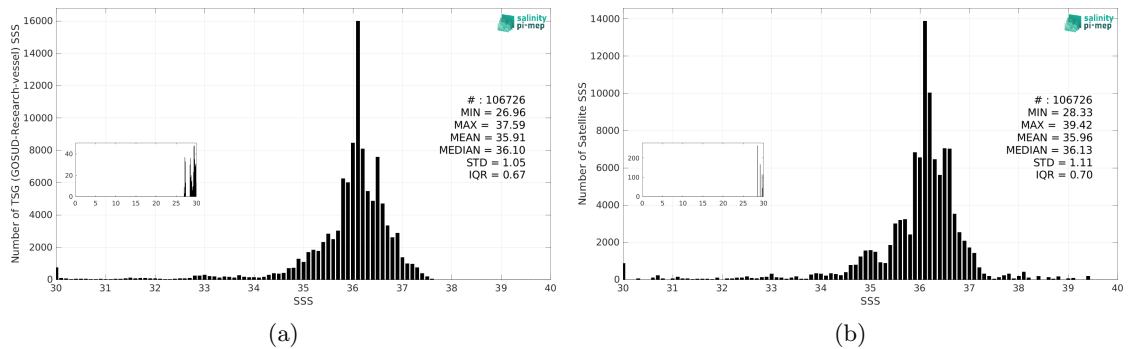
Figure 3: Histograms of SSS from TSG (GOSUD-Research-vessel) (a) and SMAP SSS L3 v5.0 - Monthly (JPL) (b) considering all match-up pairs per bins of 0.1 over the South Atlantic Ocean Pi-MEP region and for the full satellite product period.
