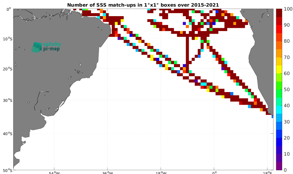
Figure 5: Number of SSS match-ups between TSG (GOSUD-Research-vessel) SSS and the SMAP SSS L3 v5.0 - Monthly (JPL) SSS product for the South Atlantic Ocean Pi-MEP region over 1^\circ \times 1^\circ boxes and for the full satellite product period.
