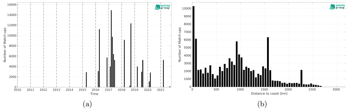
Figure 2: Number of match-ups between TSG (GOSUD-Research-vessel) and SMAP SSS L3 v5.0 - Monthly (JPL) SSS as a function of time (a) and as function of the distance to coast (b) over the South Atlantic Ocean Pi-MEP region and for the full satellite product period.
