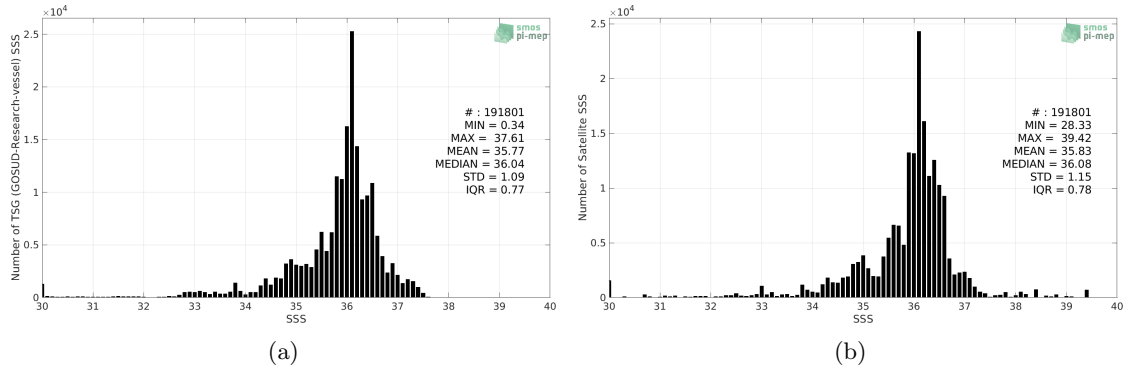
Figure 2: Histograms of SSS from TSG (GOSUD-Research-vessel) (a) and SMAP SSS L3 v5.0 - Monthly (JPL) (b) considering all match-up pairs per bins of 0.1 over the South Atlantic Ocean Pi-MEP region and for the full satellite product period.
