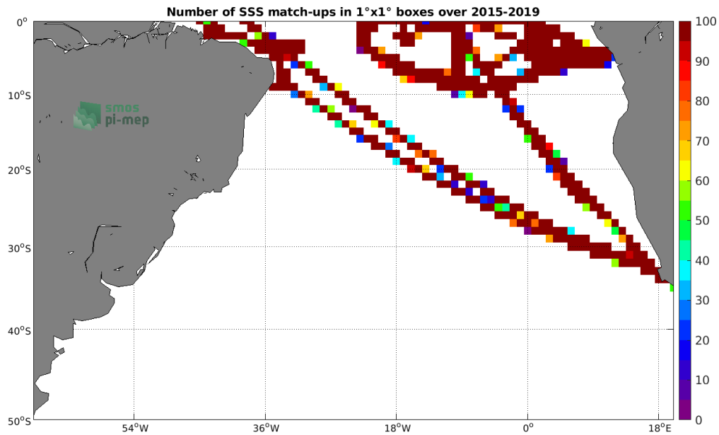
Figure 4: Number of SSS match-ups between TSG (GOSUD-Research-vessel) SSS and the SMAP SSS L3 v5.0 - Monthly (JPL) SSS product for the South Atlantic Ocean Pi-MEP region over 1^{\circ} \times 1^{\circ} boxes and for the full satellite product period.
