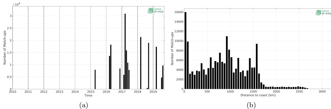
Figure 1: Number of match-ups between TSG (GOSUD-Research-vessel) and SMAP SSS L3 v5.0 - Monthly (JPL) SSS as a function of time (a) and as function of the distance to coast (b) over the South Atlantic Ocean Pi-MEP region and for the full satellite product period.
