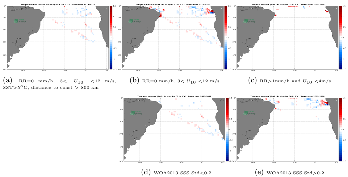
Figure 12: Temporal mean gridded over spatial boxes of size 1°x1° of \Delta SSS (SMAP SSS L3 v5.0 - Monthly (JPL) - TSG (GOSUD-Research-vessel)) for 5 different subdatasets corresponding to:RR=0 mm/h, 3 < U_{10} < 12 m/s, SST>5°C, distance to coast > 800 km (a), RR=0 mm/h, 3 < U_{10} < 12 m/s (b), RR>1mm/h and U_{10} < 4 m/s (c), WOA2013 SSS Std<0.2 (d), WOA2013 SSS Std>0.2 (e).
