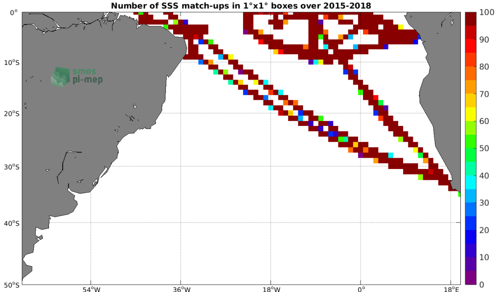
Figure 4: Number of SSS match-ups between TSG (GOSUD-Research-vessel) SSS and the SMAP SSS L3 v5.0 - Monthly (JPL) SSS product for the South Atlantic Ocean Pi-MEP region over 1°x1° boxes and for the full satellite product period.
