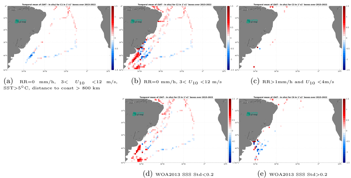
Figure 14: Temporal mean gridded over spatial boxes of size 1^\circ \times 1^\circ of \Delta\text{SSS} (SMAP SSS L3 v5.0 - Monthly (JPL) - TSG (CSIC-UTM)) for 5 different subdatasets corresponding to:RR=0 mm/h, 3 < U_{10} < 12 m/s, SST >5^\circ\text{C} , distance to coast > 800 km (a), RR=0 mm/h, 3 < U_{10} < 12 m/s (b), RR >1 mm/h and U_{10} < 4 m/s (c), WOA2013 SSS Std <0.2 (d), WOA2013 SSS Std >0.2 (e).
