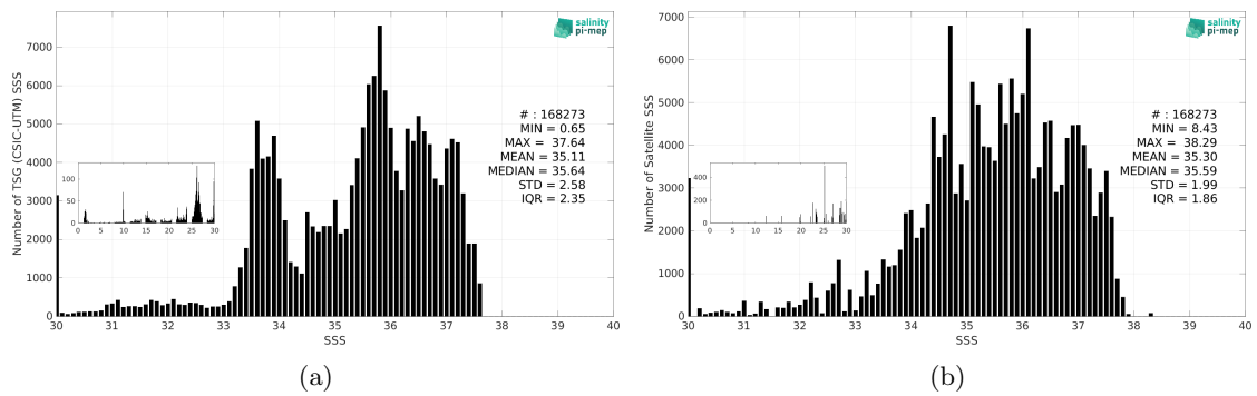
Figure 3: Histograms of SSS from TSG (CSIC-UTM) (a) and SMAP SSS L3 v5.0 - Monthly (JPL) (b) considering all match-up pairs per bins of 0.1 over the South Atlantic Ocean Pi-MEP region and for the full satellite product period.
