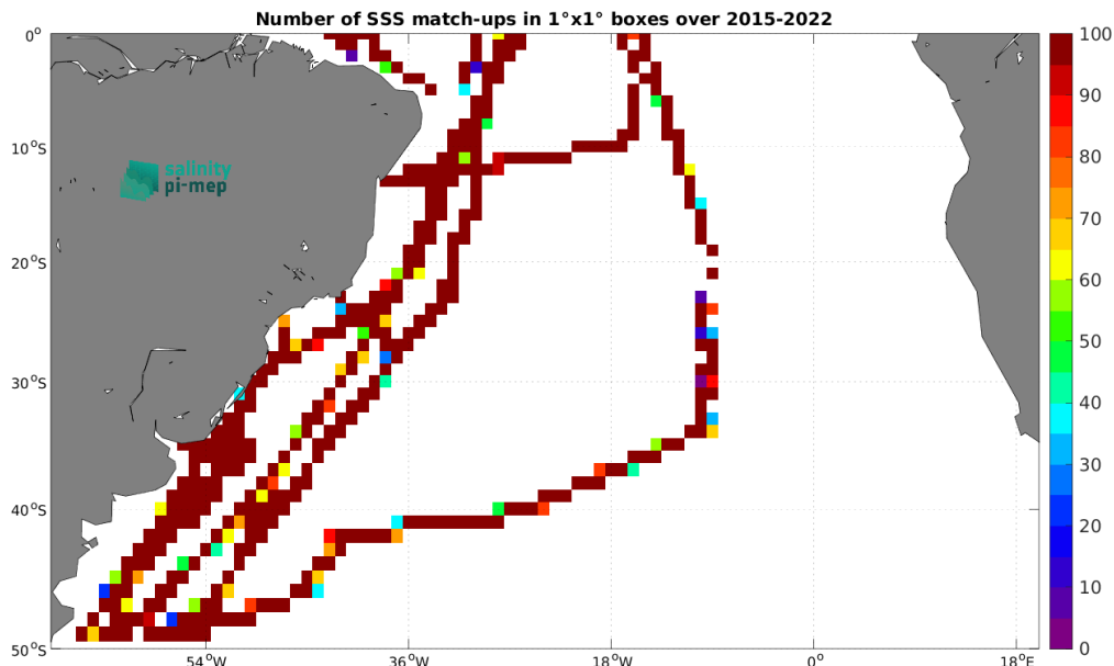
Figure 5: Number of SSS match-ups between TSG (CSIC-UTM) SSS and the SMAP SSS L3 v5.0 - Monthly (JPL) SSS product for the South Atlantic Ocean Pi-MEP region over 1^\circ \times 1^\circ boxes and for the full satellite product period.
