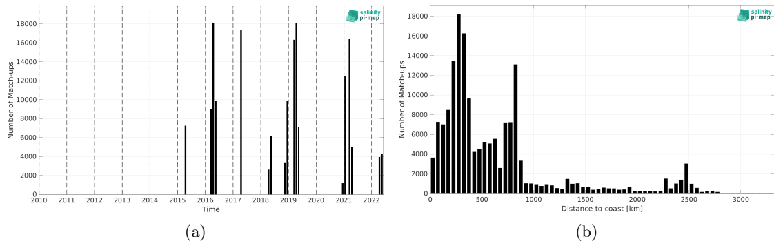
Figure 2: Number of match-ups between TSG (CSIC-UTM) and SMAP SSS L3 v5.0 - Monthly (JPL) SSS as a function of time (a) and as function of the distance to coast (b) over the South Atlantic Ocean Pi-MEP region and for the full satellite product period.
