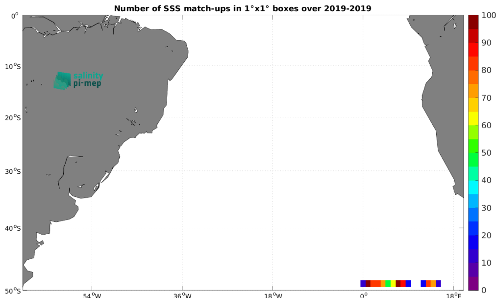
Figure 5: Number of SSS match-ups between Saildrone SSS and the SMAP SSS L3 v5.0 - Monthly (JPL) SSS product for the South Atlantic Ocean Pi-MEP region over 1^\circ \times 1^\circ boxes and for the full satellite product period.
