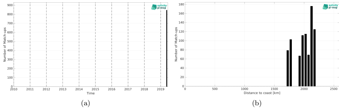
Figure 2: Number of match-ups between Saildrone and SMAP SSS L3 v5.0 - Monthly (JPL) SSS as a function of time (a) and as function of the distance to coast (b) over the South Atlantic Ocean Pi-MEP region and for the full satellite product period.
