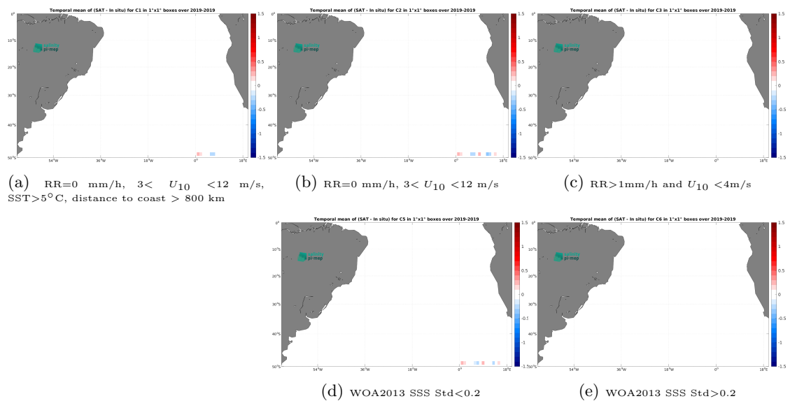
Figure 14: Temporal mean gridded over spatial boxes of size 1^\circ \times 1^\circ of \Delta SSS (SMAP SSS L3 v5.0 - Monthly (JPL) - Saildrone) for 5 different subdatasets corresponding to:RR=0 mm/h, 3 < U_{10} < 12 m/s, SST>5°C, distance to coast > 800 km (a), RR=0 mm/h, 3 < U_{10} < 12 m/s (b), RR>1mm/h and U_{10} < 4 m/s (c), WOA2013 SSS Std<0.2 (d), WOA2013 SSS Std>0.2 (e).
