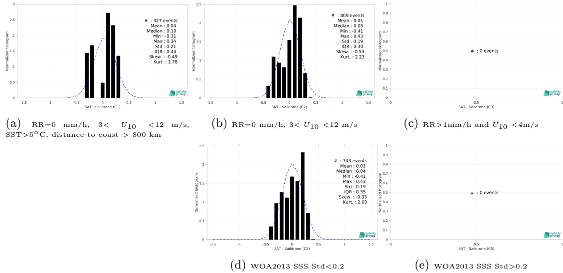
Figure 15: Normalized histogram of \Delta SSS (SMAP SSS L3 v5.0 - Monthly (JPL) - Salldrone) for 5 different subdatasets corresponding to: RR=0 mm/h, 3 < U_{10} < 12 m/s, SST > 5°C, distance to coast > 800 km (a), RR=0 mm/h, 3 < U_{10} < 12 m/s (b), RR > 1mm/h and U_{10} < 4 m/s (c), WOA2013 SSS Std < 0.2 (d), WOA2013 SSS Std > 0.2 (e).
