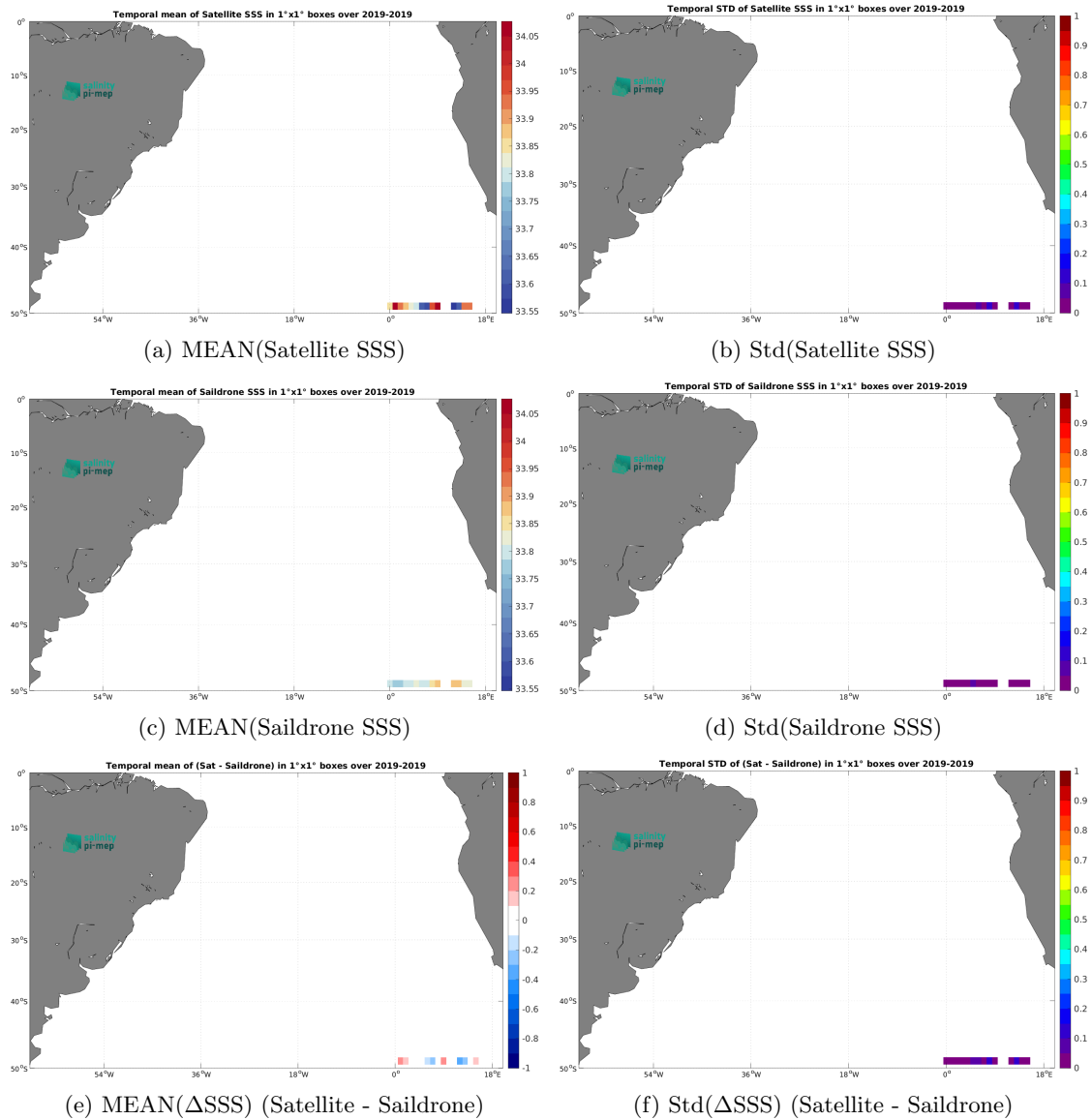
Figure 7: Temporal mean (left) and Std (right) of SSS from SMAP SSS L3 v5.0 - Monthly (JPL) (top), Saildrone (middle), and of \Delta SSS (Satellite - Saildrone). Only match-up pairs are used to generate these maps.
