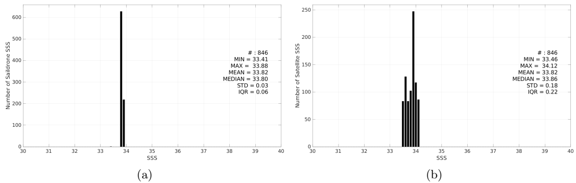
Figure 3: Histograms of SSS from Saildrone (a) and SMAP SSS L3 v5.0 - Monthly (JPL) (b) considering all match-up pairs per bins of 0.1 over the South Atlantic Ocean Pi-MEP region and for the full satellite product period.
