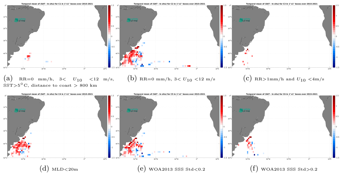
Figure 14: Temporal mean gridded over spatial boxes of size 1^\circ \times 1^\circ of \Delta SSS (SMAP SSS L3 v5.0 - Monthly (JPL) - Marine mammals) for 6 different subdatasets corresponding to:RR=0 mm/h, 3 < U_{10} < 12 m/s, SST>5°C, distance to coast > 800 km (a), RR=0 mm/h, 3 < U_{10} < 12 m/s (b), RR>1mm/h and U_{10} < 4 m/s (c),MLD<20m (d),WOA2013 SSS Std<0.2 (e),WOA2013 SSS Std>0.2 (f).
