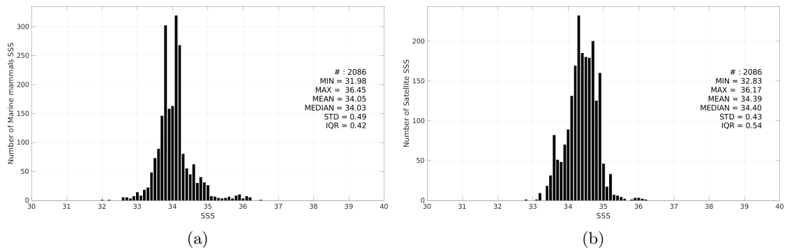
Figure 3: Histograms of SSS from Marine mammals (a) and SMAP SSS L3 v5.0 - Monthly (JPL) (b) considering all match-up pairs per bins of 0.1 over the South Atlantic Ocean Pi-MEP region and for the full satellite product period.
