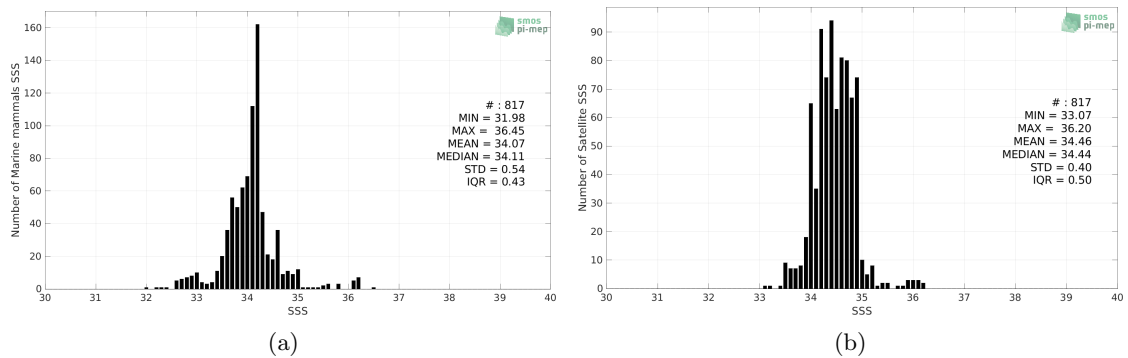
Figure 2: Histograms of SSS from Marine mammals (a) and SMAP SSS L3 v5.0 - Monthly (JPL) (b) considering all match-up pairs per bins of 0.1 over the South Atlantic Ocean Pi-MEP region and for the full satellite product period.
