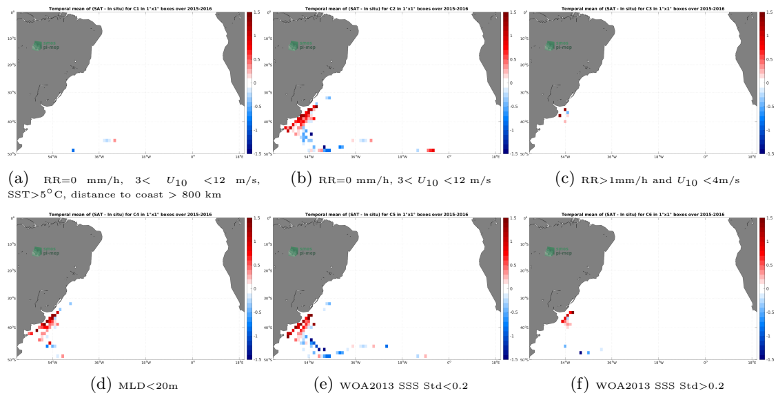
Figure 12: Temporal mean gridded over spatial boxes of size 1^\circ \times 1^\circ of \Delta SSS (SMAP SSS L3 v5.0 - Monthly (JPL) - Marine mammals) for 6 different subdatasets corresponding to:RR=0 mm/h, 3 < U_{10} < 12 m/s, SST > 5^\circ\text{C} , distance to coast > 800 km (a), RR=0 mm/h, 3 < U_{10} < 12 m/s (b), RR > 1 mm/h and U_{10} < 4 m/s (c),MLD < 20 m (d),WOA2013 SSS Std < 0.2 (e),WOA2013 SSS Std > 0.2 (f).
