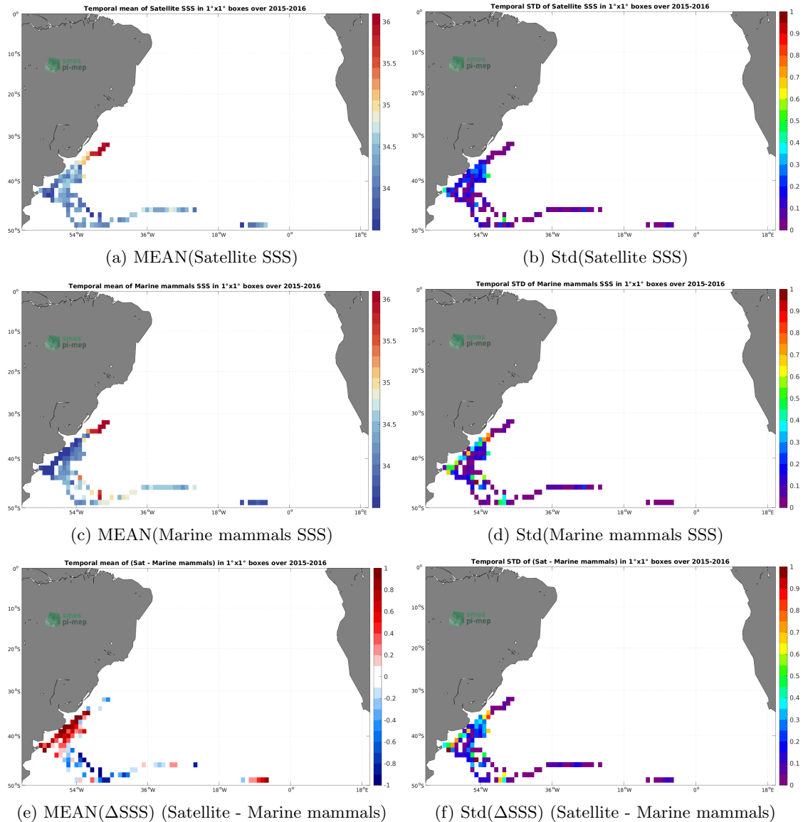
Figure 6: Temporal mean (left) and Std (right) of SSS from SMAP SSS L3 v5.0 - Monthly (JPL) (top), Marine mammals (middle), and of \Delta SSS (Satellite - Marine mammals). Only match-up pairs are used to generate these maps.
