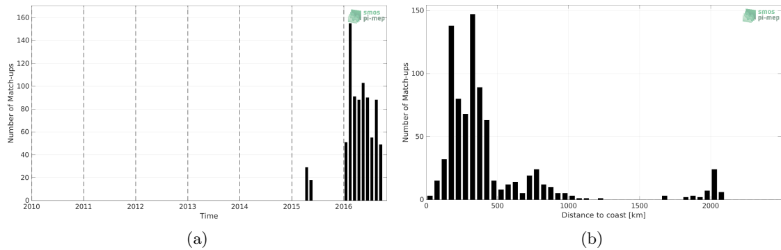
Figure 1: Number of match-ups between Marine mammals and SMAP SSS L3 v5.0 - Monthly (JPL) SSS as a function of time (a) and as function of the distance to coast (b) over the South Atlantic Ocean Pi-MEP region and for the full satellite product period.
