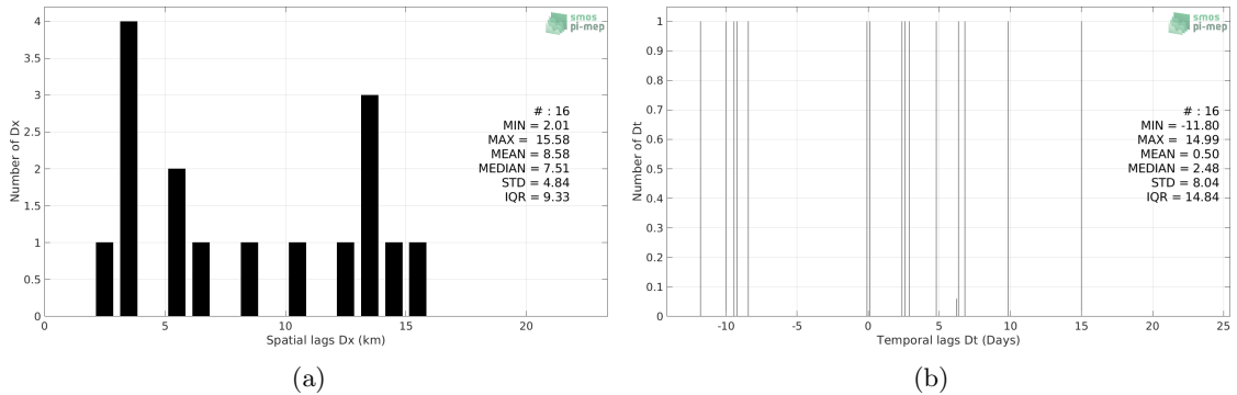
Figure 5: Histograms of the spatial (a) and temporal (b) lags between the location/time of the Sea mammals pixel measurement and the date of the corresponding SMAP SSS L3 v5.0 - Monthly (JPL) SSS pixel.
