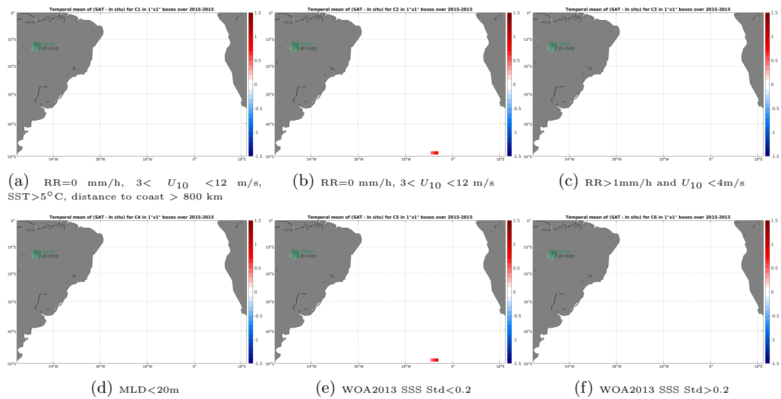
Figure 12: Temporal mean gridded over spatial boxes of size 1^{\circ}\times 1^{\circ} of \Delta\text{SSS} (SMAP SSS L3 v5.0 - Monthly (JPL) - Sea mammals) for 6 different subdatasets corresponding to:RR=0 mm/h, 3 < U_{10} < 12 m/s, SST >5^{\circ}\text{C} , distance to coast > 800 km (a), RR=0 mm/h, 3 < U_{10} < 12 m/s (b), RR >1 mm/h and U_{10} < 4 m/s (c),MLD <20 m (d),WOA2013 SSS Std <0.2 (e),WOA2013 SSS Std >0.2 (f).
