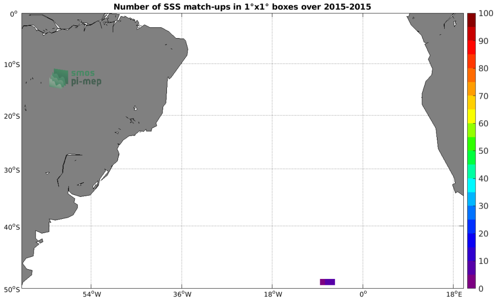
Figure 4: Number of SSS match-ups between Sea mammals SSS and the SMAP SSS L3 v5.0 - Monthly (JPL) SSS product for the South Atlantic Ocean Pi-MEP region over 1^{\circ} \times 1^{\circ} boxes and for the full satellite product period.
