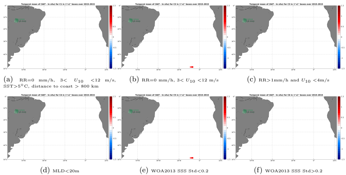
Figure 12: Temporal mean gridded over spatial boxes of size 1^{\circ}\times 1^{\circ} of \Delta\text{SSS} (SMAP SSS L3 v5.0 - Monthly (JPL) - Sea mammals) for 6 different subdatasets corresponding to:RR=0 mm/h, 3 < U_{10} < 12 m/s, SST > 5^{\circ}\text{C} , distance to coast > 800 km (a), RR=0 mm/h, 3 < U_{10} < 12 m/s (b), RR > 1\text{mm/h} and U_{10} < 4\text{m/s} (c),MLD < 20\text{m} (d),WOA2013 SSS Std < 0.2 (e),WOA2013 SSS Std > 0.2 (f).
