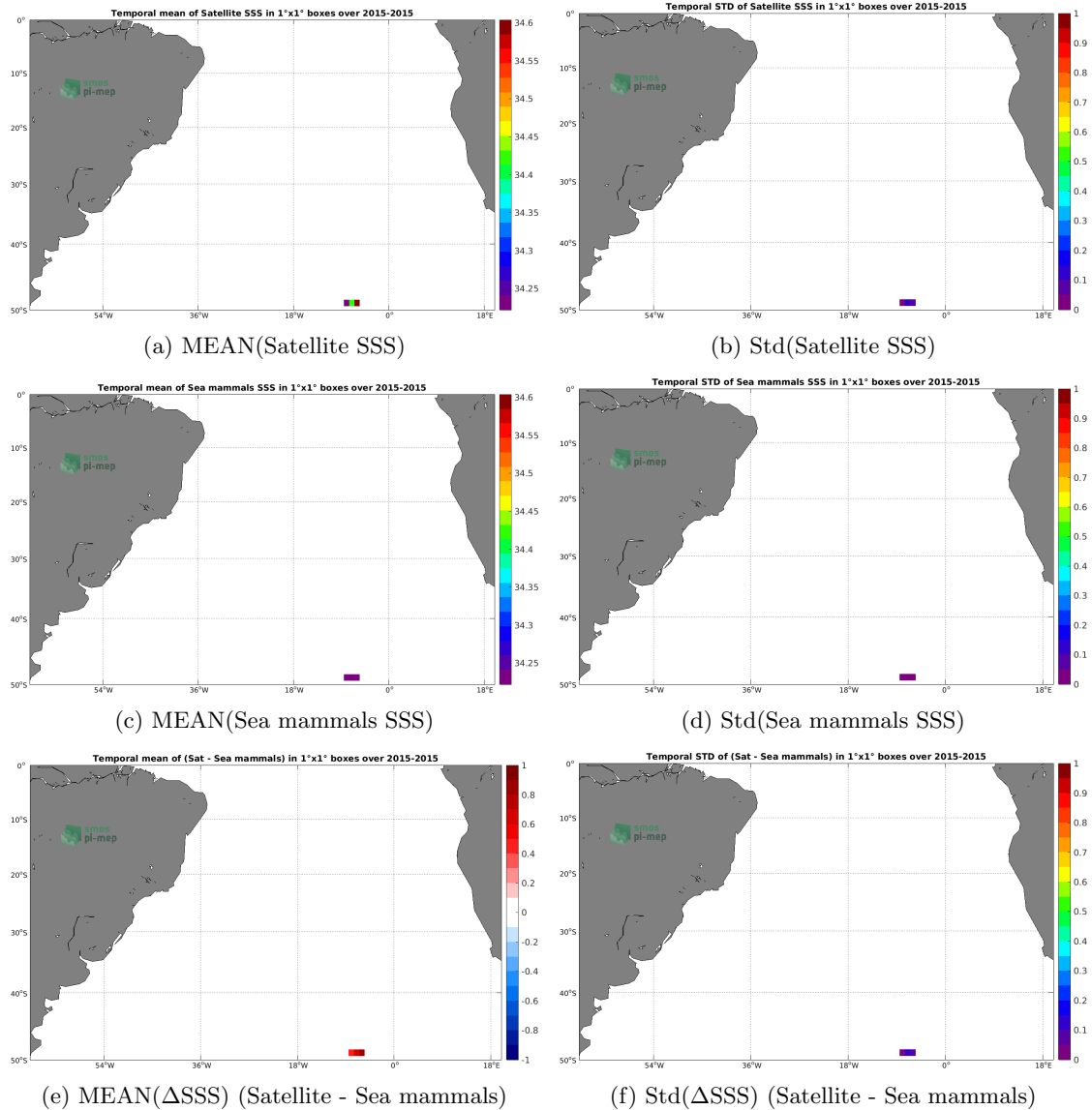
Figure 6: Temporal mean (left) and Std (right) of SSS from SMAP SSS L3 v5.0 - Monthly (JPL) (top), Sea mammals (middle), and of \Delta SSS (Satellite - Sea mammals). Only match-up pairs are used to generate these maps.
