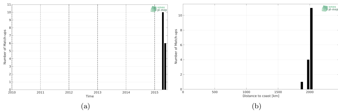
Figure 1: Number of match-ups between Sea mammals and SMAP SSS L3 v5.0 - Monthly (JPL) SSS as a function of time (a) and as function of the distance to coast (b) over the South Atlantic Ocean Pi-MEP region and for the full satellite product period.
