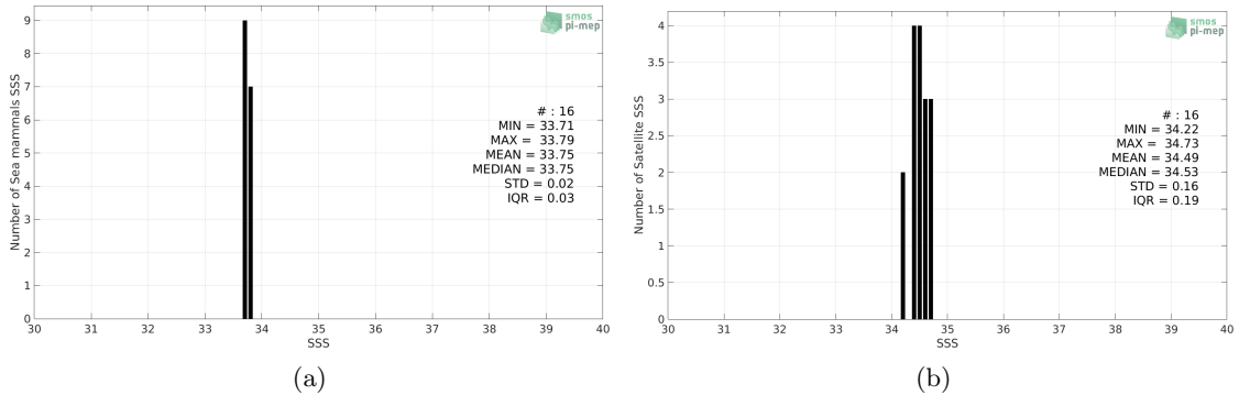
Figure 2: Histograms of SSS from Sea mammals (a) and SMAP SSS L3 v5.0 - Monthly (JPL) (b) considering all match-up pairs per bins of 0.1 over the South Atlantic Ocean Pi-MEP region and for the full satellite product period.
