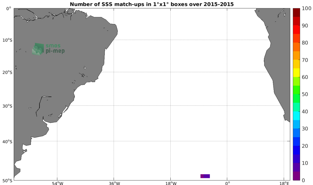
Figure 4: Number of SSS match-ups between Sea mammals SSS and the SMAP SSS L3 v5.0 - Monthly (JPL) SSS product for the South Atlantic Ocean Pi-MEP region over 1°x1° boxes and for the full satellite product period.
