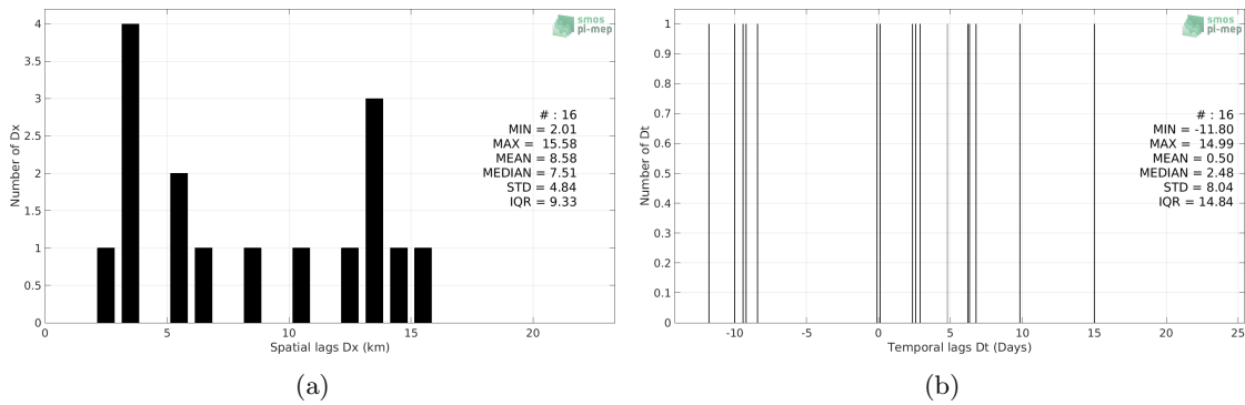
Figure 5: Histograms of the spatial (a) and temporal (b) lags between the time of the Sea mammals measurements and the date of the corresponding SMAP SSS L3 v5.0 - Monthly (JPL) SSS product.
