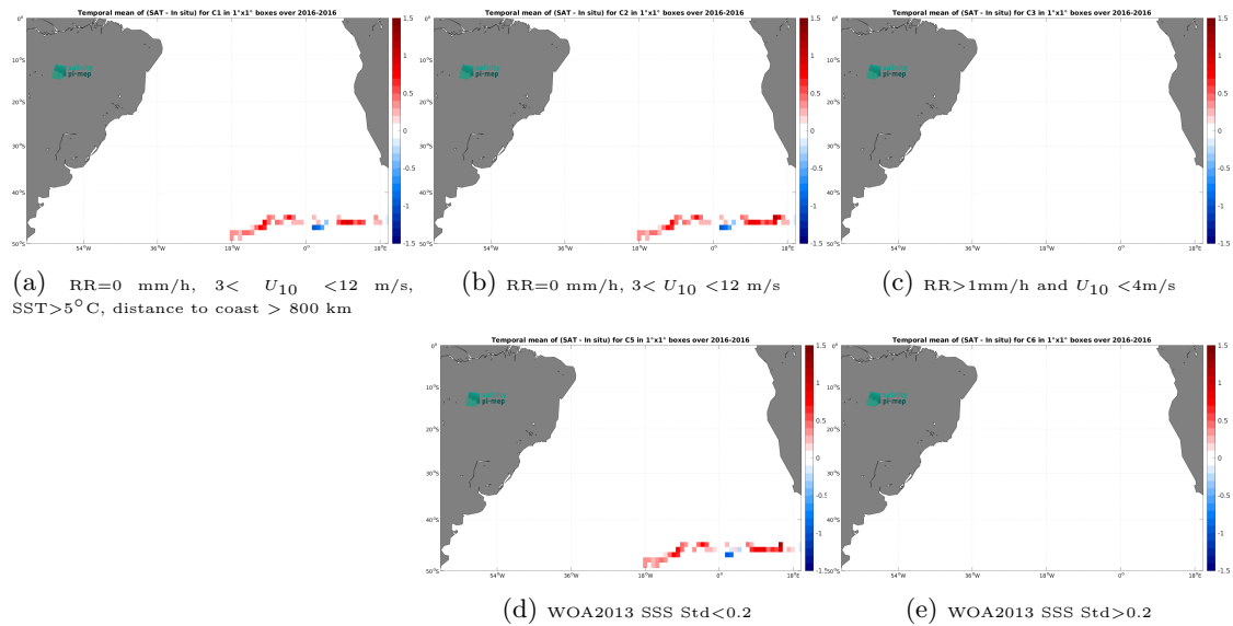
Figure 13: Temporal mean gridded over spatial boxes of size 1^\circ \times 1^\circ of \Delta\text{SSS} (SMAP SSS L3 v5.0 - Monthly (JPL) - Surface drifters) for 5 different subdatasets corresponding to: \text{RR}=0 mm/h, 3 < U_{10} < 12 m/s, \text{SST} > 5^\circ\text{C} , distance to coast > 800 km (a), \text{RR}=0 mm/h, 3 < U_{10} < 12 m/s (b), \text{RR} > 1\text{mm/h} and U_{10} < 4\text{m/s} (c), WOA2013 SSS Std < 0.2 (d), WOA2013 SSS Std > 0.2 (e).
