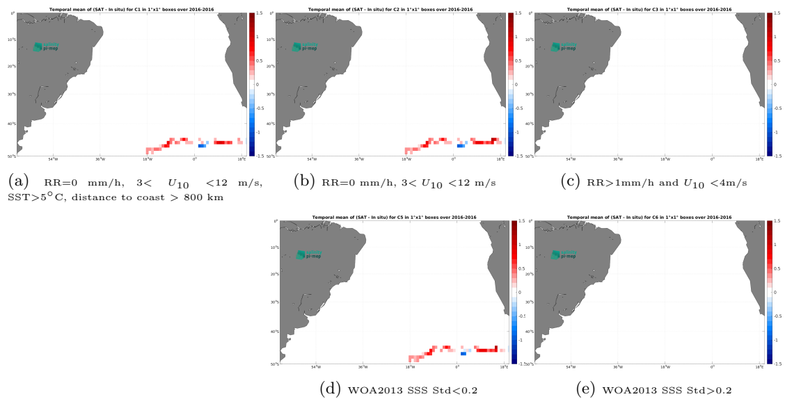
Figure 13: Temporal mean gridded over spatial boxes of size 1^\circ \times 1^\circ of \Delta SSS (SMAP SSS L3 v5.0 - Monthly (JPL) - Surface drifters) for 5 different subdatasets corresponding to:RR=0 mm/h, 3 < U_{10} < 12 m/s, SST >5^\circ\text{C} , distance to coast > 800 km (a), RR=0 mm/h, 3 < U_{10} < 12 m/s (b), RR >1 mm/h and U_{10} < 4 m/s (c), WOA2013 SSS Std <0.2 (d), WOA2013 SSS Std >0.2 (e).
