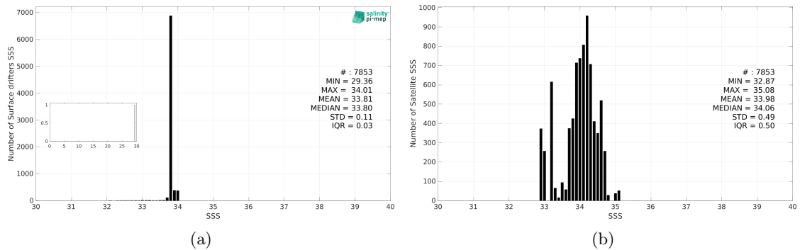
Figure 3: Histograms of SSS from Surface drifters (a) and SMAP SSS L3 v5.0 - Monthly (JPL) (b) considering all match-up pairs per bins of 0.1 over the South Atlantic Ocean Pi-MEP region and for the full satellite product period.
