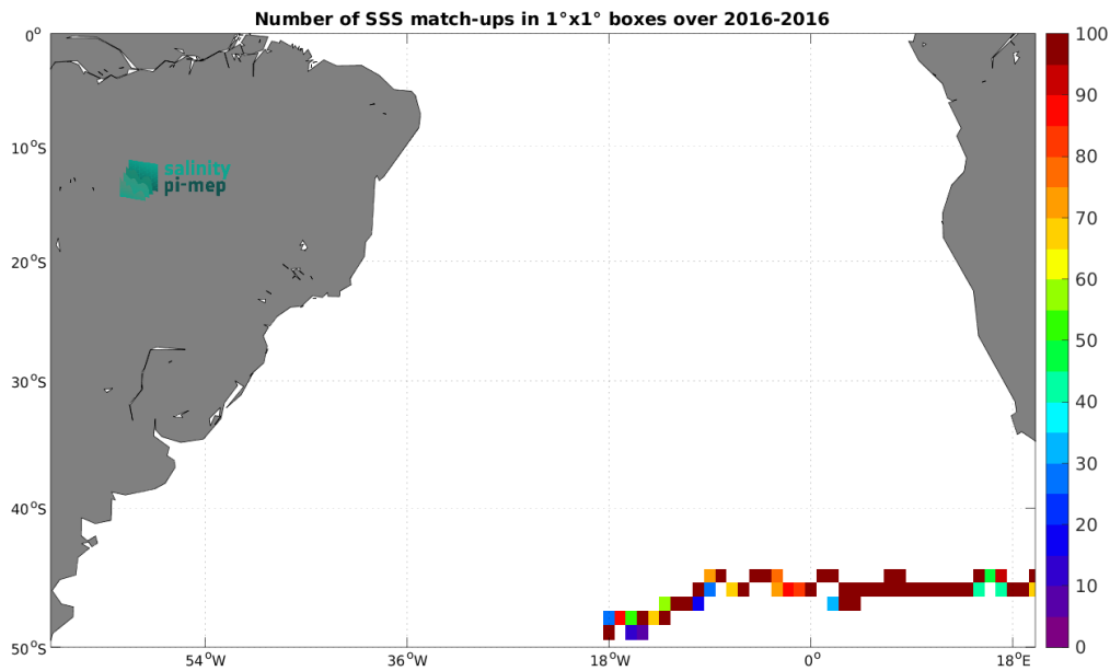
Figure 4: Number of SSS match-ups between Surface drifters SSS and the SMAP SSS L3 v5.0 - Monthly (JPL) SSS product for the South Atlantic Ocean Pi-MEP region over 1^\circ \times 1^\circ boxes and for the full satellite product period.
