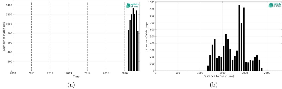
Figure 2: Number of match-ups between Surface drifters and SMAP SSS L3 v5.0 - Monthly (JPL) SSS as a function of time (a) and as function of the distance to coast (b) over the South Atlantic Ocean Pi-MEP region and for the full satellite product period.
