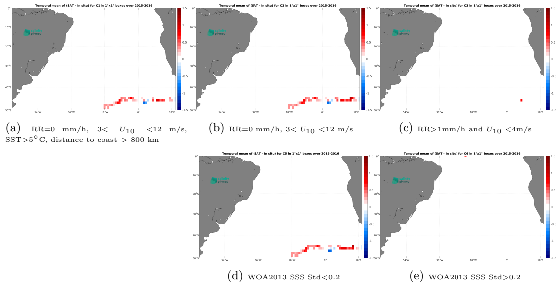
Figure 11: Temporal mean gridded over spatial boxes of size 1^\circ \times 1^\circ of \Delta SSS (SMAP SSS L3 v5.0 - Monthly (JPL) - Surface drifters) for 5 different subdatasets corresponding to:RR=0 mm/h, 3 < U_{10} < 12 m/s, SST >5^\circ\text{C} , distance to coast > 800 km (a), RR=0 mm/h, 3 < U_{10} < 12 m/s (b), RR >1 mm/h and U_{10} < 4 m/s (c), WOA2013 SSS Std <0.2 (d), WOA2013 SSS Std >0.2 (e).
