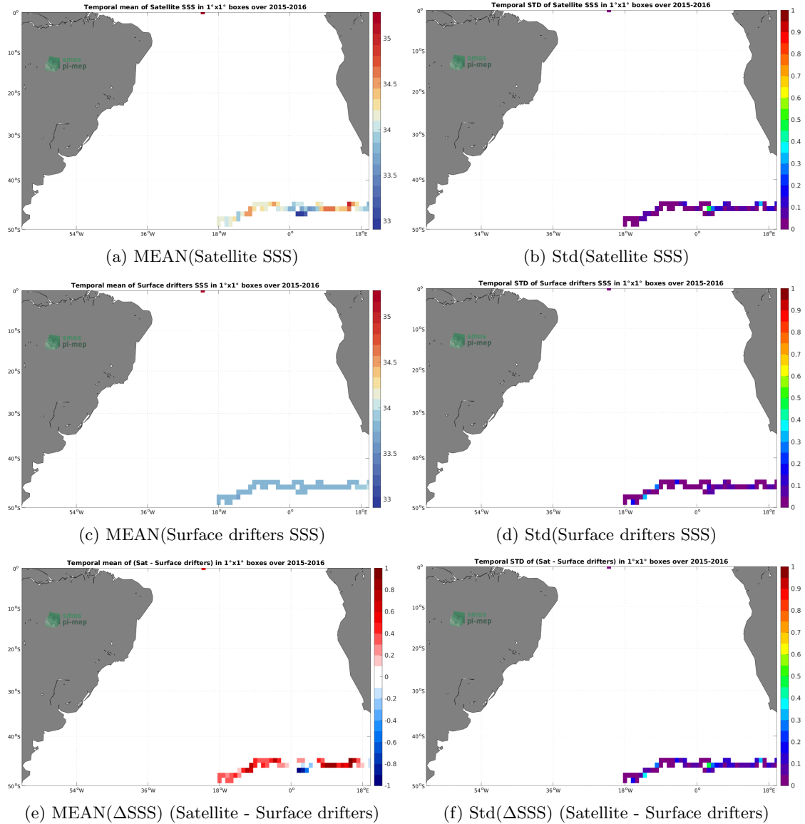
Figure 5: Temporal mean (left) and Std (right) of SSS from SMAP SSS L3 v5.0 - Monthly (JPL) (top), Surface drifters (middle), and of \Delta SSS (Satellite - Surface drifters). Only match-up pairs are used to generate these maps.
