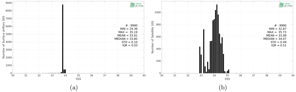
Figure 2: Histograms of SSS from Surface drifters (a) and SMAP SSS L3 v5.0 - Monthly (JPL) (b) considering all match-up pairs per bins of 0.1 over the South Atlantic Ocean Pi-MEP region and for the full satellite product period.
