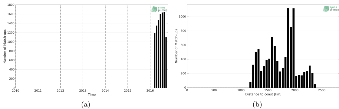
Figure 1: Number of match-ups between Surface drifters and SMAP SSS L3 v5.0 - Monthly (JPL) SSS as a function of time (a) and as function of the distance to coast (b) over the South Atlantic Ocean Pi-MEP region and for the full satellite product period.
