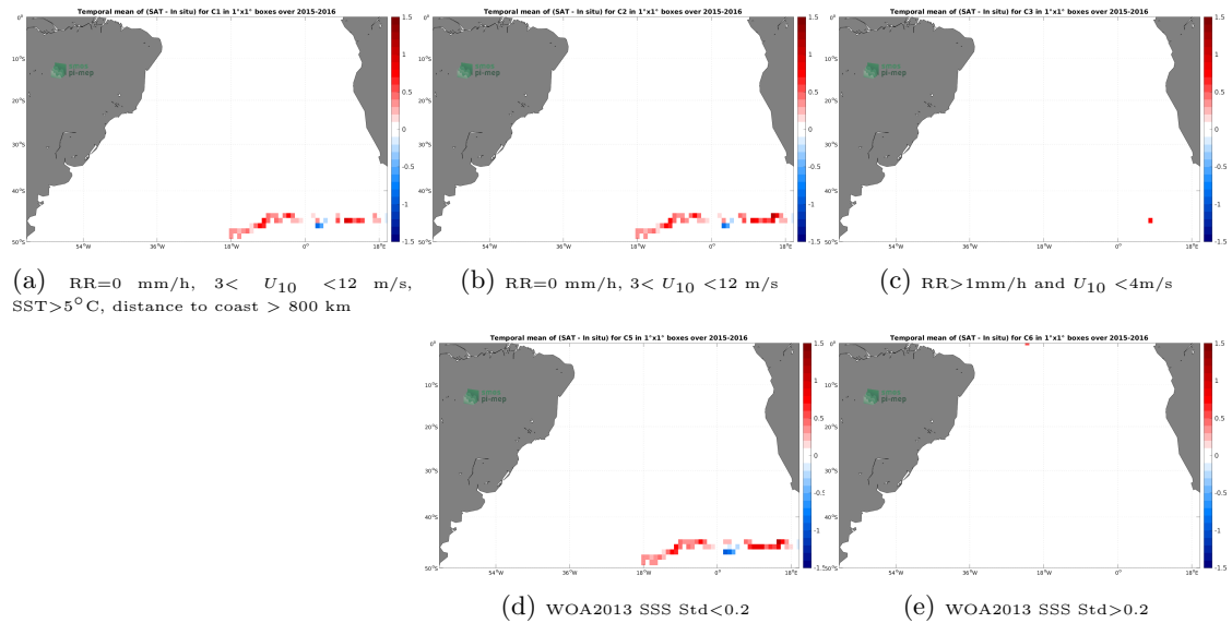
Figure 11: Temporal mean gridded over spatial boxes of size 1^{\circ}\times 1^{\circ} of \Delta\text{SSS} (SMAP SSS L3 v5.0 - Monthly (JPL) - Surface drifters) for 5 different subdatasets corresponding to: \text{RR}=0 mm/h, 3 < U_{10} < 12 m/s, \text{SST} > 5^{\circ}\text{C} , distance to coast > 800 km (a), \text{RR}=0 mm/h, 3 < U_{10} < 12 m/s (b), \text{RR} > 1\text{mm/h} and U_{10} < 4\text{m/s} (c), WOA2013 SSS Std < 0.2 (d), WOA2013 SSS Std > 0.2 (e).
