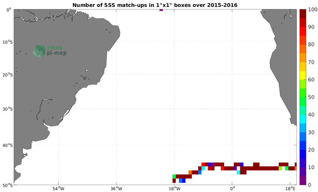
Figure 3: Number of SSS match-ups between Surface drifters SSS and the SMAP SSS L3 v5.0 - Monthly (JPL) SSS product for the South Atlantic Ocean Pi-MEP region over 1^\circ \times 1^\circ boxes and for the full satellite product period.
