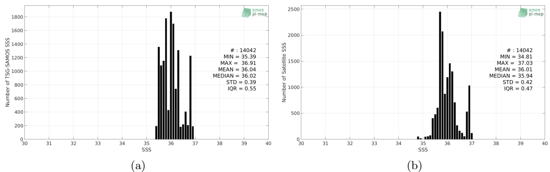
Figure 2: Histograms of SSS from TSG-SAMOS (a) and SMAP-L3-JPL-V4.3-MONTHLY-60KM (b) considering all match-up pairs per bins of 0.1 over the South Atlantic Ocean Pi-MEP region and for the full satellite product period.
