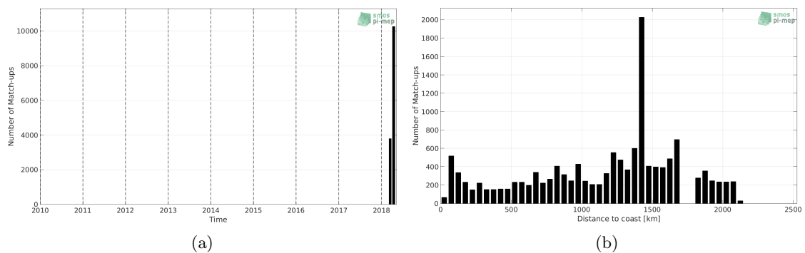
Figure 1: Number of match-ups between TSG-SAMOS and SMAP-L3-JPL-V4.3-MONTHLY-60KM SSS as a function of time (a) and as function of the distance to coast (b) over the South Atlantic Ocean Pi-MEP region and for the full satellite product period.
