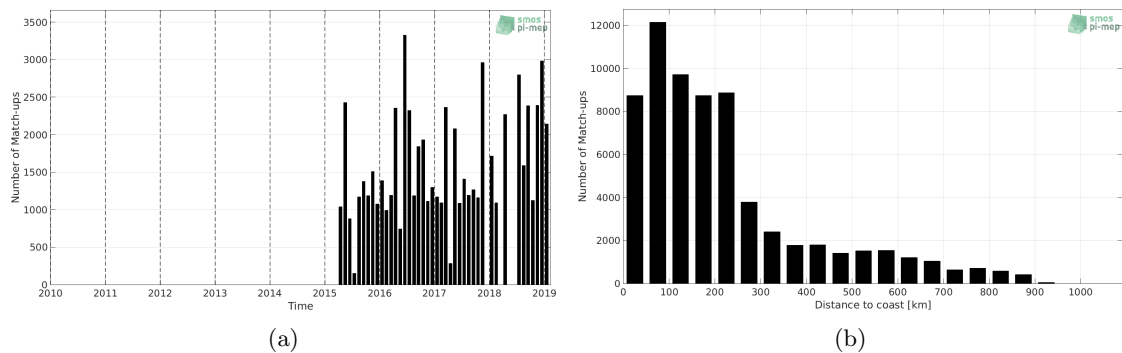
Figure 1: Number of match-ups between TSG-LEGOS-DM and SMAP-L3-JPL-V4.3-MONTHLY-60KM SSS as a function of time (a) and as function of the distance to coast (b) over the South Atlantic Ocean Pi-MEP region and for the full satellite product period.
