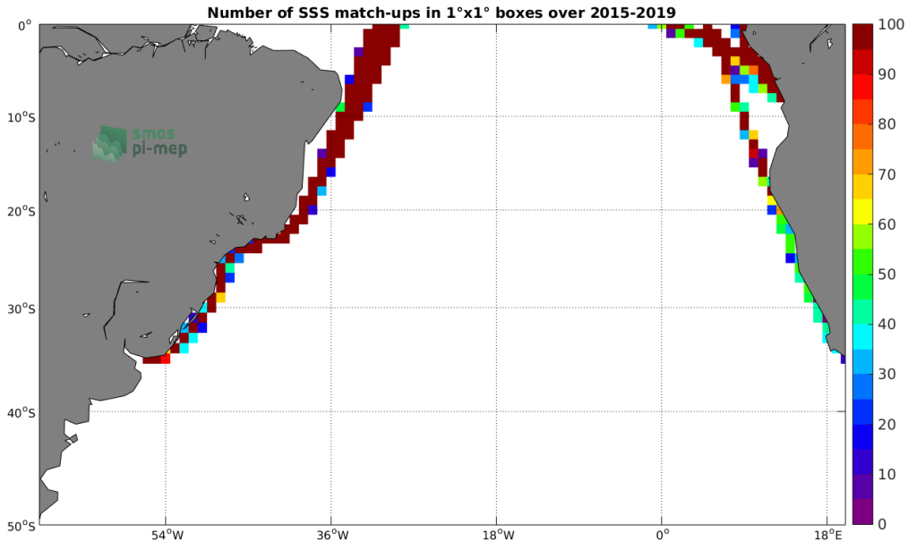
Figure 4: Number of SSS match-ups between TSG-LEGOS-DM SSS and the SMAP-L3-JPL-V4.3-MONTHLY-60KM SSS product for the South Atlantic Ocean Pi-MEP region over 1^\circ \times 1^\circ boxes and for the full satellite product period.
