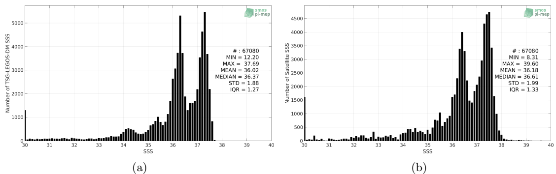
Figure 2: Histograms of SSS from TSG-LEGOS-DM (a) and SMAP-L3-JPL-V4.3-MONTHLY-60KM (b) considering all match-up pairs per bins of 0.1 over the South Atlantic Ocean Pi-MEP region and for the full satellite product period.
