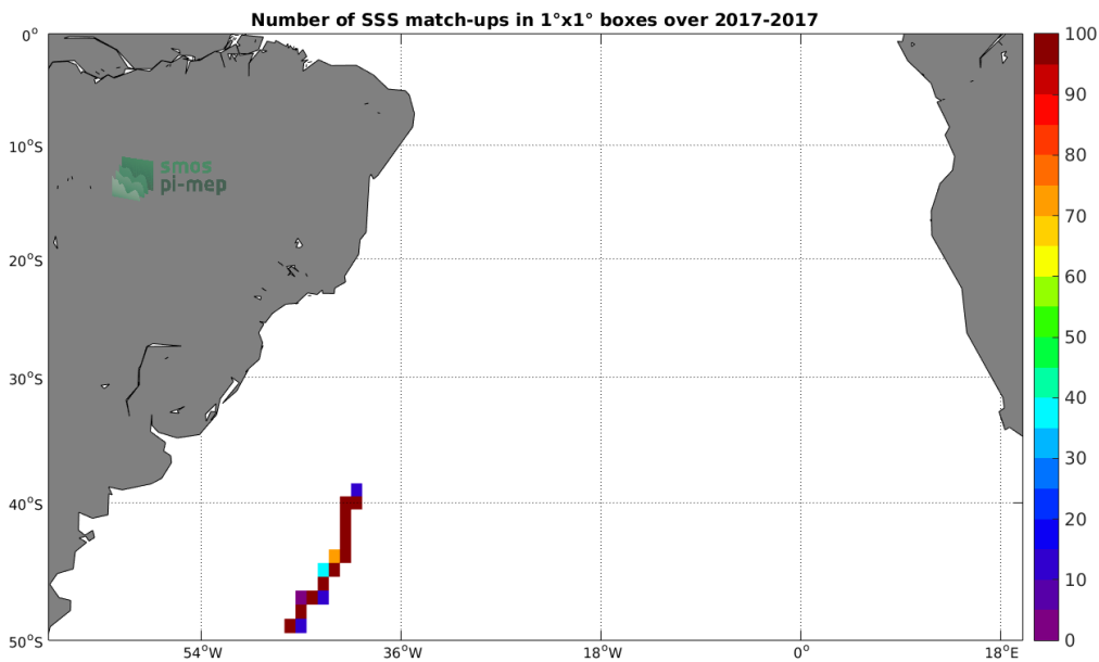
Figure 4: Number of SSS match-ups between TSG-GOSUD-Sailing-ship SSS and the SMAP-L3-JPL-V4.3-MONTHLY-60KM SSS product for the South Atlantic Ocean Pi-MEP region over 1^\circ \times 1^\circ boxes and for the full satellite product period.
