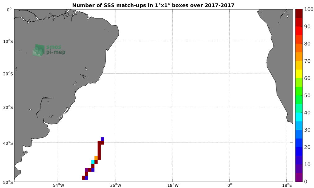
Figure 4: Number of SSS match-ups between TSG-GOSUD-Sailing-ship SSS and the SMAP-L3-JPL-V4.3-MONTHLY-60KM SSS product for the South Atlantic Ocean Pi-MEP region over 1°x1° boxes and for the full satellite product period.
