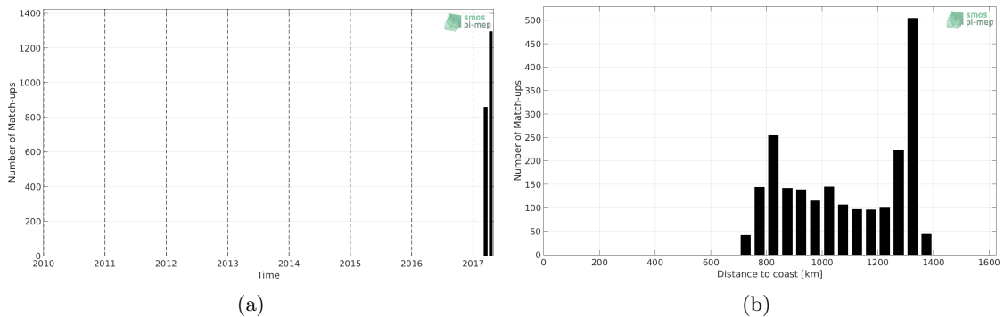
Figure 1: Number of match-ups between TSG-GOSUD-Sailing-ship and SMAP-L3-JPL-V4.3-MONTHLY-60KM SSS as a function of time (a) and as function of the distance to coast (b) over the South Atlantic Ocean Pi-MEP region and for the full satellite product period.
