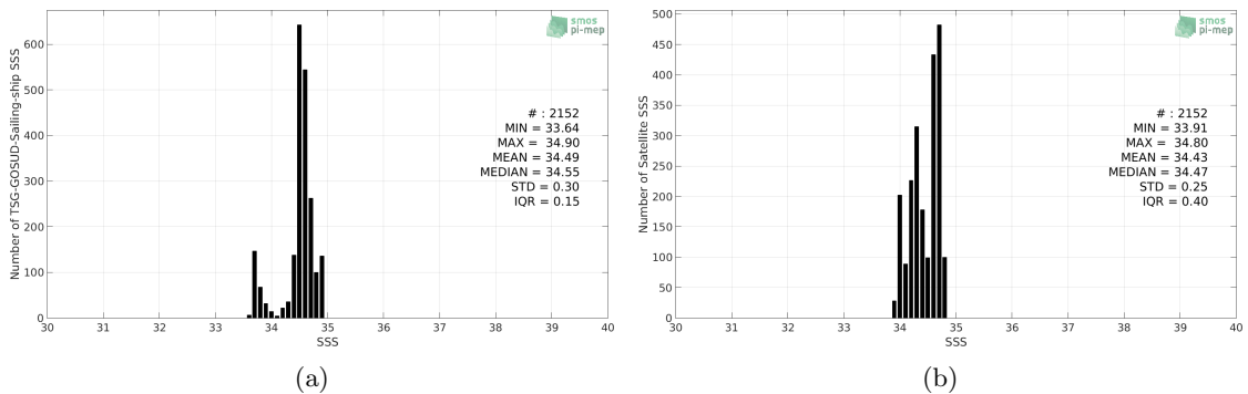
Figure 2: Histograms of SSS from TSG-GOSUD-Sailing-ship (a) and SMAP-L3-JPL-V4.3-MONTHLY-60KM (b) considering all match-up pairs per bins of 0.1 over the South Atlantic Ocean Pi-MEP region and for the full satellite product period.
