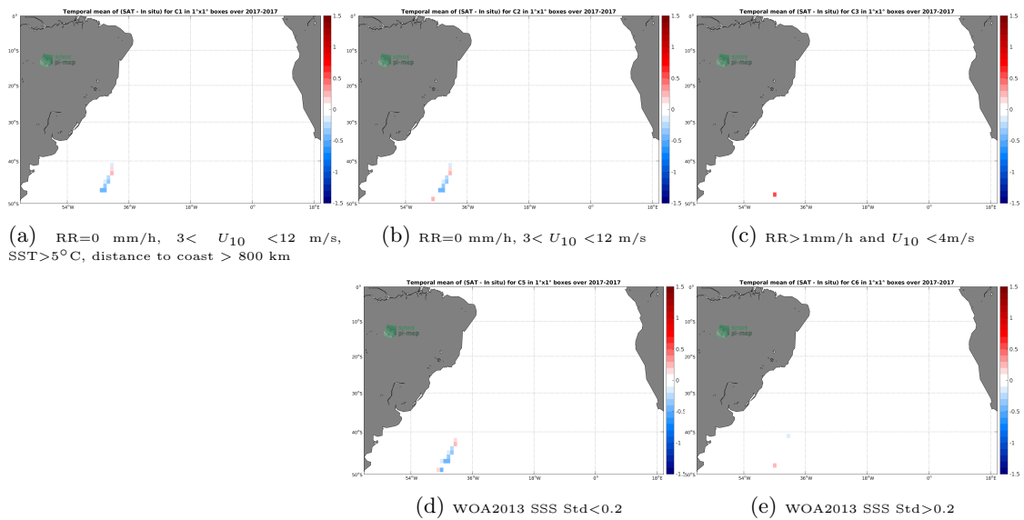
Figure 12: Temporal mean gridded over spatial boxes of size 1^\circ \times 1^\circ of \Delta SSS (SMAP-L3-JPL-V4.3-MONTHLY-60KM - TSG-GOSUD-Sailing-ship) for 5 different subdatasets corresponding to:RR=0 mm/h, 3 < U_{10} < 12 m/s, SST>5°C, distance to coast > 800 km (a), RR=0 mm/h, 3 < U_{10} < 12 m/s (b), RR>1mm/h and U_{10} < 4 m/s (c), WOA2013 SSS Std<0.2 (d), WOA2013 SSS Std>0.2 (e).
