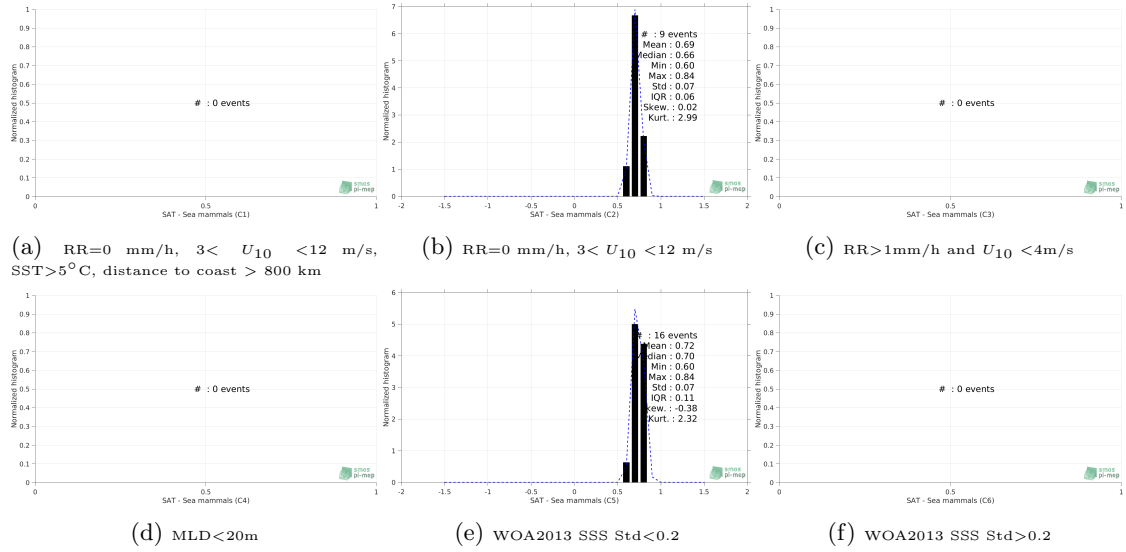
Figure 13: Normalized histogram of \Delta\text{SSS} (SMAP-L3-JPL-V4.3-MONTHLY-60KM - Sea mammals) for 6 different subdatasets corresponding to: RR=0 mm/h, 3 < U_{10} < 12 m/s, SST > 5^\circ\text{C} , distance to coast > 800 km (a), RR=0 mm/h, 3 < U_{10} < 12 m/s (b), RR > 1\text{mm/h} and U_{10} < 4\text{m/s} (c), MLD < 20\text{m} (d), WOA2013 SSS Std < 0.2 (e), WOA2013 SSS Std > 0.2 (f).
