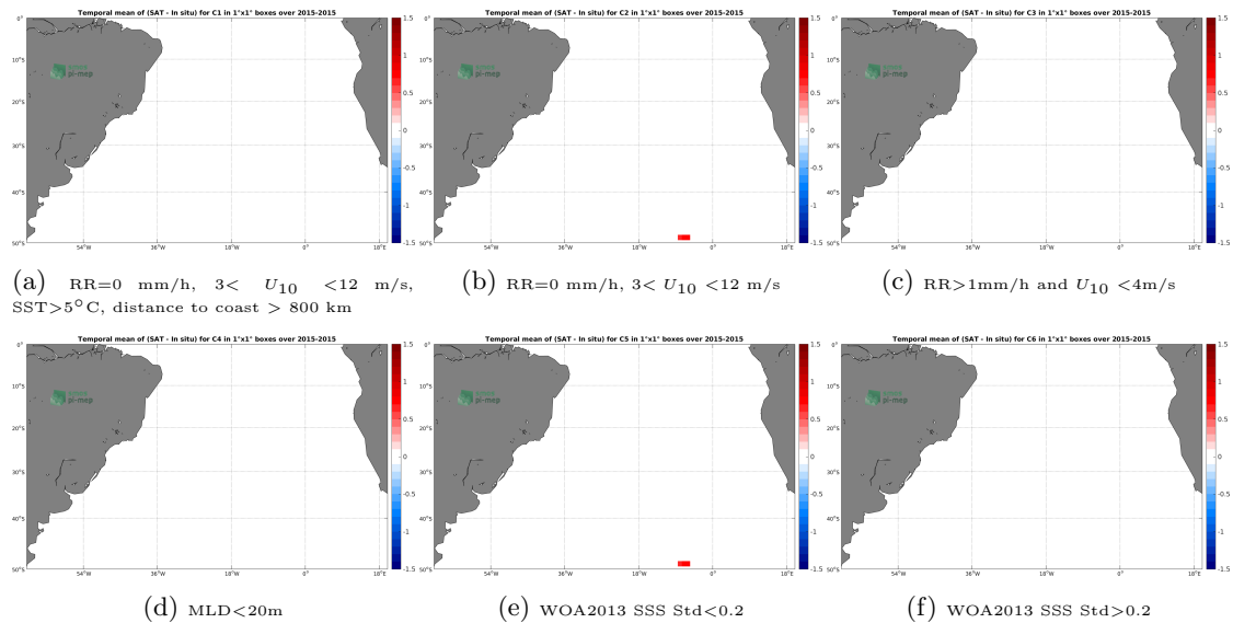
Figure 12: Temporal mean gridded over spatial boxes of size 1^{\circ}\times 1^{\circ} of \Delta\text{SSS} (SMAP-L3-JPL-V4.3-MONTHLY-60KM - Sea mammals) for 6 different subdatasets corresponding to:RR=0 mm/h, 3 < U_{10} < 12 m/s, SST >5^{\circ}\text{C} , distance to coast > 800 km (a), RR=0 mm/h, 3 < U_{10} < 12 m/s (b), RR >1 mm/h and U_{10} < 4 m/s (c),MLD <20 m (d),WOA2013 SSS Std <0.2 (e),WOA2013 SSS Std >0.2 (f).
