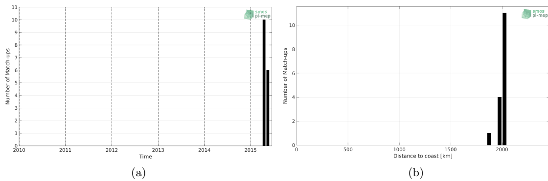
Figure 1: Number of match-ups between Sea mammals and SMAP-L3-JPL-V4.3-MONTHLY-60KM SSS as a function of time (a) and as function of the distance to coast (b) over the South Atlantic Ocean Pi-MEP region and for the full satellite product period.
