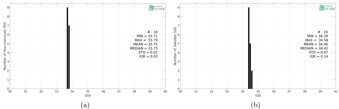
Figure 2: Histograms of SSS from Sea mammals (a) and SMAP-L3-JPL-V4.3-MONTHLY-60KM (b) considering all match-up pairs per bins of 0.1 over the South Atlantic Ocean Pi-MEP region and for the full satellite product period.
