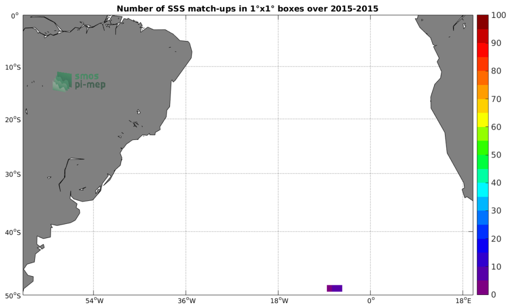
Figure 4: Number of SSS match-ups between Sea mammals SSS and the SMAP-L3-JPL-V4.3-MONTHLY-60KM SSS product for the South Atlantic Ocean Pi-MEP region over 1^\circ \times 1^\circ boxes and for the full satellite product period.
