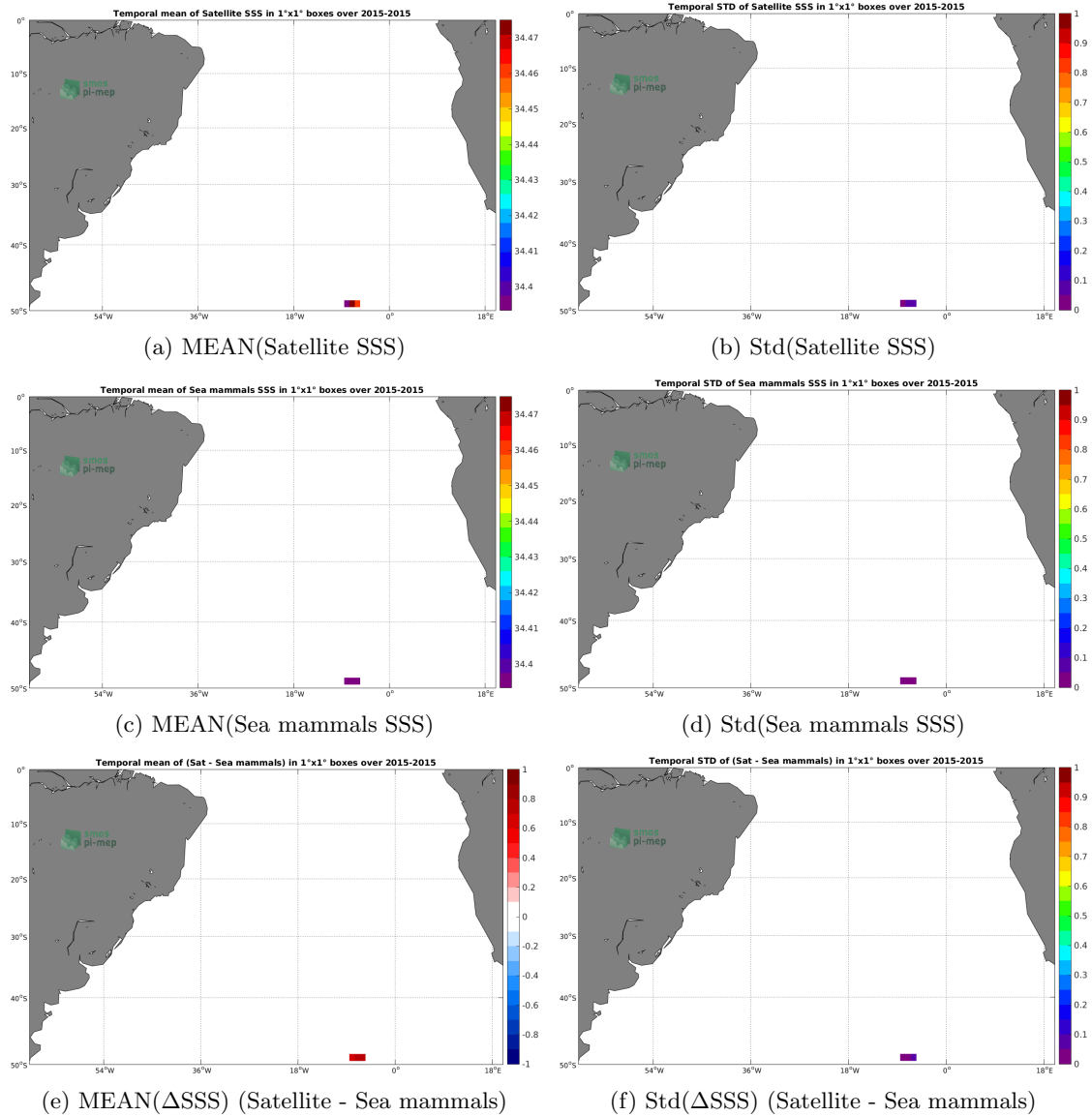
Figure 6: Temporal mean (left) and Std (right) of SSS from SMAP-L3-JPL-V4.3-MONTHLY-60KM (top), Sea mammals (middle), and of \Delta SSS (Satellite - Sea mammals). Only match-up pairs are used to generate these maps.
