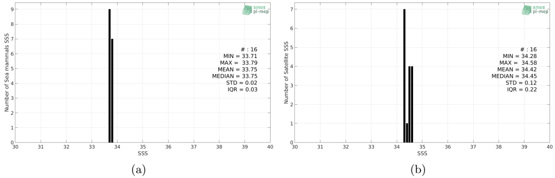
Figure 2: Histograms of SSS from Sea mammals (a) and SMAP-L3-JPL-V4.2-MONTHLY-60KM (b) considering all match-up pairs per bins of 0.1 over the South Atlantic Ocean Pi-MEP region and for the full satellite product period.
