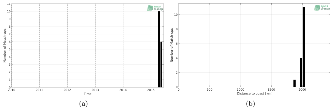
Figure 1: Number of match-ups between Sea mammals and SMAP-L3-JPL-V4.2-MONTHLY-60KM SSS as a function of time (a) and as function of the distance to coast (b) over the South Atlantic Ocean Pi-MEP region and for the full satellite product period.
