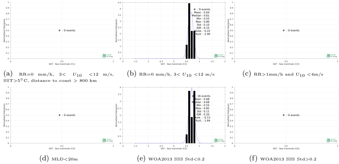
Figure 13: Normalized histogram of \Delta SSS (SMAP-L3-JPL-V4.2-MONTHLY-60KM - Sea mammals) for 6 different subdatasets corresponding to: RR=0 mm/h, 3 < U_{10} < 12 m/s, SST>5°C, distance to coast > 800 km (a), RR=0 mm/h, 3 < U_{10} < 12 m/s (b), RR>1mm/h and U_{10} < 4 m/s (c), MLD<20m (d), WOA2013 SSS Std<0.2 (e), WOA2013 SSS Std>0.2 (f).
