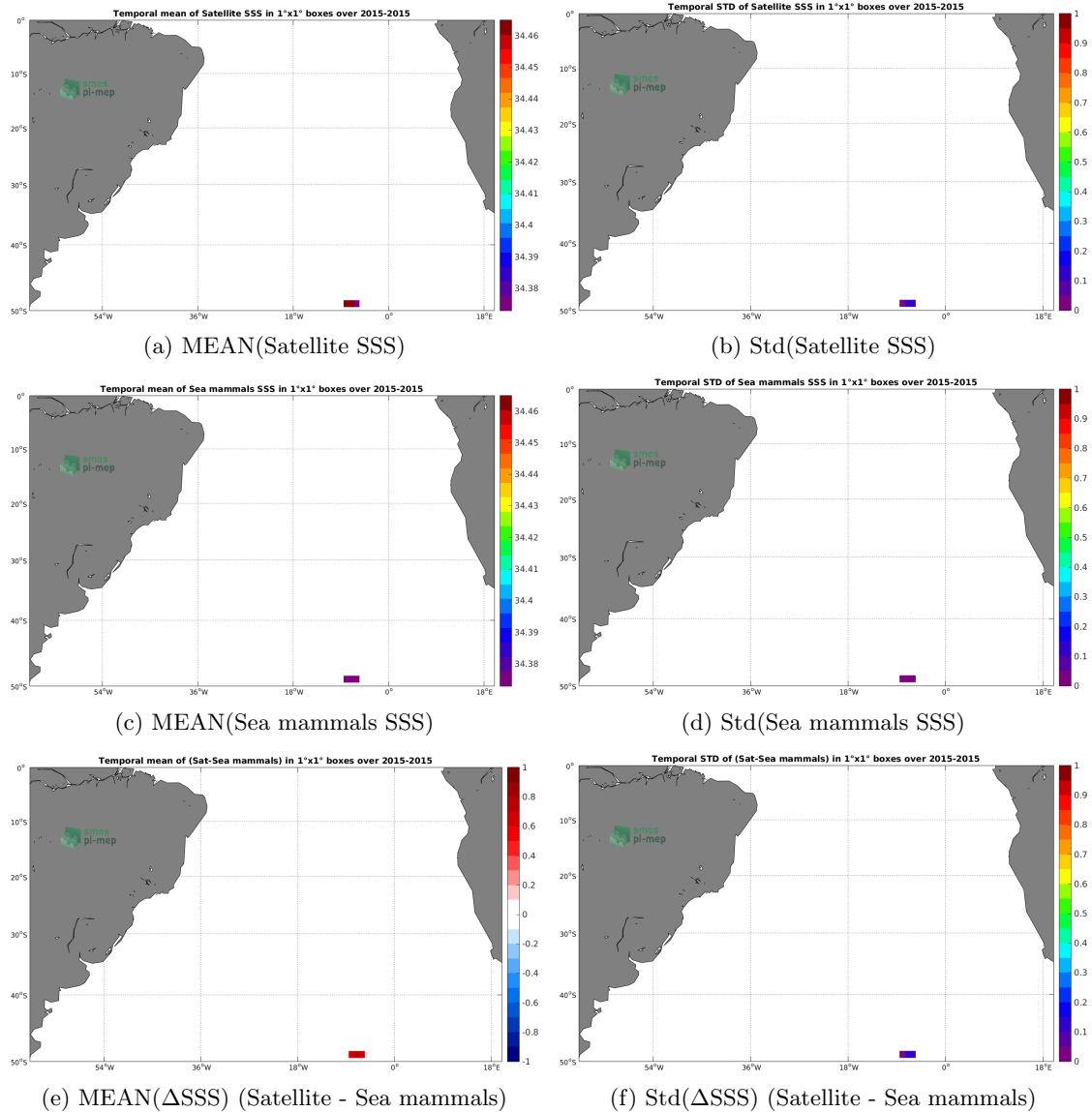
Figure 6: Temporal mean (left) and Std (right) of SSS from SMAP-L3-JPL-V4.2-MONTHLY-60KM (top), Sea mammals (middle), and of \Delta SSS (Satellite - Sea mammals). Only match-up pairs are used to generate these maps.
