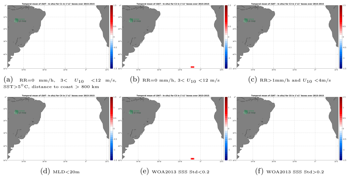
Figure 12: Temporal mean gridded over spatial boxes of size 1^\circ \times 1^\circ of \Delta SSS (SMAP-L3-JPL-V4.2-MONTHLY-60KM - Sea mammals) for 6 different subdatasets corresponding to:RR=0 mm/h, 3 < U_{10} < 12 m/s, SST >5^\circ C, distance to coast > 800 km (a), RR=0 mm/h, 3 < U_{10} < 12 m/s (b), RR >1 mm/h and U_{10} < 4 m/s (c),MLD <20 m (d),WOA2013 SSS Std <0.2 (e),WOA2013 SSS Std >0.2 (f).
