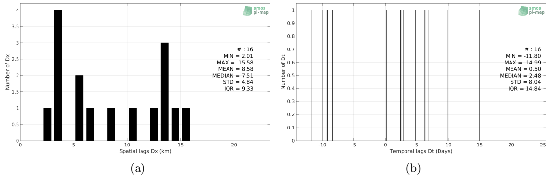
Figure 5: Histograms of the spatial (a) and temporal (b) lags between the time of the Sea mammals measurements and the date of the corresponding SMAP-L3-JPL-V4.2-MONTHLY-60KM SSS product.
