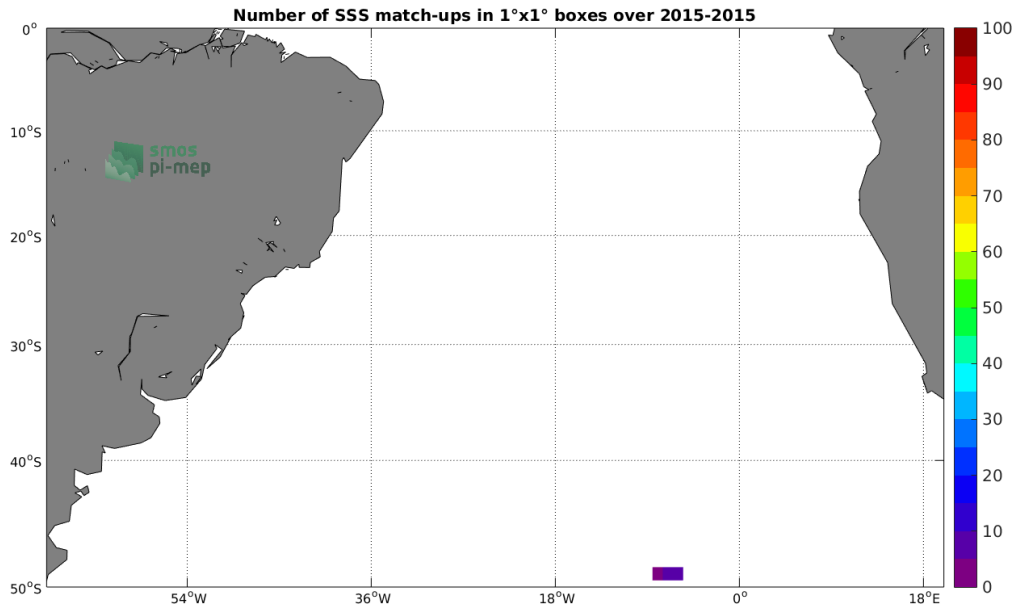
Figure 4: Number of SSS match-ups between Sea mammals SSS and the SMAP-L3-JPL-V4.2-MONTHLY-60KM SSS product for the South Atlantic Ocean Pi-MEP region over 1°x1° boxes and for the full satellite product period.
