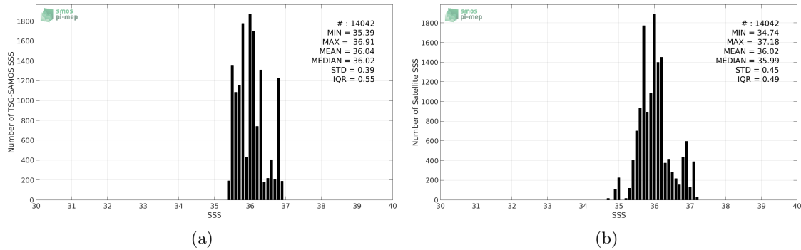
Figure 2: Histograms of SSS from TSG-SAMOS (a) and SMAP-L3-JPL-V4-8DAY-RUNNING-60KM (b) considering all match-up pairs per bins of 0.1 over the South Atlantic Ocean Pi-MEP region and for the full satellite product period.
