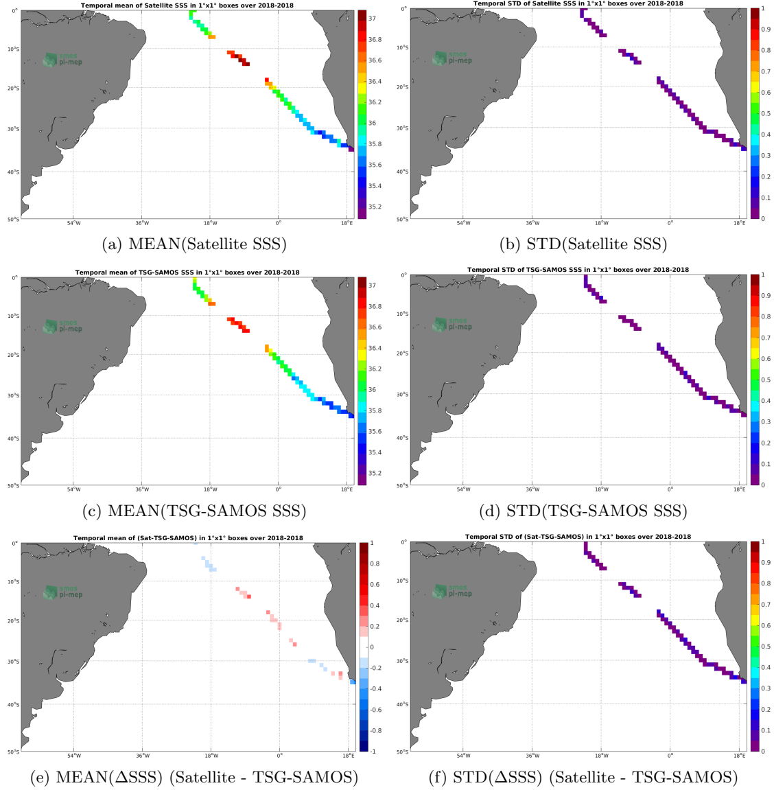
Figure 6: Temporal mean (left) and STD (right) of SSS from SMAP-L3-JPL-V4-8DAY-RUNNING-60KM (top), TSG-SAMOS (middle), and of \Delta SSS (Satellite - TSG-SAMOS). Only match-up pairs are used to generate these maps.
