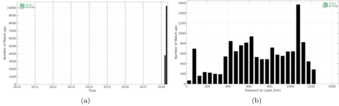
Figure 1: Number of match-ups between TSG-SAMOS and SMAP-L3-JPL-V4-8DAY-RUNNING-60KM SSS as a function of time (a) and as function of the distance to coast (b) over the South Atlantic Ocean Pi-MEP region and for the full satellite product period.
