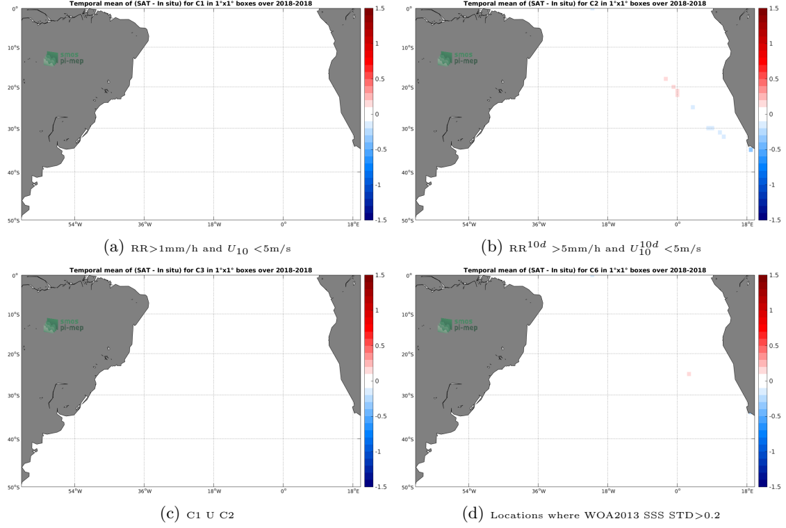
Figure 12: Temporal mean gridded over spatial boxes of size 1^\circ \times 1^\circ of \Delta SSS (SMAP-L3-JPL-V4-8DAY-RUNNING-60KM - TSG-SAMOS) for 4 different subdatasets corresponding to: RR > 1mm/h and U_{10} < 5\text{m/s} (a), RR^{10d} > 5\text{mm/h} and U_{10}^{10d} < 5\text{m/s} (b), C1 U C2 (c), Locations where WOA2013 SSS STD > 0.2 (d).
