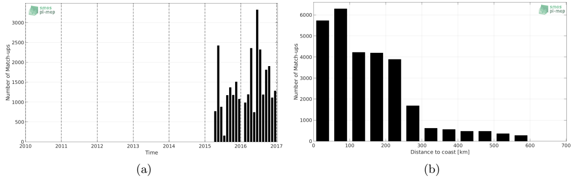
Figure 1: Number of match-ups between TSG-LEGOS-DM and SMAP-L3-JPL-V4-8DAY-RUNNING-60KM SSS as a function of time (a) and as function of the distance to coast (b) over the South Atlantic Ocean Pi-MEP region and for the full satellite product period.
