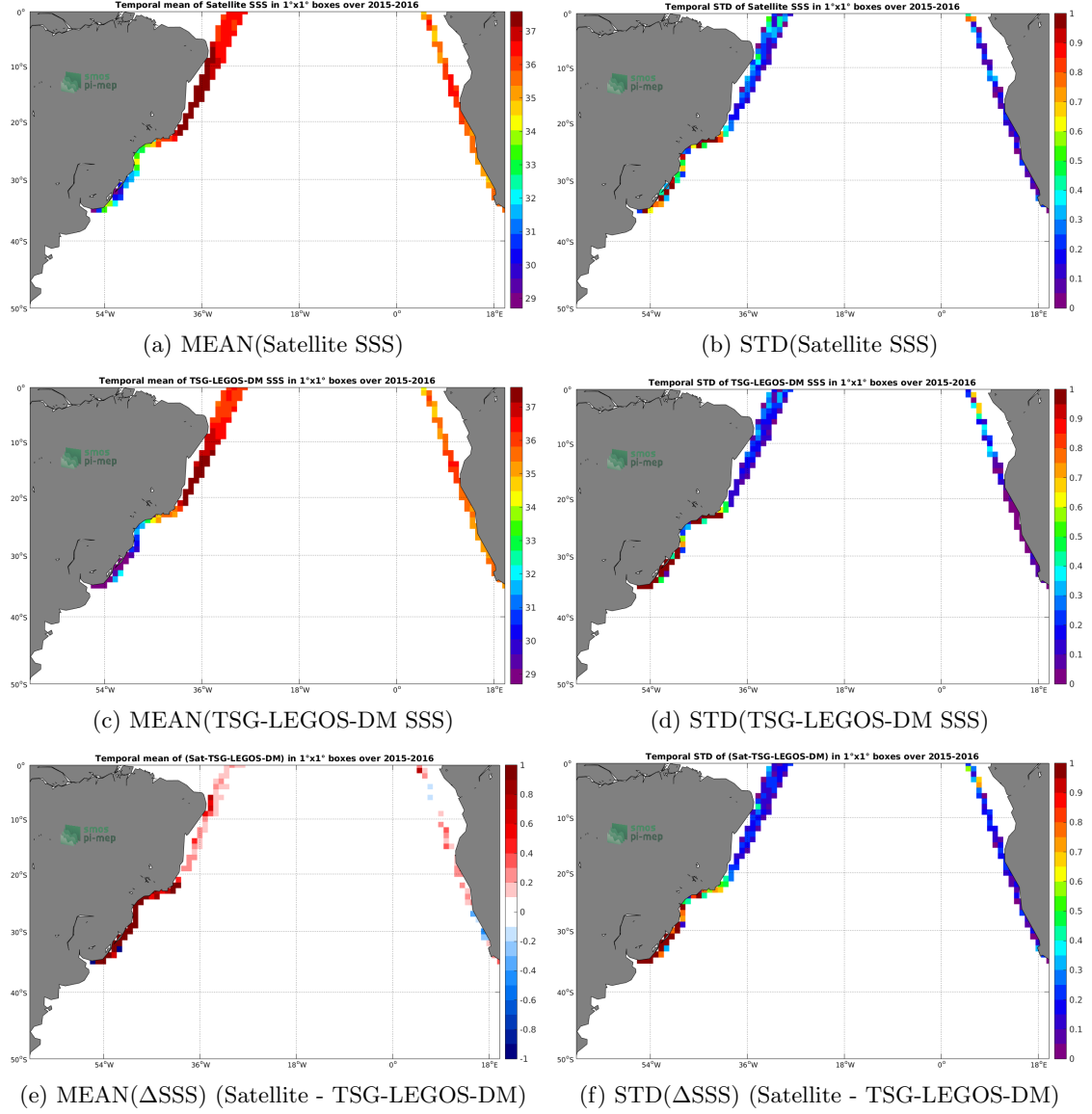
Figure 6: Temporal mean (left) and STD (right) of SSS from SMAP-L3-JPL-V4-8DAY-RUNNING-60KM (top), TSG-LEGOS-DM (middle), and of \Delta SSS (Satellite - TSG-LEGOS-DM). Only match-up pairs are used to generate these maps.
