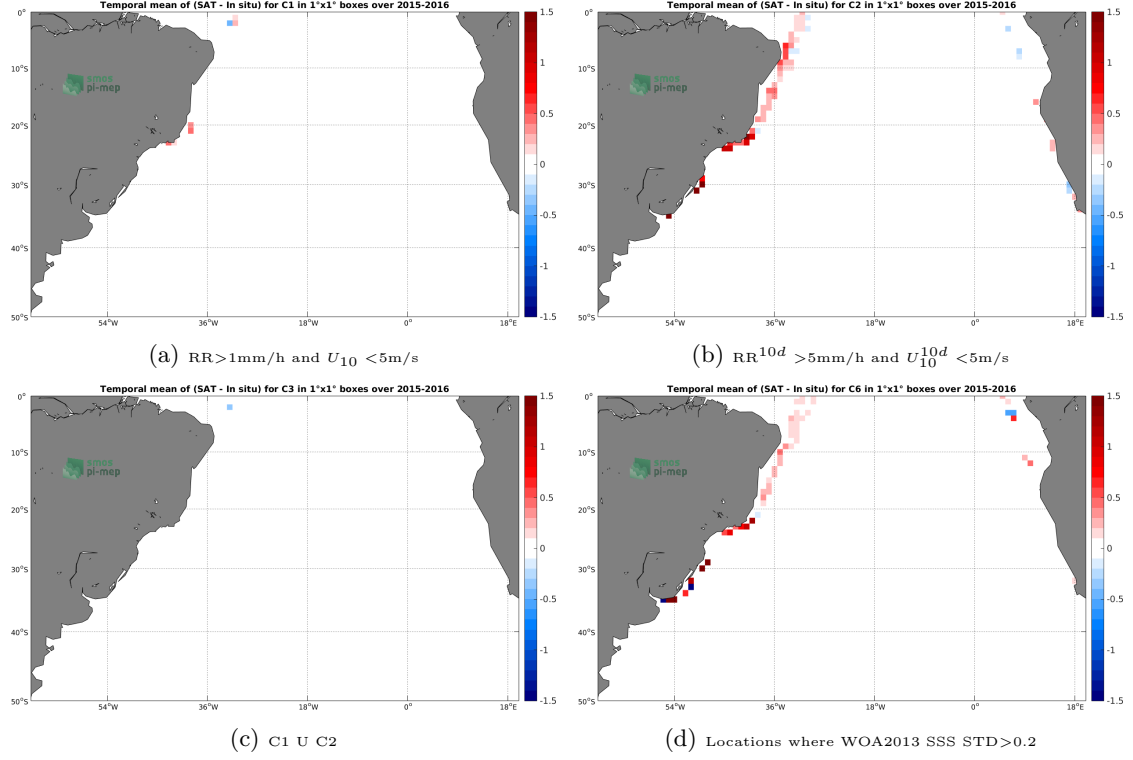
Figure 12: Temporal mean gridded over spatial boxes of size 1^\circ \times 1^\circ of \Delta SSS (SMAP-L3-JPL-V4-8DAY-RUNNING-60KM - TSG-LEGOS-DM) for 4 different subdatasets corresponding to: RR > 1mm/h and U_{10} < 5\text{m/s} (a), RR^{10d} > 5\text{mm/h} and U_{10}^{10d} < 5\text{m/s} (b), C1 U C2 (c), Locations where WOA2013 SSS STD > 0.2 (d).
