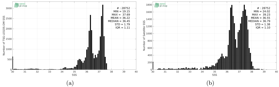
Figure 2: Histograms of SSS from TSG-LEGOS-DM (a) and SMAP-L3-JPL-V4-8DAY-RUNNING-60KM (b) considering all match-up pairs per bins of 0.1 over the South Atlantic Ocean Pi-MEP region and for the full satellite product period.
