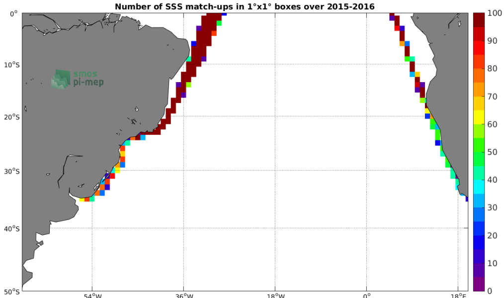
Figure 4: Number of SSS match-ups between TSG-LEGOS-DM SSS and the SMAP-L3-JPL-V4-8DAY-RUNNING-60KM SSS product for the South Atlantic Ocean Pi-MEP region over 1^\circ \times 1^\circ boxes and for the full satellite product period.
