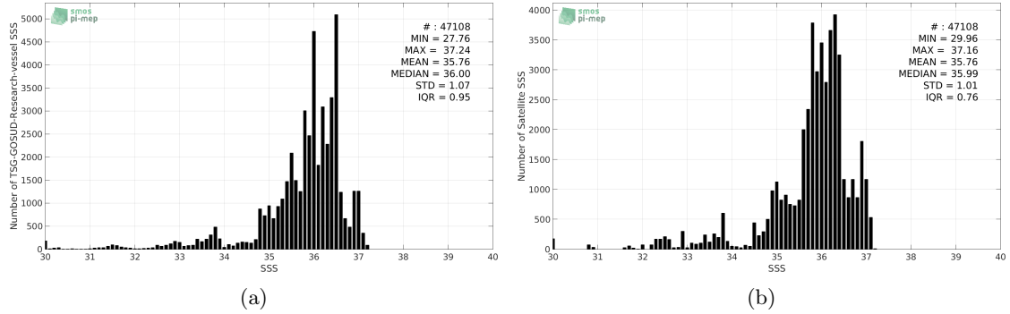
Figure 2: Histograms of SSS from TSG-GOSUD-Research-vessel (a) and SMAP-L3-JPL-V4-8DAY-RUNNING-60KM (b) considering all match-up pairs per bins of 0.1 over the South Atlantic Ocean Pi-MEP region and for the full satellite product period.
