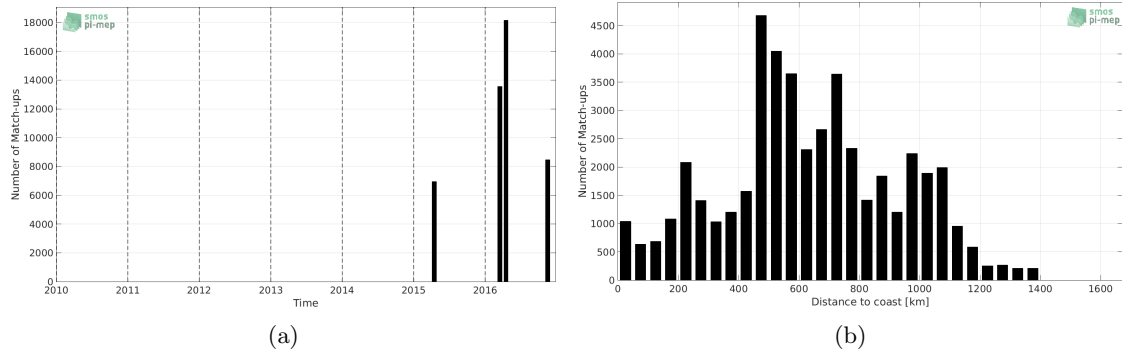
Figure 1: Number of match-ups between TSG-GOSUD-Research-vessel and SMAP-L3-JPL-V4-8DAY-RUNNING-60KM SSS as a function of time (a) and as function of the distance to coast (b) over the South Atlantic Ocean Pi-MEP region and for the full satellite product period.
