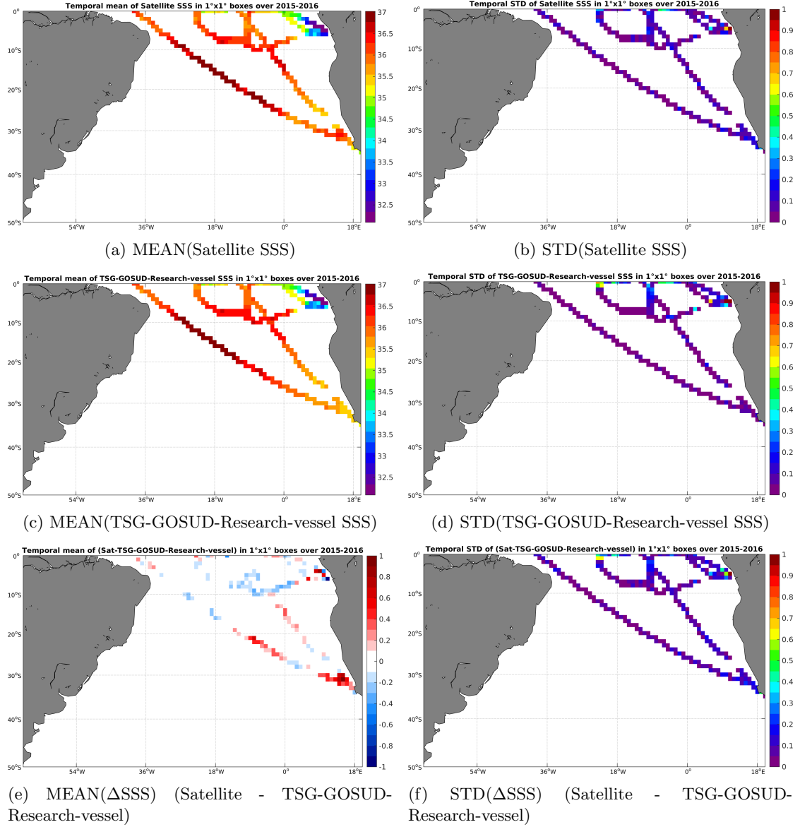
Figure 6: Temporal mean (left) and STD (right) of SSS from SMAP-L3-JPL-V4-8DAY-RUNNING-60KM (top), TSG-GOSUD-Research-vessel (middle), and of \Delta SSS (Satellite - TSG-GOSUD-Research-vessel). Only match-up pairs are used to generate these maps.
