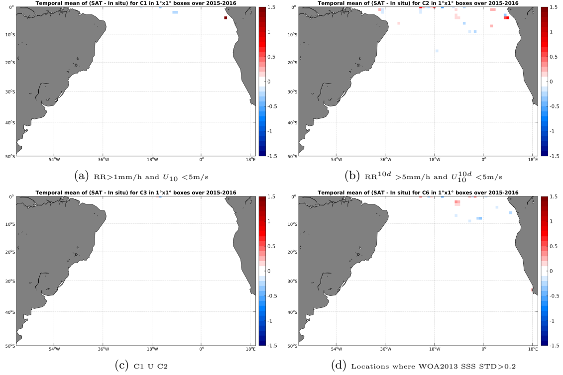
Figure 12: Temporal mean gridded over spatial boxes of size 1^\circ \times 1^\circ of \Delta SSS (SMAP-L3-JPL-V4-8DAY-RUNNING-60KM - TSG-GOSUD-Research-vessel) for 4 different subdatasets corresponding to: RR > 1\text{mm/h} and U_{10} < 5\text{m/s} (a), RR^{10d} > 5\text{mm/h} and U_{10}^{10d} < 5\text{m/s} (b), C1 U C2 (c), Locations where WOA2013 SSS STD > 0.2 (d).
