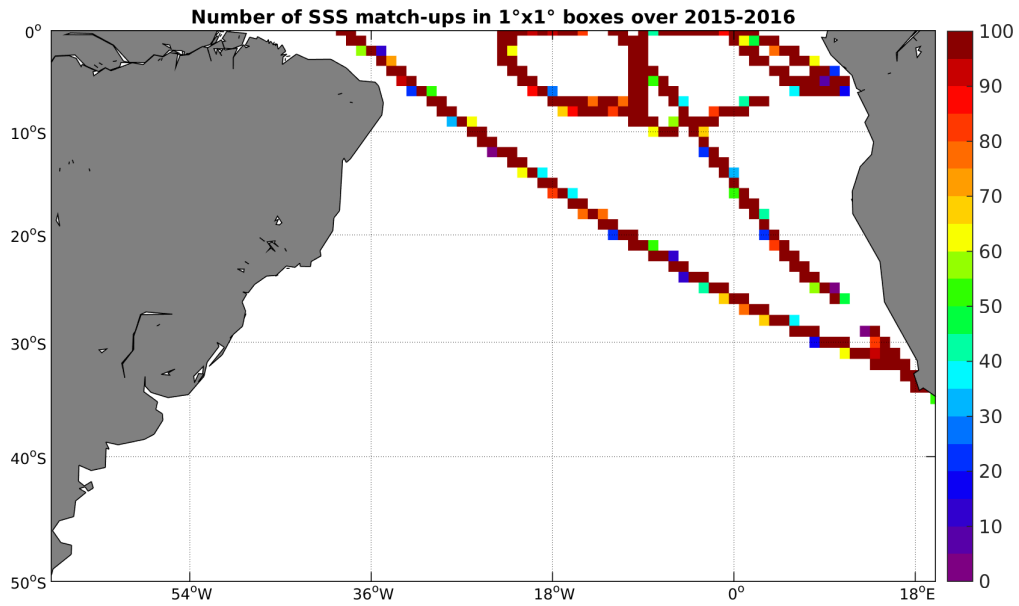
Figure 4: Number of SSS match-ups between TSG-GOSUD-Research-vessel SSS and the SMAP-L3-JPL-V4-8DAY-RUNNING-60KM SSS product for the South Atlantic Ocean Pi-MEP region over 1^\circ \times 1^\circ boxes and for the full satellite product period.
