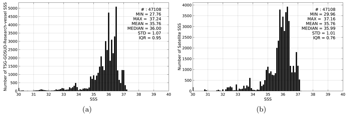
Figure 2: Histograms of SSS from TSG-GOSUD-Research-vessel (a) and SMAP-L3-JPL-V4-8DAY-RUNNING-60KM (b) considering all match-up pairs per bins of 0.1 over the South Atlantic Ocean Pi-MEP region and for the full satellite product period.
