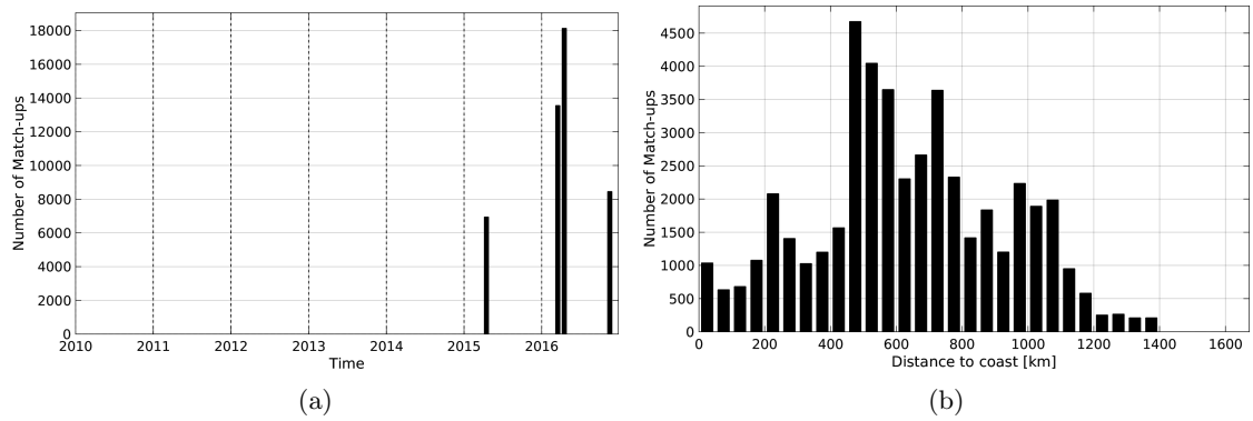
Figure 1: Number of match-ups between TSG-GOSUD-Research-vessel and SMAP-L3-JPL-V4-8DAY-RUNNING-60KM SSS as a function of time (a) and as function of the distance to coast (b) over the South Atlantic Ocean Pi-MEP region and for the full satellite product period.
