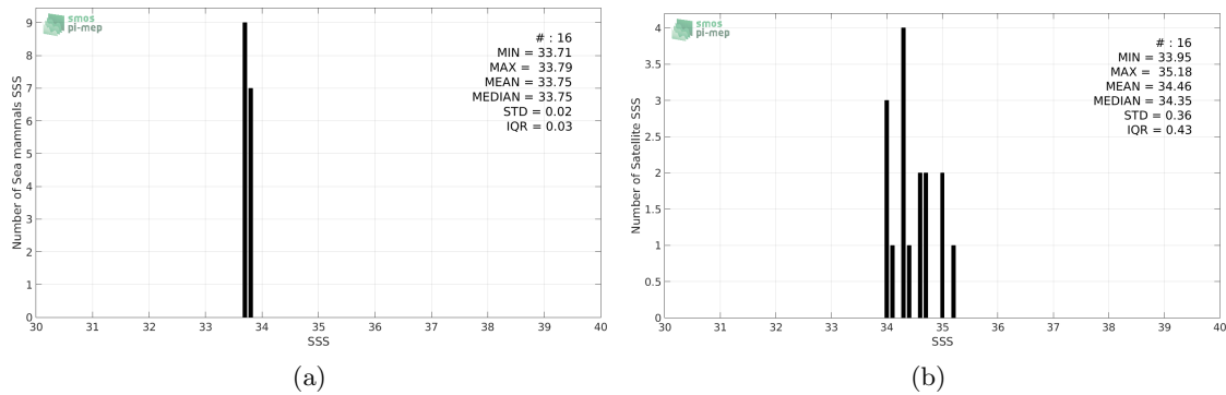
Figure 2: Histograms of SSS from Sea mammals (a) and SMAP-L3-JPL-V4-8DAY-RUNNING-60KM (b) considering all match-up pairs per bins of 0.1 over the South Atlantic Ocean Pi-MEP region and for the full satellite product period.
