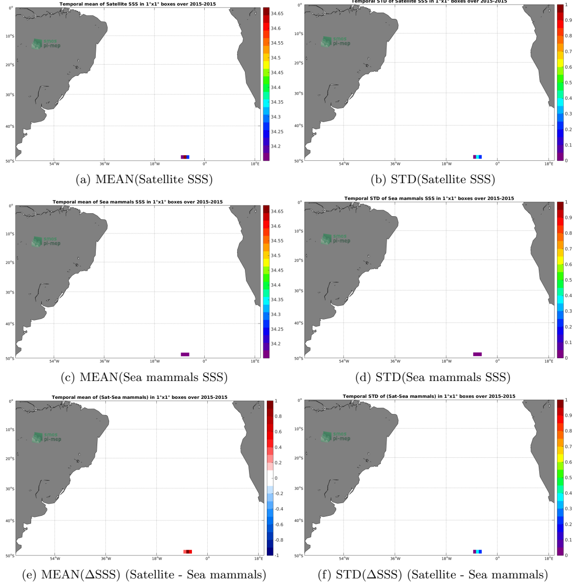
Figure 6: Temporal mean (left) and STD (right) of SSS from SMAP-L3-JPL-V4-8DAY-RUNNING-60KM (top), Sea mammals (middle), and of \Delta SSS (Satellite - Sea mammals). Only match-up pairs are used to generate these maps.
