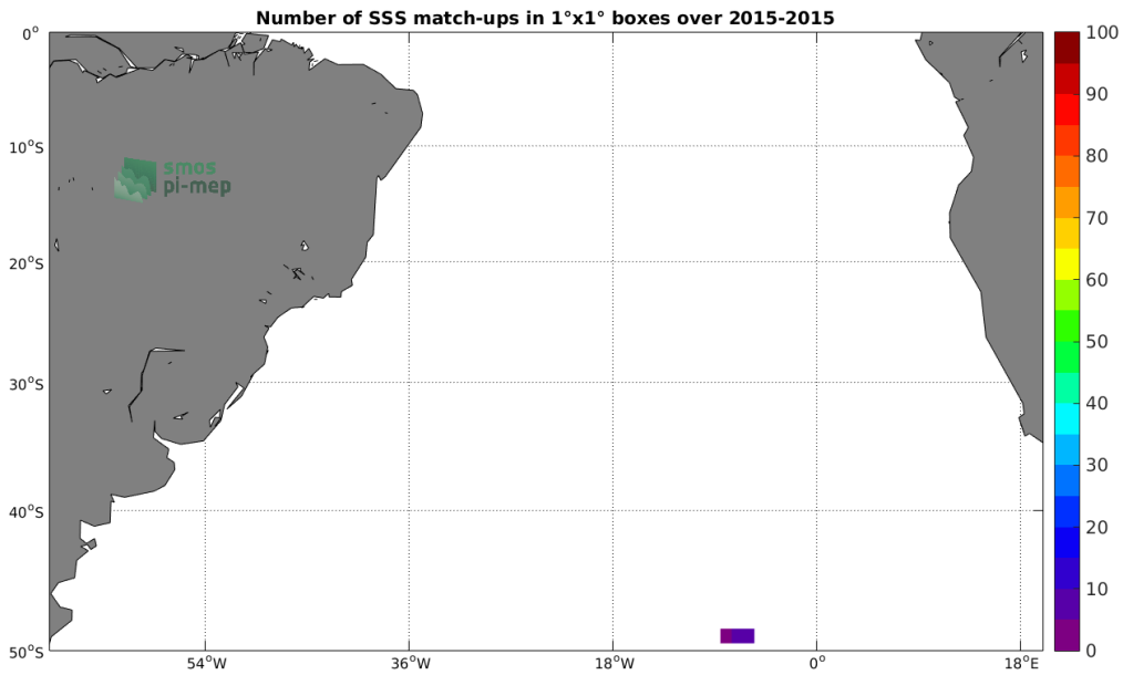
Figure 4: Number of SSS match-ups between Sea mammals SSS and the SMAP-L3-JPL-V4-8DAY-RUNNING-60KM SSS product for the South Atlantic Ocean Pi-MEP region over 1^\circ \times 1^\circ boxes and for the full satellite product period.
