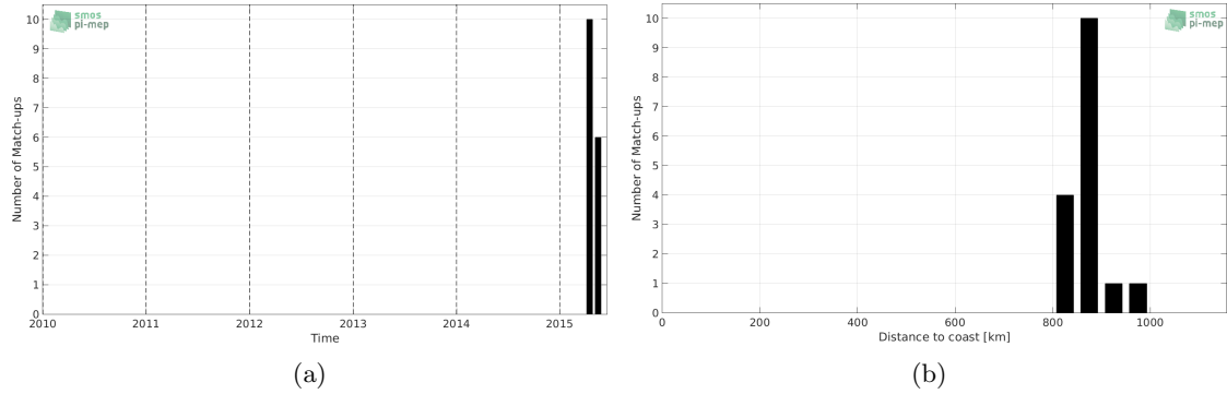
Figure 1: Number of match-ups between Sea mammals and SMAP-L3-JPL-V4-8DAY-RUNNING-60KM SSS as a function of time (a) and as function of the distance to coast (b) over the South Atlantic Ocean Pi-MEP region and for the full satellite product period.
