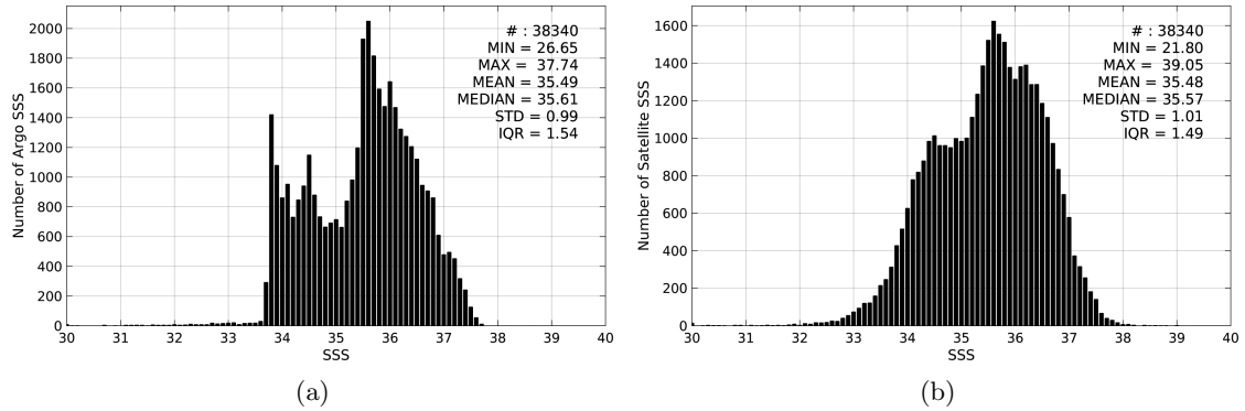
Figure 2: Histograms of SSS from Argo (a) and SMAP-L3-JPL-V4-8DAY-RUNNING-60KM (b) considering all match-up pairs per bins of 0.1 over the South Atlantic Ocean Pi-MEP region and for the full satellite product period.
