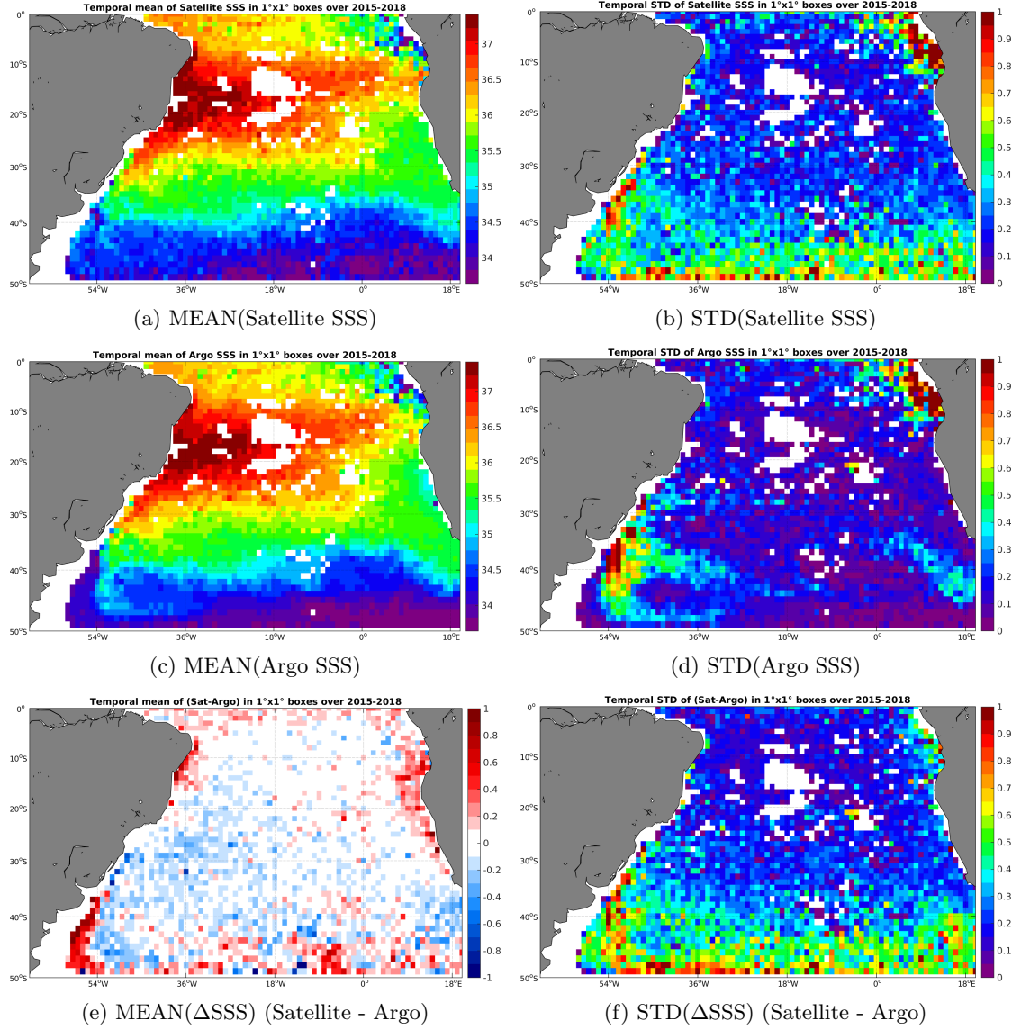
Figure 6: Temporal mean (left) and STD (right) of SSS from SMAP-L3-JPL-V4-8DAY-RUNNING-60KM (top), Argo (middle), and of \Delta SSS (Satellite - Argo). Only match-up pairs are used to generate these maps.
