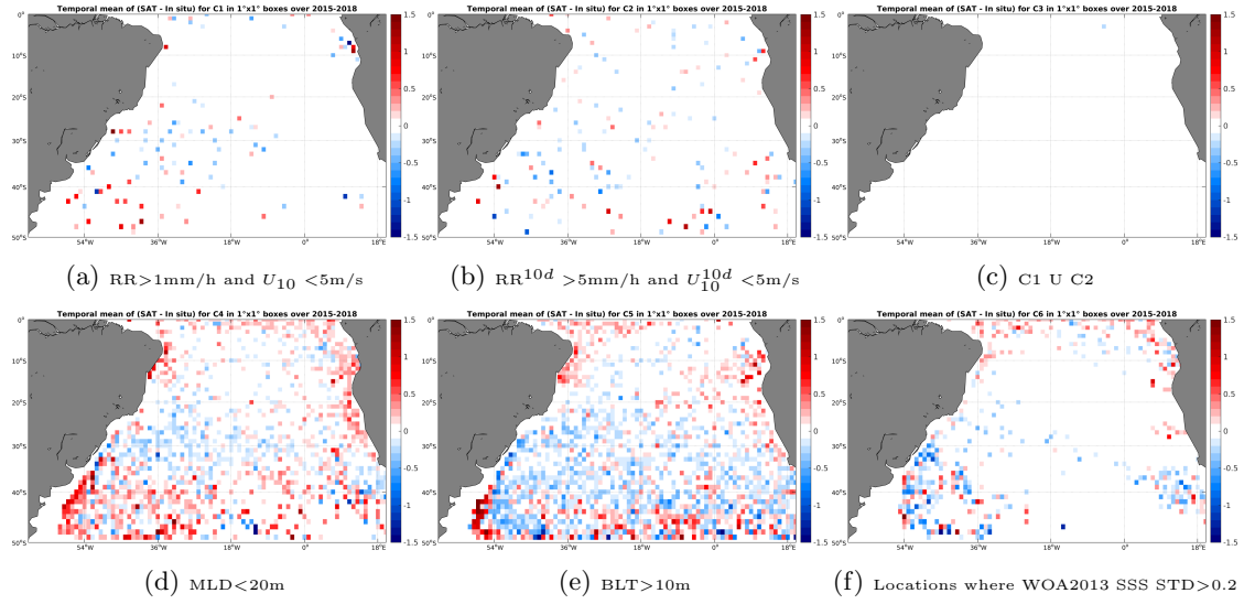
Figure 12: Temporal mean gridded over spatial boxes of size 1^\circ \times 1^\circ of \Delta SSS (SMAP-L3-JPL-V4-8DAY-RUNNING-60KM - Argo) for 6 different subdatasets corresponding to: RR > 1\text{mm/h} and U_{10} < 5\text{m/s} (a), RR^{10d} > 5\text{mm/h} and U_{10}^{10d} < 5\text{m/s} (b), C1 U C2 (c), MLD < 20\text{m} (d), BLT > 10\text{m} (e), Locations where WOA2013 SSS STD > 0.2 (f).
