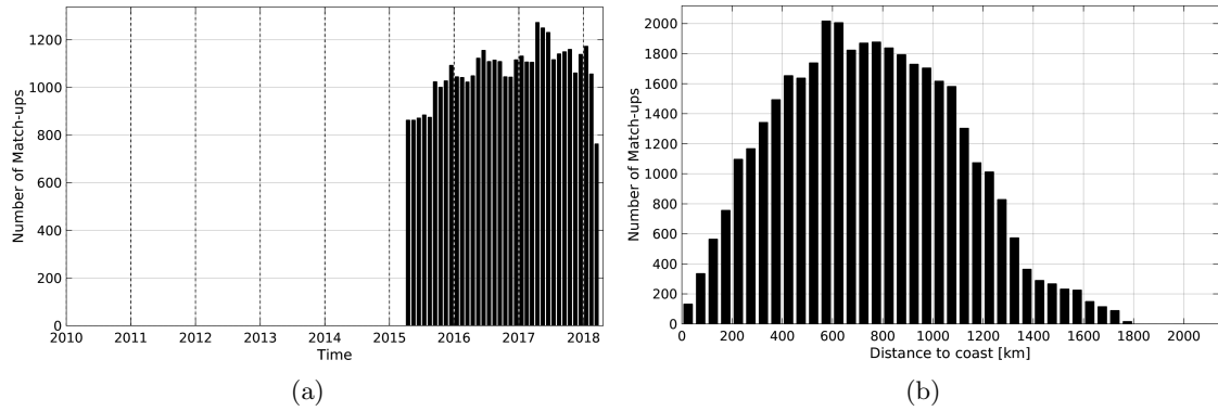
Figure 1: Number of match-ups between Argo and SMAP-L3-JPL-V4-8DAY-RUNNING-60KM SSS as a function of time (a) and as function of the distance to coast (b) over the South Atlantic Ocean Pi-MEP region and for the full satellite product period.
