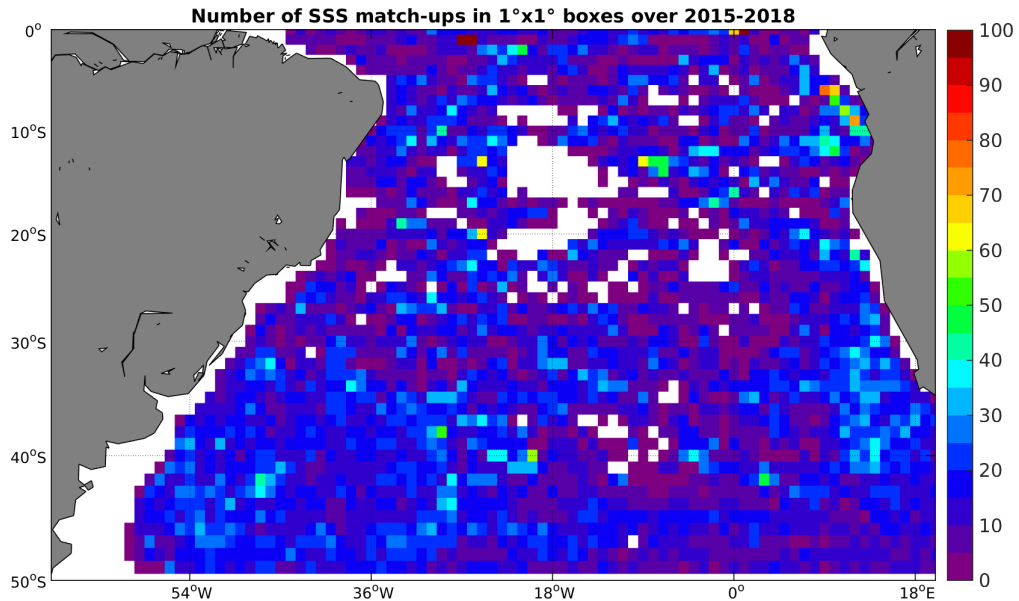
Figure 4: Number of SSS match-ups between Argo SSS and the SMAP-L3-JPL-V4-8DAY-RUNNING-60KM SSS product for the South Atlantic Ocean Pi-MEP region over 1^\circ \times 1^\circ boxes and for the full satellite product period.
