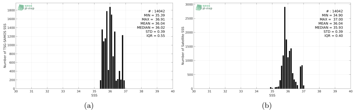
Figure 2: Histograms of SSS from TSG-SAMOS (a) and SMAP-L3-JPL-V4-MONTHLY-60KM (b) considering all match-up pairs per bins of 0.1 over the South Atlantic Ocean Pi-MEP region and for the full satellite product period.
