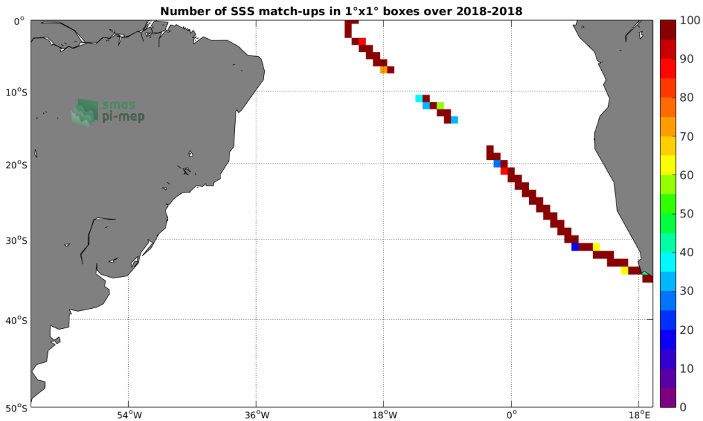
Figure 4: Number of SSS match-ups between TSG-SAMOS SSS and the SMAP-L3-JPL-V4-MONTHLY-60KM SSS product for the South Atlantic Ocean Pi-MEP region over 1^{\circ} \times 1^{\circ} boxes and for the full satellite product period.
