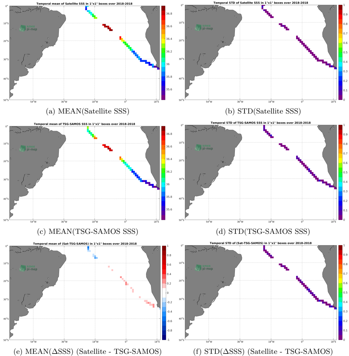
Figure 6: Temporal mean (left) and STD (right) of SSS from SMAP-L3-JPL-V4-MONTHLY-60KM (top), TSG-SAMOS (middle), and of \Delta SSS (Satellite - TSG-SAMOS). Only match-up pairs are used to generate these maps.
