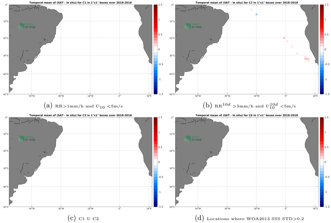
Figure 12: Temporal mean gridded over spatial boxes of size 1^\circ \times 1^\circ of \Delta SSS (SMAP-L3-JPL-V4-MONTHLY-60KM - TSG-SAMOS) for 4 different subdatasets corresponding to: RR > 1\text{mm/h} and U_{10} < 5\text{m/s} (a), RR^{10d} > 5\text{mm/h} and U_{10}^{10d} < 5\text{m/s} (b), C1 U C2 (c), Locations where WOA2013 SSS STD > 0.2 (d).
