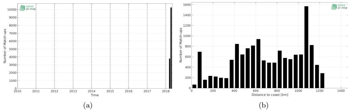
Figure 1: Number of match-ups between TSG-SAMOS and SMAP-L3-JPL-V4-MONTHLY-60KM SSS as a function of time (a) and as function of the distance to coast (b) over the South Atlantic Ocean Pi-MEP region and for the full satellite product period.
