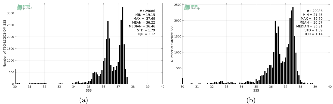
Figure 2: Histograms of SSS from TSG-LEGOS-DM (a) and SMAP-L3-JPL-V4-MONTHLY-60KM (b) considering all match-up pairs per bins of 0.1 over the South Atlantic Ocean Pi-MEP region and for the full satellite product period.
