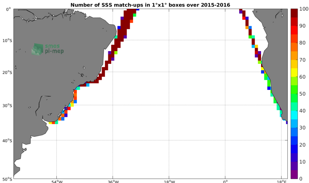
Figure 4: Number of SSS match-ups between TSG-LEGOS-DM SSS and the SMAP-L3-JPL-V4-MONTHLY-60KM SSS product for the South Atlantic Ocean Pi-MEP region over 1^\circ \times 1^\circ boxes and for the full satellite product period.
