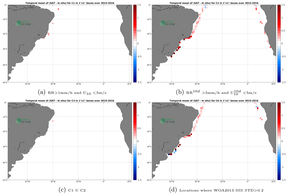
Figure 12: Temporal mean gridded over spatial boxes of size 1^\circ \times 1^\circ of \Delta SSS (SMAP-L3-JPL-V4-MONTHLY-60KM - TSG-LEGOS-DM) for 4 different subdatasets corresponding to: RR > 1\text{mm/h} and U_{10} < 5\text{m/s} (a), RR^{10d} > 5\text{mm/h} and U_{10}^{10d} < 5\text{m/s} (b), C1 U C2 (c), Locations where WOA2013 SSS STD > 0.2 (d).
