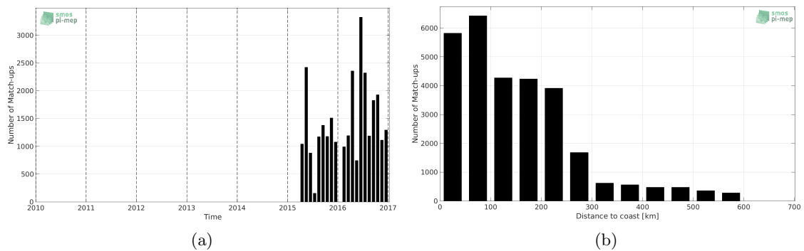
Figure 1: Number of match-ups between TSG-LEGOS-DM and SMAP-L3-JPL-V4-MONTHLY-60KM SSS as a function of time (a) and as function of the distance to coast (b) over the South Atlantic Ocean Pi-MEP region and for the full satellite product period.
