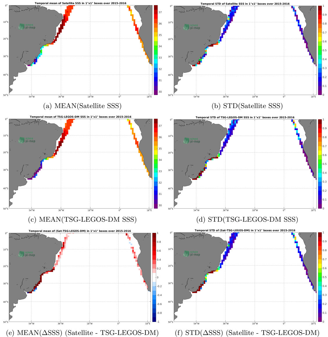
Figure 6: Temporal mean (left) and STD (right) of SSS from SMAP-L3-JPL-V4-MONTHLY-60KM (top), TSG-LEGOS-DM (middle), and of \Delta SSS (Satellite - TSG-LEGOS-DM). Only match-up pairs are used to generate these maps.
