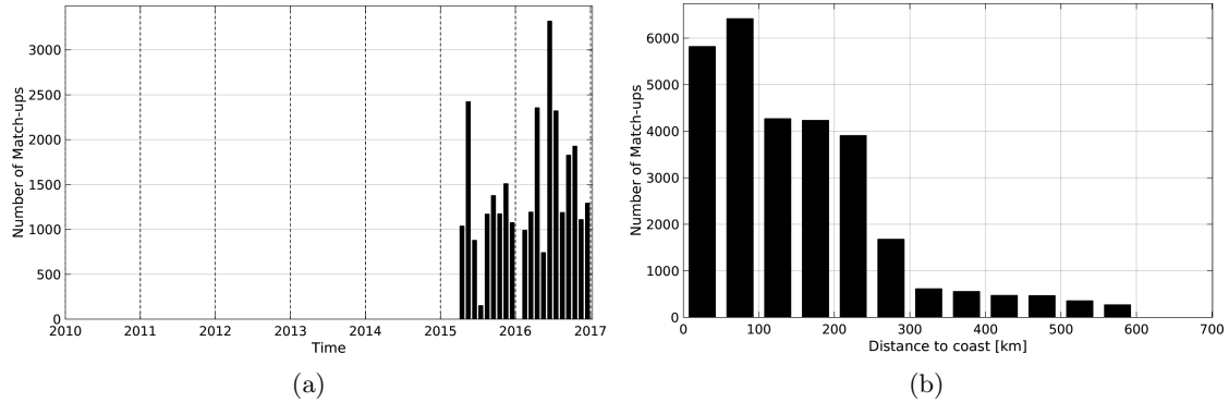
Figure 1: Number of match-ups between TSG-LEGOS-DM and SMAP-L3-JPL-V4-MONTHLY-60KM SSS as a function of time (a) and as function of the distance to coast (b) over the South Atlantic Ocean Pi-MEP region and for the full satellite product period.
