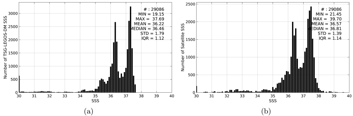
Figure 2: Histograms of SSS from TSG-LEGOS-DM (a) and SMAP-L3-JPL-V4-MONTHLY-60KM (b) considering all match-up pairs per bins of 0.1 over the South Atlantic Ocean Pi-MEP region and for the full satellite product period.
