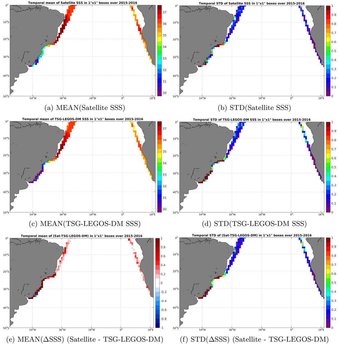
Figure 6: Temporal mean (left) and STD (right) of SSS from SMAP-L3-JPL-V4-MONTHLY-60KM (top), TSG-LEGOS-DM (middle), and of \Delta SSS (Satellite - TSG-LEGOS-DM). Only match-up pairs are used to generate these maps.
