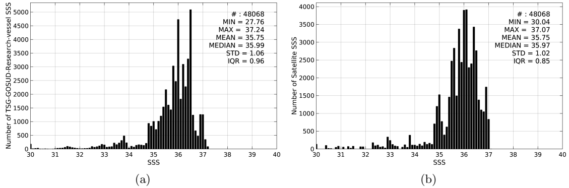
Figure 2: Histograms of SSS from TSG-GOSUD-Research-vessel (a) and SMAP-L3-JPL-V4-MONTHLY-60KM (b) considering all match-up pairs per bins of 0.1 over the South Atlantic Ocean Pi-MEP region and for the full satellite product period.
