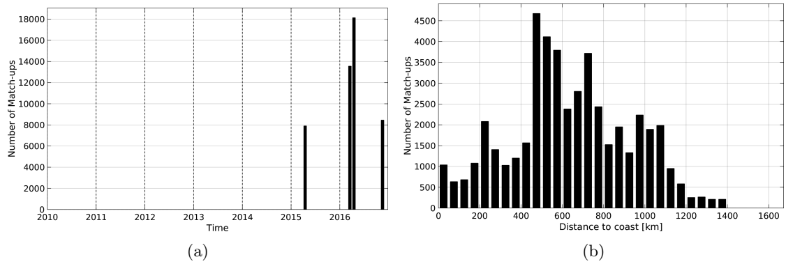
Figure 1: Number of match-ups between TSG-GOSUD-Research-vessel and SMAP-L3-JPL-V4-MONTHLY-60KM SSS as a function of time (a) and as function of the distance to coast (b) over the South Atlantic Ocean Pi-MEP region and for the full satellite product period.
