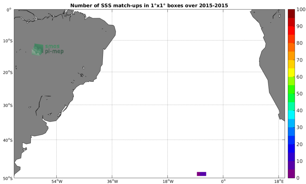
Figure 4: Number of SSS match-ups between Sea mammals SSS and the SMAP-L3-JPL-V4-MONTHLY-60KM SSS product for the South Atlantic Ocean Pi-MEP region over 1^\circ \times 1^\circ boxes and for the full satellite product period.
