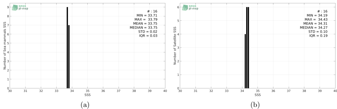
Figure 2: Histograms of SSS from Sea mammals (a) and SMAP-L3-JPL-V4-MONTHLY-60KM (b) considering all match-up pairs per bins of 0.1 over the South Atlantic Ocean Pi-MEP region and for the full satellite product period.
