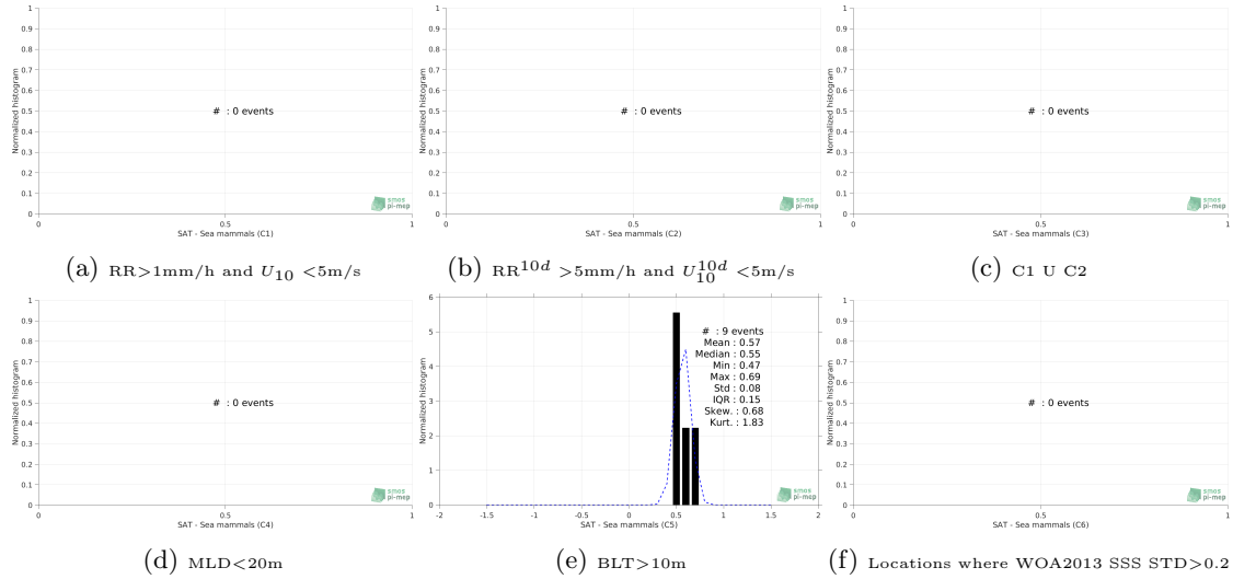
Figure 13: Normalized histogram of \Delta SSS (SMAP-L3-JPL-V4-MONTHLY-60KM - Sea mammals) for 6 different subdatasets corresponding to: RR>1mm/h and U_{10} < 5 m/s (a), RR 10d >5mm/h and U_{10}^{10d} < 5 m/s (b), C1 U C2 (c),MLD<20m (d),BLT>10m (e),Locations where WOA2013 SSS STD>0.2 (f).
