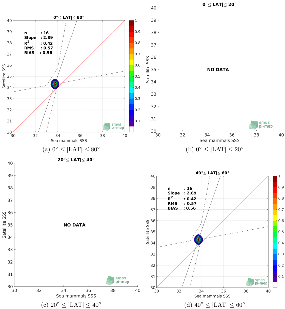
Figure 9: Contour maps of the concentration of SMAP-L3-JPL-V4-MONTHLY-60KM SSS (y-axis) versus Sea mammals SSS (x-axis) at match-up pairs for different latitude bands. For each plot, the red line shows x=y . The black thin and dashed lines indicate a linear fit through the data cloud and the \pm 95\% confidence levels, respectively. The number match-up pairs n , the slope and R^2 coefficient of the linear fit, the root mean square (RMS) and the mean bias between satellite and in situ data are indicated for each latitude band in each plots.
