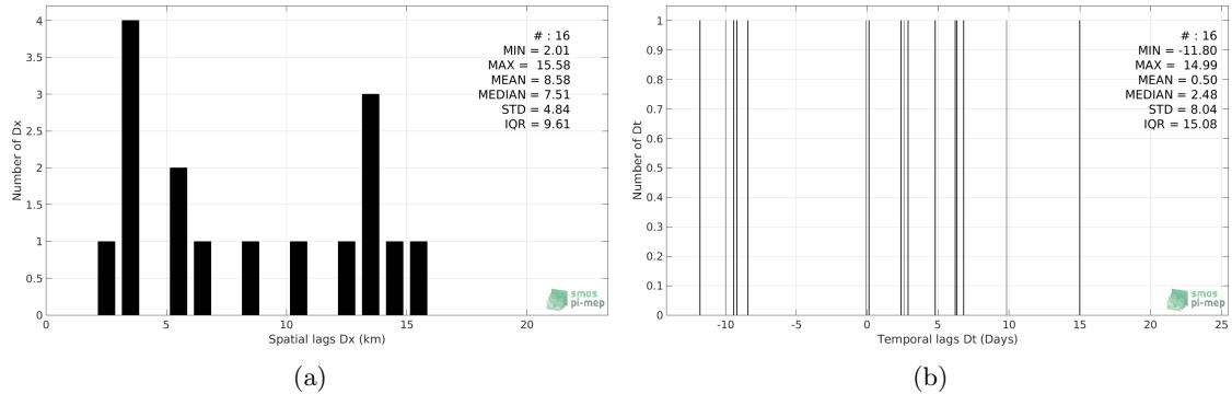
Figure 5: Histograms of the spatial (a) and temporal (b) lags between the time of the Sea mammals measurements and the date of the corresponding SMAP-L3-JPL-V4-MONTHLY-60KM SSS product.
