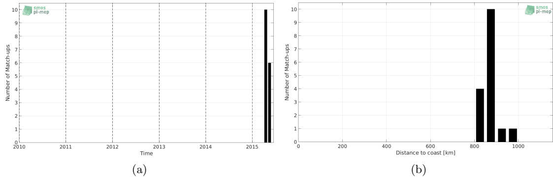
Figure 1: Number of match-ups between Sea mammals and SMAP-L3-JPL-V4-MONTHLY-60KM SSS as a function of time (a) and as function of the distance to coast (b) over the South Atlantic Ocean Pi-MEP region and for the full satellite product period.
