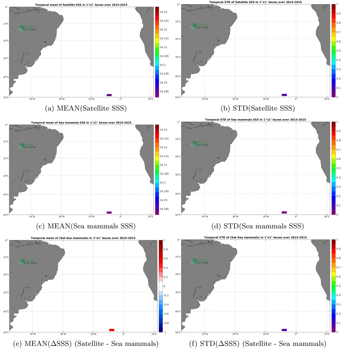
Figure 6: Temporal mean (left) and STD (right) of SSS from SMAP-L3-JPL-V4-MONTHLY-60KM (top), Sea mammals (middle), and of \Delta SSS (Satellite - Sea mammals). Only match-up pairs are used to generate these maps.
