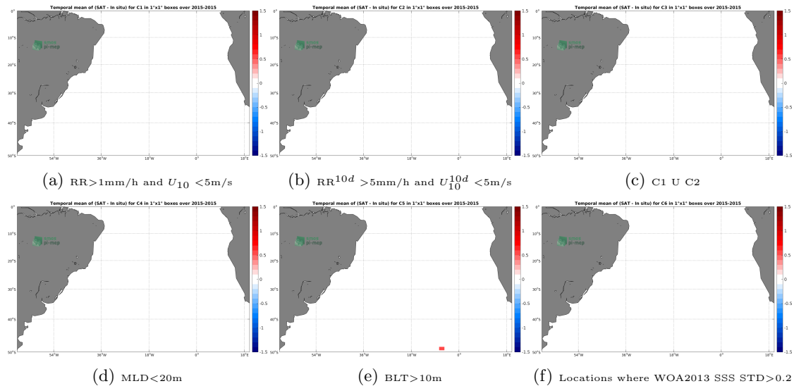
Figure 12: Temporal mean gridded over spatial boxes of size 1^\circ \times 1^\circ of \Delta\text{SSS} (SMAP-L3-JPL-V4-MONTHLY-60KM - Sea mammals) for 6 different subdatasets corresponding to: \text{RR} > 1\text{mm/h} and U_{10} < 5\text{m/s} (a), \text{RR}^{10d} > 5\text{mm/h} and U_{10}^{10d} < 5\text{m/s} (b), C1 U C2 (c), \text{MLD} < 20\text{m} (d), \text{BLT} > 10\text{m} (e), Locations where WOA2013 SSS STD > 0.2 (f).
