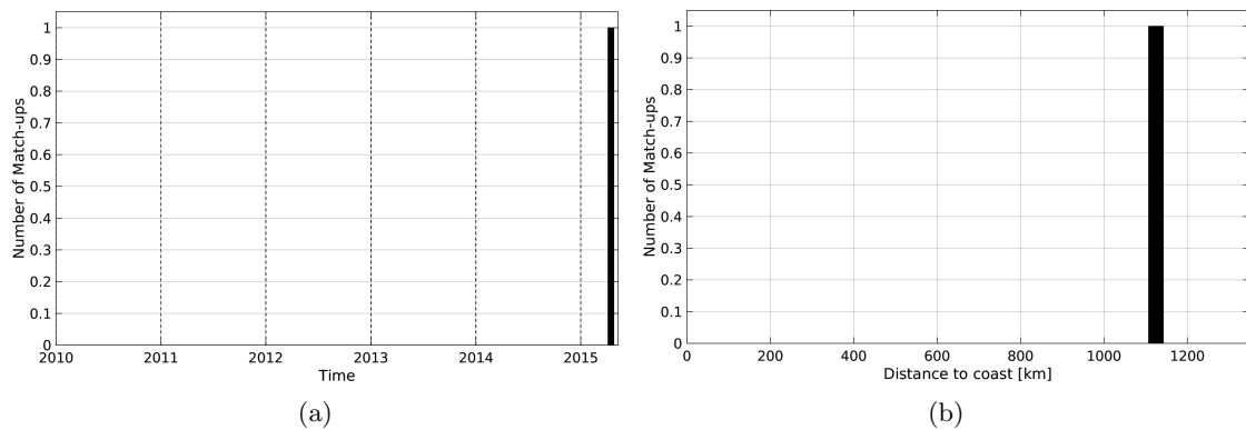
Figure 1: Number of match-ups between Surface drifters and SMAP-L3-JPL-V4-MONTHLY-60KM SSS as a function of time (a) and as function of the distance to coast (b) over the South Atlantic Ocean Pi-MEP region and for the full satellite product period.
