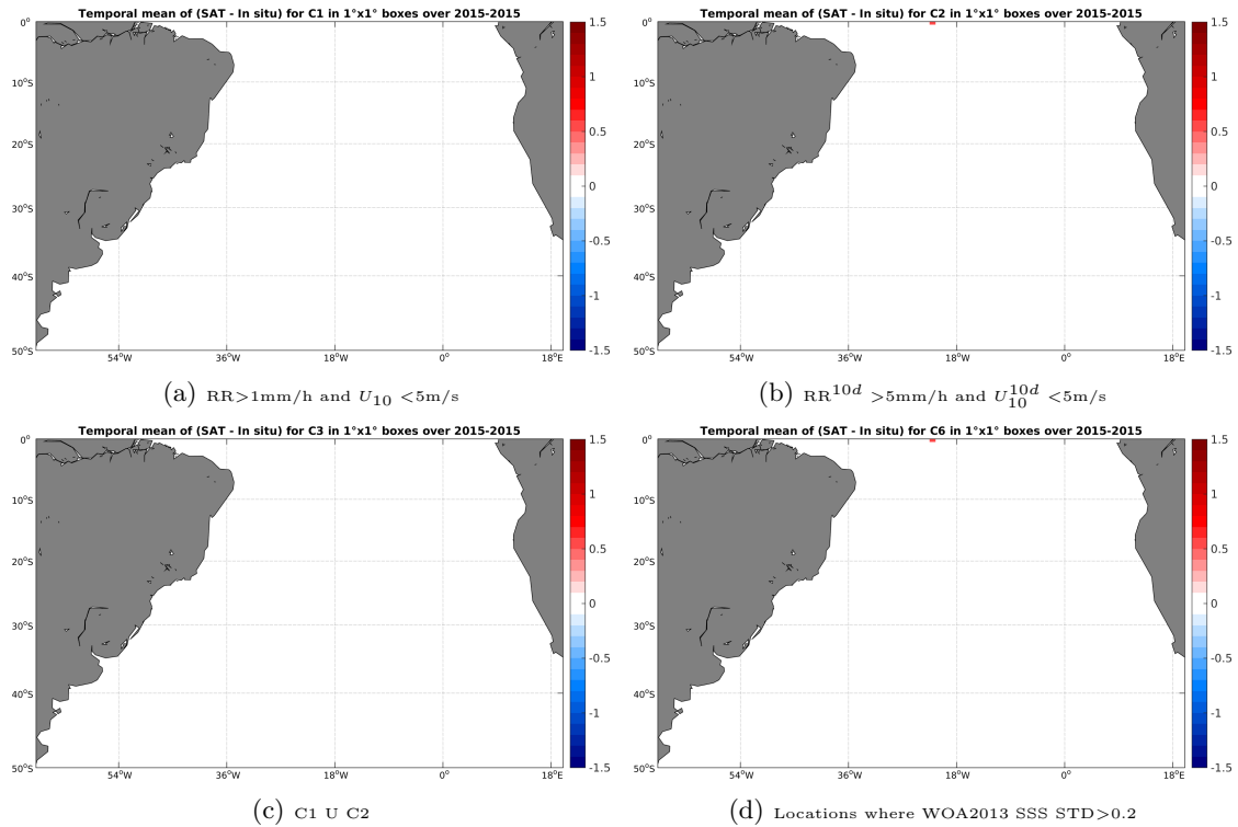
Figure 11: Temporal mean gridded over spatial boxes of size 1^\circ \times 1^\circ of \Delta SSS (SMAP-L3-JPL-V4-MONTHLY-60KM - Surface drifters) for 4 different subdatasets corresponding to: RR > 1\text{mm/h} and U_{10} < 5\text{m/s} (a), RR^{10d} > 5\text{mm/h} and U_{10}^{10d} < 5\text{m/s} (b), C1 U C2 (c), Locations where WOA2013 SSS STD > 0.2 (d).
