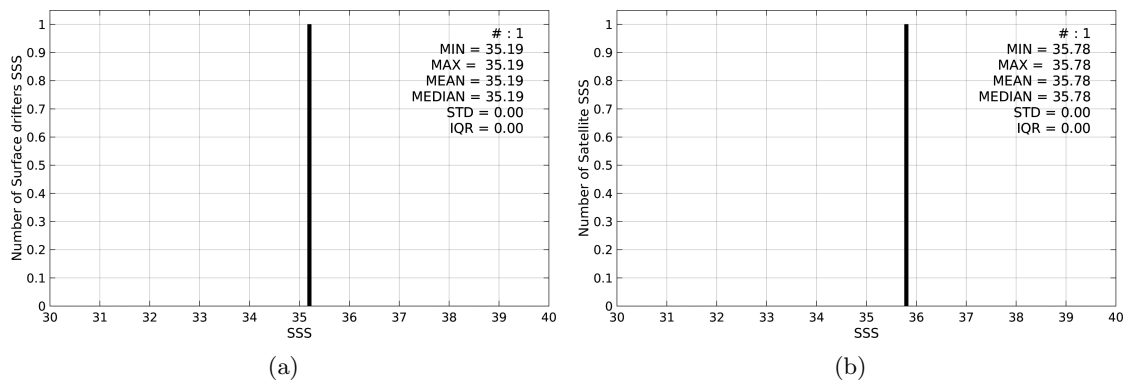
Figure 2: Histograms of SSS from Surface drifters (a) and SMAP-L3-JPL-V4-MONTHLY-60KM (b) considering all match-up pairs per bins of 0.1 over the South Atlantic Ocean Pi-MEP region and for the full satellite product period.
