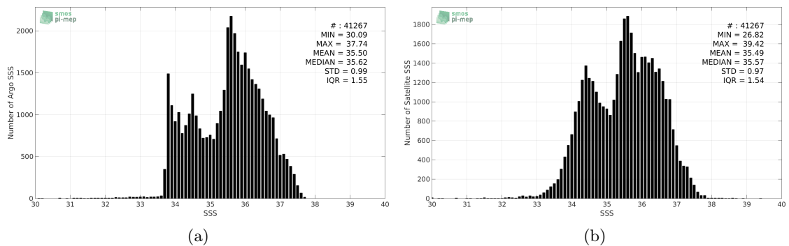
Figure 2: Histograms of SSS from Argo (a) and SMAP-L3-JPL-V4-MONTHLY-60KM (b) considering all match-up pairs per bins of 0.1 over the South Atlantic Ocean Pi-MEP region and for the full satellite product period.
