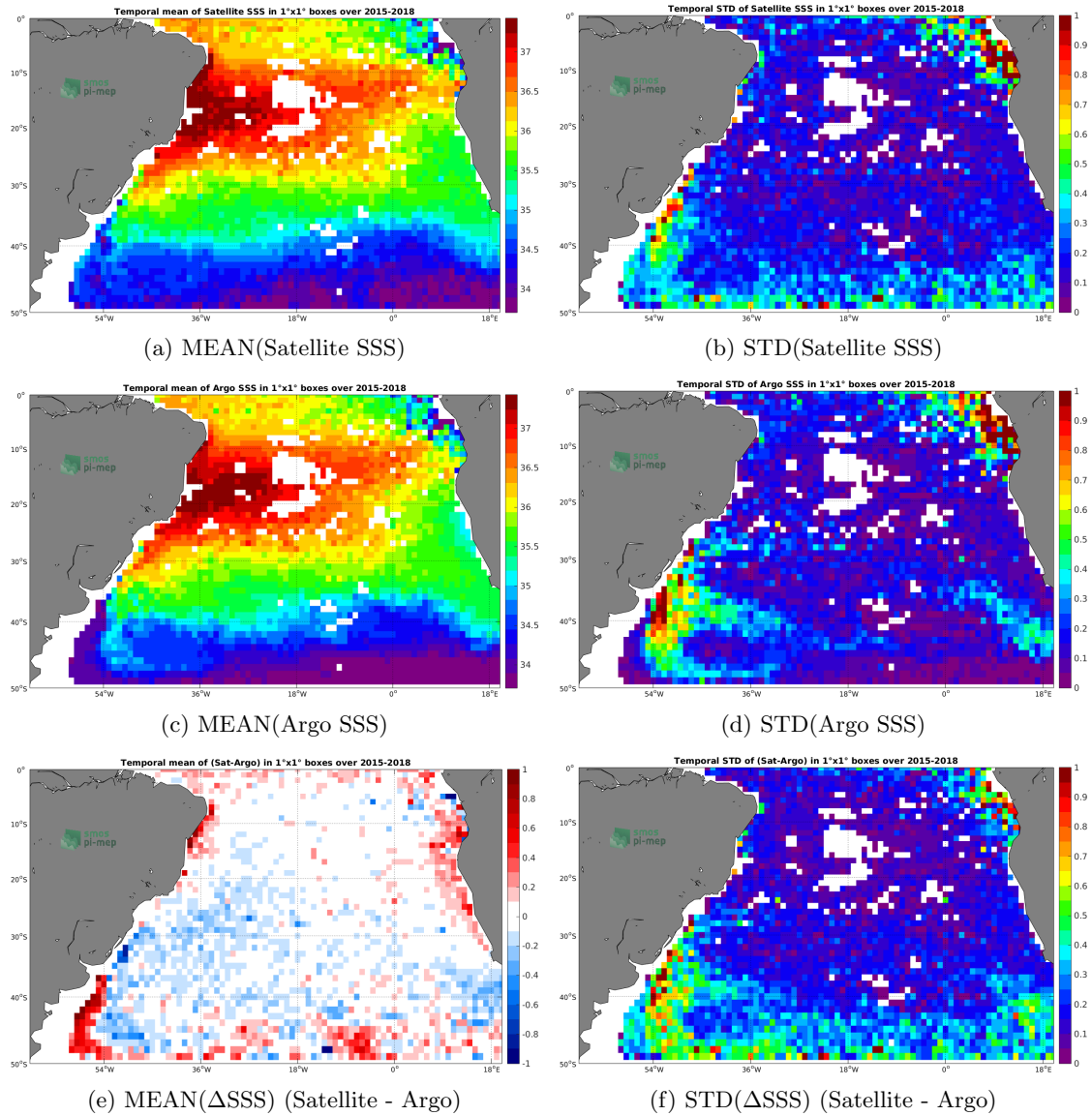
Figure 6: Temporal mean (left) and STD (right) of SSS from SMAP-L3-JPL-V4-MONTHLY-60KM (top), Argo (middle), and of \Delta SSS (Satellite - Argo). Only match-up pairs are used to generate these maps.
