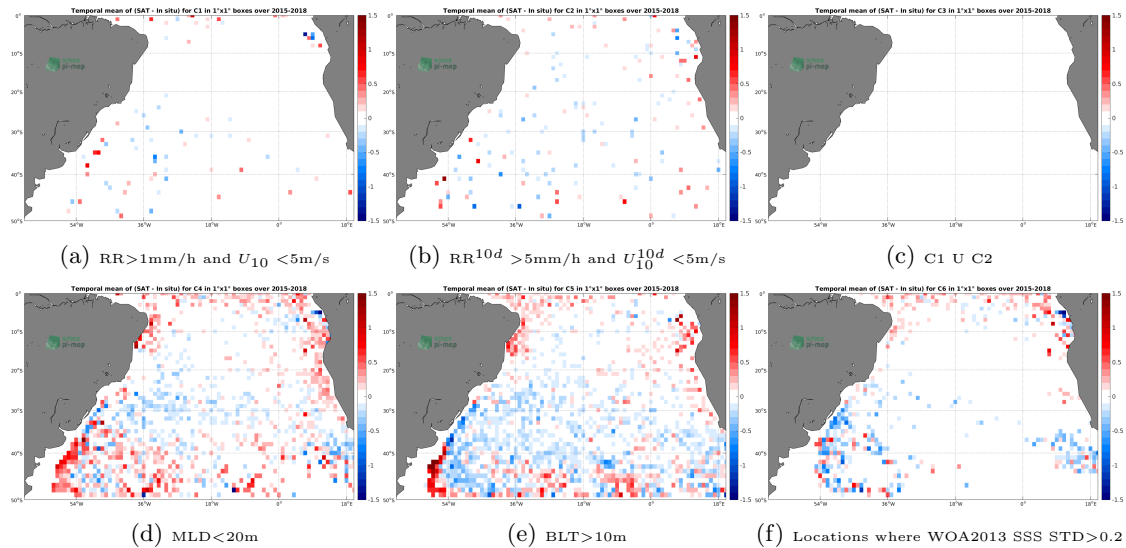
Figure 12: Temporal mean gridded over spatial boxes of size 1^\circ \times 1^\circ of \Delta\text{SSS} (SMAP-L3-JPL-V4-MONTHLY-60KM - Argo) for 6 different subdatasets corresponding to: \text{RR} > 1\text{mm/h} and U_{10} < 5\text{m/s} (a), \text{RR}^{10d} > 5\text{mm/h} and U_{10}^{10d} < 5\text{m/s} (b), C1 U C2 (c), \text{MLD} < 20\text{m} (d), \text{BLT} > 10\text{m} (e), Locations where WOA2013 SSS STD > 0.2 (f).
