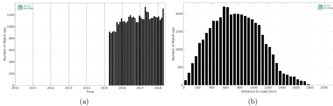
Figure 1: Number of match-ups between Argo and SMAP-L3-JPL-V4-MONTHLY-60KM SSS as a function of time (a) and as function of the distance to coast (b) over the South Atlantic Ocean Pi-MEP region and for the full satellite product period.
