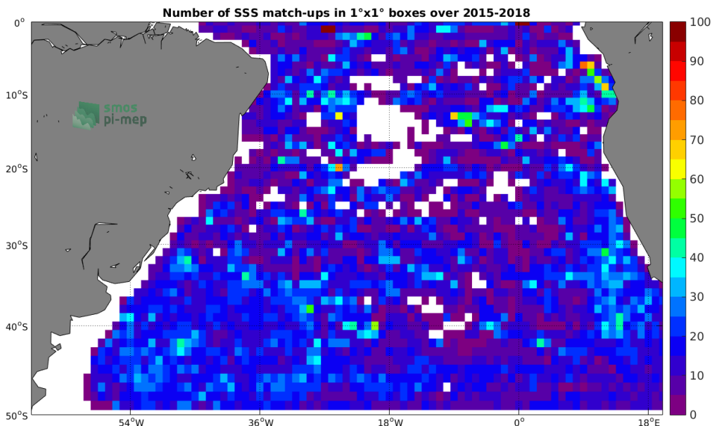
Figure 4: Number of SSS match-ups between Argo SSS and the SMAP-L3-JPL-V4-MONTHLY-60KM SSS product for the South Atlantic Ocean Pi-MEP region over 1°x1° boxes and for the full satellite product period.
