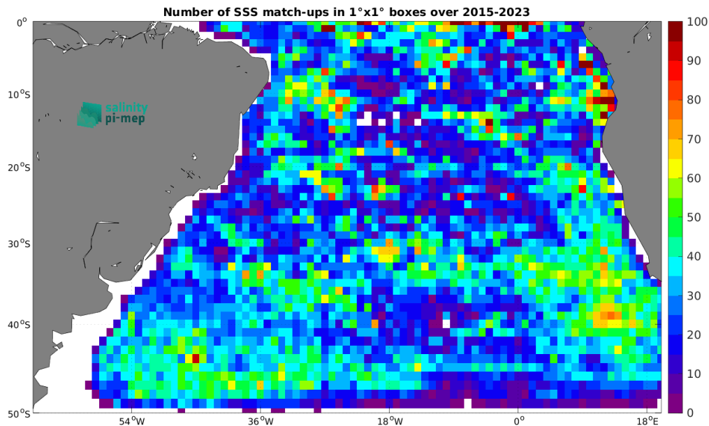
Figure 4: Number of SSS match-ups between Argo SSS and the SMAP SSS L2-AVERAGED v5 (RSS) SSS product for the South Atlantic Ocean Pi-MEP region over 1^\circ \times 1^\circ boxes and for the full satellite product period.
