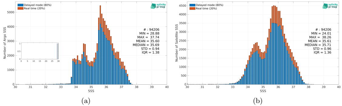
Figure 2: Histograms of SSS from Argo (a) and SMAP SSS L2-AVERAGED v5 (RSS) (b) considering all match-up pairs per bins of 0.1 over the South Atlantic Ocean Pi-MEP region and for the full satellite product period.
