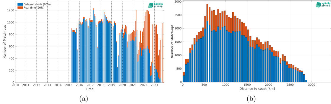
Figure 1: Number of match-ups between Argo and SMAP SSS L2-AVERAGED v5 (RSS) SSS as a function of time (a) and as function of the distance to coast (b) over the South Atlantic Ocean Pi-MEP region and for the full satellite product period.
