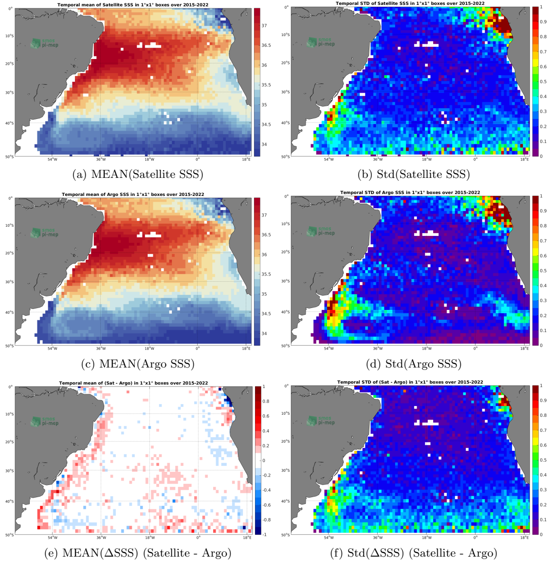
Figure 6: Temporal mean (left) and Std (right) of SSS from SMAP SSS L2-AVERAGED v5 (RSS) (top), Argo (middle), and of \Delta SSS (Satellite - Argo). Only match-up pairs are used to generate these maps.
