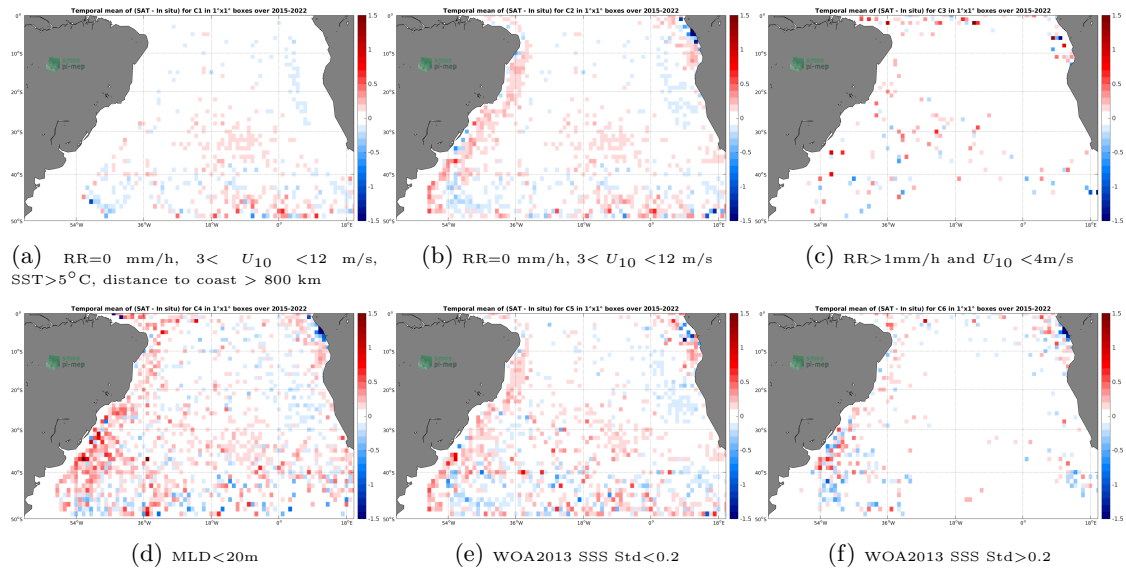
Figure 12: Temporal mean gridded over spatial boxes of size 1^\circ \times 1^\circ of \Delta SSS (SMAP SSS L2-AVERAGED v5 (RSS) - Argo) for 6 different subdatasets corresponding to:RR=0 mm/h, 3 < U_{10} < 12 m/s, SST >5^\circ\text{C} , distance to coast > 800 km (a), RR=0 mm/h, 3 < U_{10} < 12 m/s (b), RR >1 mm/h and U_{10} < 4 m/s (c),MLD <20 m (d),WOA2013 SSS Std <0.2 (e),WOA2013 SSS Std >0.2 (f).
