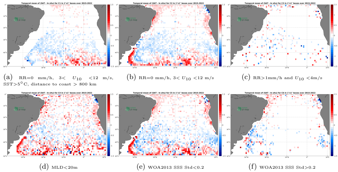
Figure 12: Temporal mean gridded over spatial boxes of size 1^\circ \times 1^\circ of \Delta SSS (SMAP SSS L2-AVERAGED v5.0 (JPL) - Argo) for 6 different subdatasets corresponding to:RR=0 mm/h, 3 < U_{10} < 12 m/s, SST >5^\circ\text{C} , distance to coast > 800 km (a), RR=0 mm/h, 3 < U_{10} < 12 m/s (b), RR >1 mm/h and U_{10} < 4 m/s (c),MLD <20 m (d),WOA2013 SSS Std <0.2 (e),WOA2013 SSS Std >0.2 (f).
