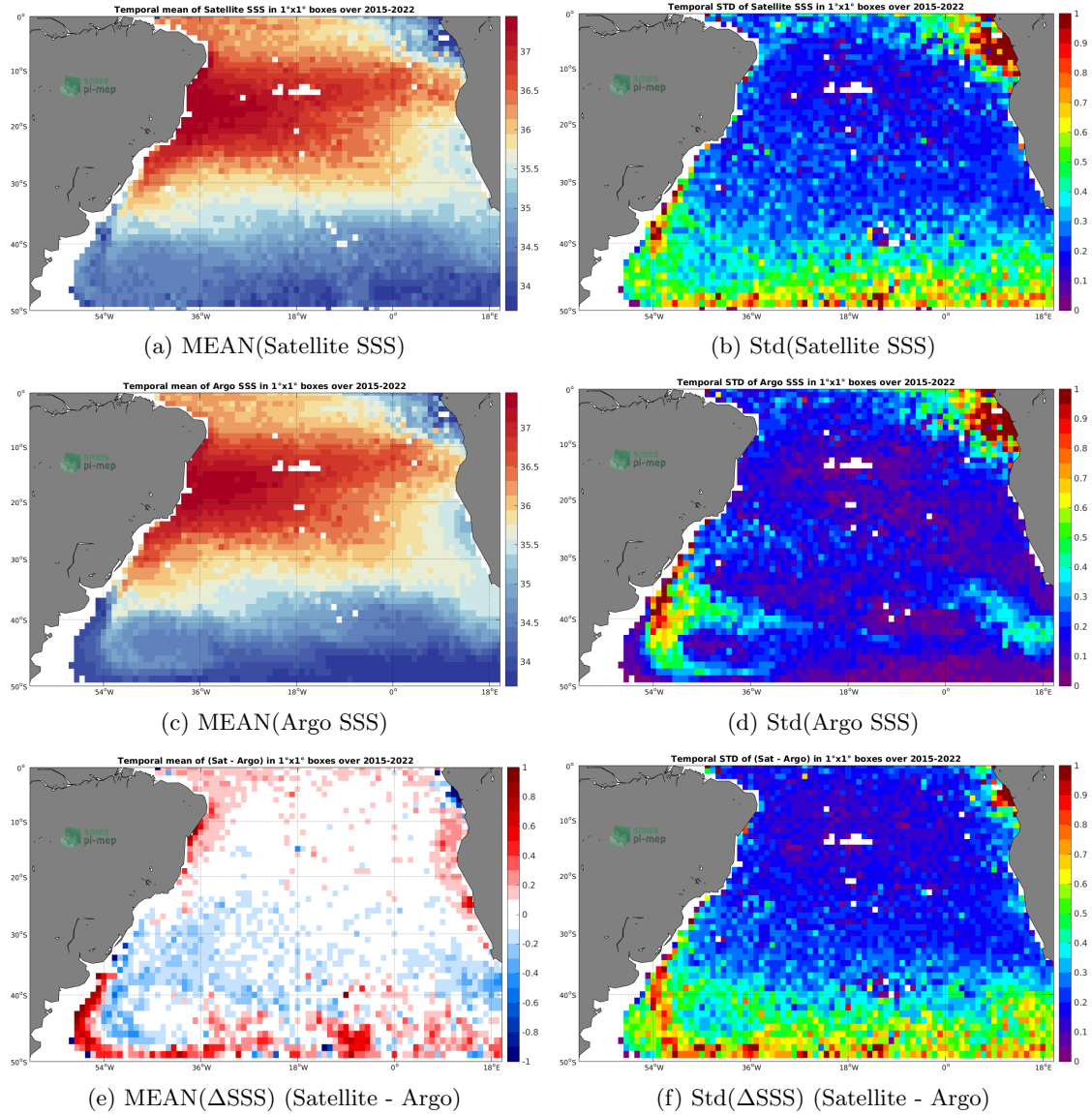
Figure 6: Temporal mean (left) and Std (right) of SSS from SMAP SSS L2-AVERAGED v5.0 (JPL) (top), Argo (middle), and of \Delta SSS (Satellite - Argo). Only match-up pairs are used to generate these maps.
