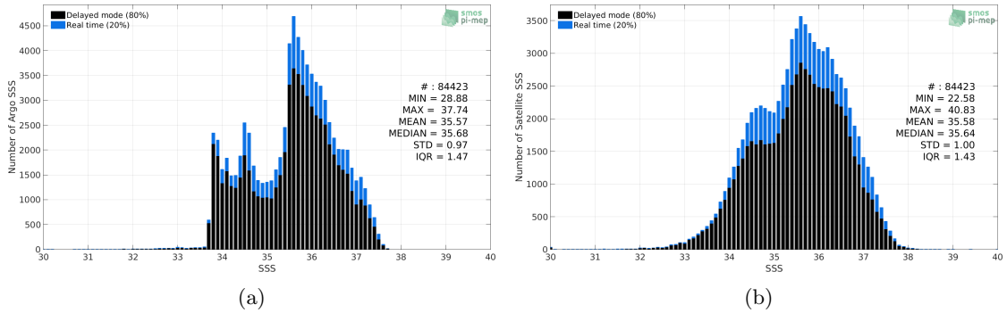
Figure 2: Histograms of SSS from Argo (a) and SMAP SSS L2-AVERAGED v5.0 (JPL) (b) considering all match-up pairs per bins of 0.1 over the South Atlantic Ocean Pi-MEP region and for the full satellite product period.
