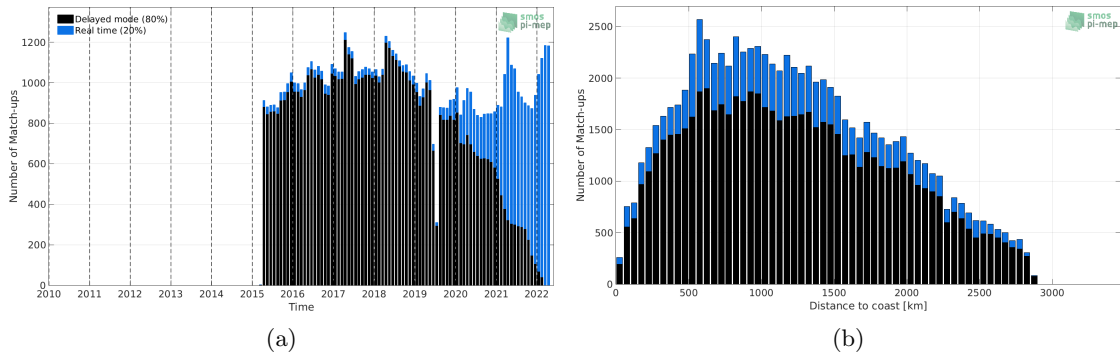
Figure 1: Number of match-ups between Argo and SMAP SSS L2-AVERAGED v5.0 (JPL) SSS as a function of time (a) and as function of the distance to coast (b) over the South Atlantic Ocean Pi-MEP region and for the full satellite product period.
