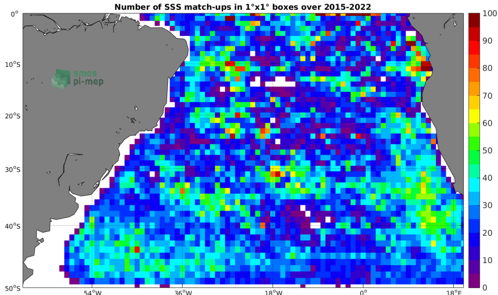
Figure 4: Number of SSS match-ups between Argo SSS and the SMAP SSS L2-AVERAGED v5.0 (JPL) SSS product for the South Atlantic Ocean Pi-MEP region over 1^\circ \times 1^\circ boxes and for the full satellite product period.
