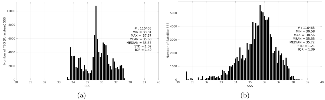
Figure 3: Histograms of SSS from TSG (Polarstern) (a) and SMAP SSS L2 v6 (RSS) (b) considering all match-up pairs per bins of 0.1 over the South Atlantic Ocean Pi-MEP region and for the full satellite product period.
