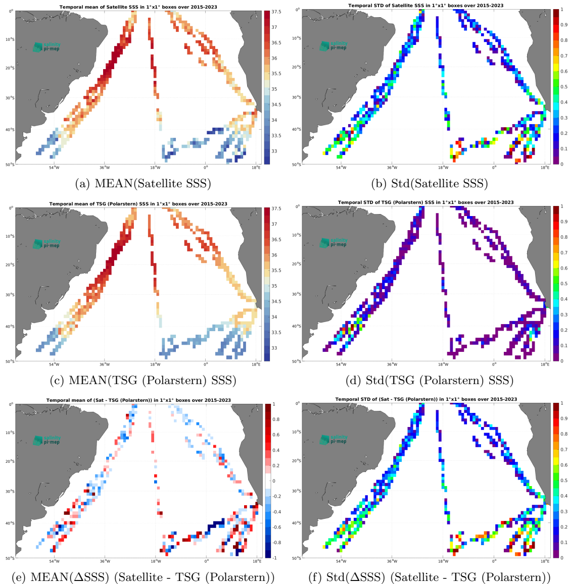
Figure 7: Temporal mean (left) and Std (right) of SSS from SMAP SSS L2 v6 (RSS) (top), TSG (Polarstern) (middle), and of \Delta SSS (Satellite - TSG (Polarstern)). Only match-up pairs are used to generate these maps.
