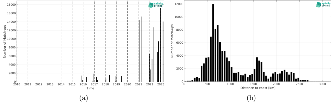
Figure 2: Number of match-ups between TSG (Polarstern) and SMAP SSS L2 v6 (RSS) SSS as a function of time (a) and as function of the distance to coast (b) over the South Atlantic Ocean Pi-MEP region and for the full satellite product period.
