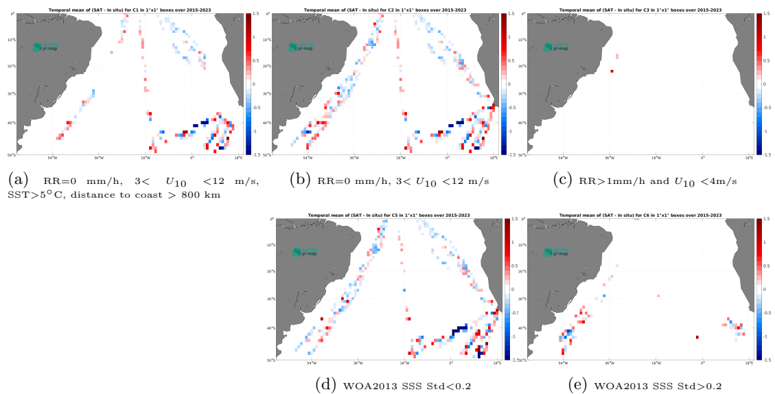
Figure 14: Temporal mean gridded over spatial boxes of size 1^\circ \times 1^\circ of \Delta SSS (SMAP SSS L2 v6 (RSS) - TSG (Polarstern)) for 5 different subdatasets corresponding to:RR=0 mm/h, 3 < U_{10} < 12 m/s, SST>5°C, distance to coast > 800 km (a), RR=0 mm/h, 3 < U_{10} < 12 m/s (b), RR>1mm/h and U_{10} < 4 m/s (c), WOA2013 SSS Std<0.2 (d), WOA2013 SSS Std>0.2 (e).
