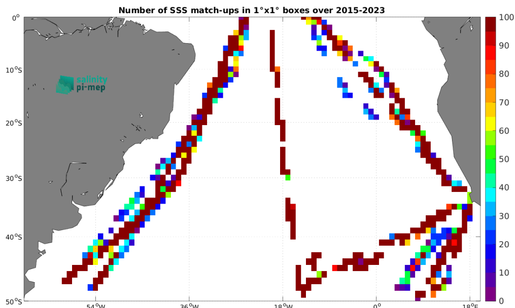
Figure 5: Number of SSS match-ups between TSG (Polarstern) SSS and the SMAP SSS L2 v6 (RSS) SSS product for the South Atlantic Ocean Pi-MEP region over 1^\circ \times 1^\circ boxes and for the full satellite product period.
