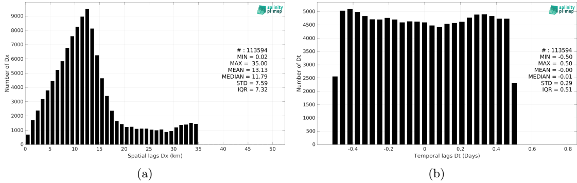
Figure 6: Histograms of the spatial (a) and temporal (b) lags between the location/time of the TSG (LEGOS-DM) measurement and the date of the corresponding SMAP SSS L2 v6 (RSS) SSS pixel.
