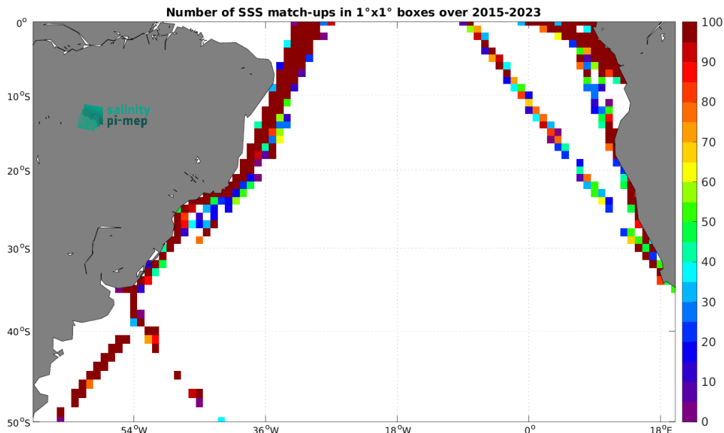
Figure 5: Number of SSS match-ups between TSG (LEGOS-DM) SSS and the SMAP SSS L2 v6 (RSS) SSS product for the South Atlantic Ocean Pi-MEP region over 1^\circ \times 1^\circ boxes and for the full satellite product period.
