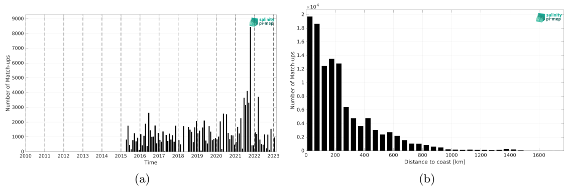
Figure 2: Number of match-ups between TSG (LEGOS-DM) and SMAP SSS L2 v6 (RSS) SSS as a function of time (a) and as function of the distance to coast (b) over the South Atlantic Ocean Pi-MEP region and for the full satellite product period.
