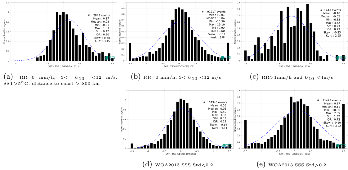
Figure 15: Normalized histogram of \Delta SSS (SMAP SSS L2 v6 (RSS) - TSG (LEGOS-DM)) for 5 different subdatasets corresponding to: RR=0 mm/h, 3 < U_{10} < 12 m/s, SST>5°C, distance to coast > 800 km (a), RR=0 mm/h, 3 < U_{10} < 12 m/s (b), RR>1mm/h and U_{10} < 4 m/s (c), WOA2013 SSS Std<0.2 (d), WOA2013 SSS Std>0.2 (e).
