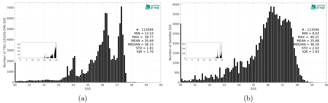
Figure 3: Histograms of SSS from TSG (LEGOS-DM) (a) and SMAP SSS L2 v6 (RSS) (b) considering all match-up pairs per bins of 0.1 over the South Atlantic Ocean Pi-MEP region and for the full satellite product period.
