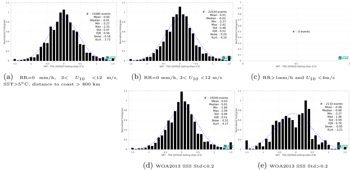
Figure 15: Normalized histogram of \Delta SSS (SMAP SSS L2 v6 (RSS) - TSG (GOSUD-Sailing-ship)) for 5 different subdatasets corresponding to: RR=0 mm/h, 3 < U_{10} < 12 m/s, SST > 5°C, distance to coast > 800 km (a), RR=0 mm/h, 3 < U_{10} < 12 m/s (b), RR > 1mm/h and U_{10} < 4 m/s (c), WOA2013 SSS Std < 0.2 (d), WOA2013 SSS Std > 0.2 (e).
