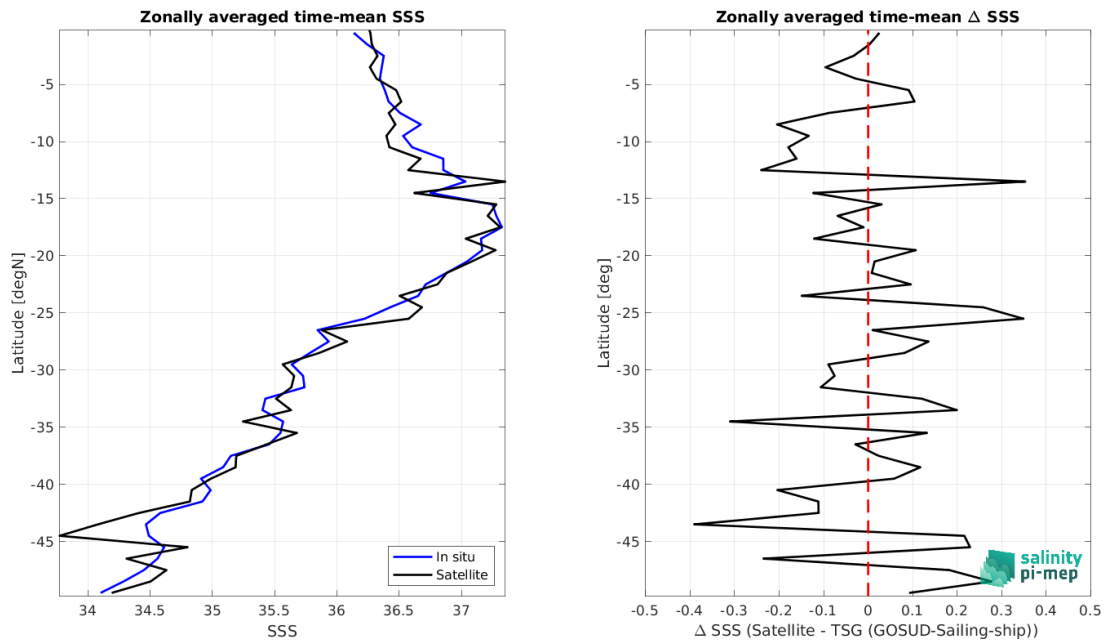
Figure 9: Left panel: Zonal mean SSS from SMAP SSS L2 v6 (RSS) satellite product (black) and from TSG (GOSUD-Sailing-ship) (blue). Right panel: Zonal mean of \Delta SSS (Satellite - TSG (GOSUD-Sailing-ship)) for all the collected Pi-MEP match-up pairs estimated over the full satellite product period.
