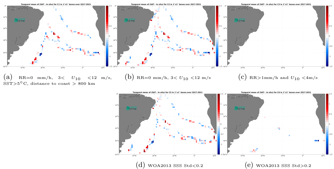
Figure 14: Temporal mean gridded over spatial boxes of size 1^\circ \times 1^\circ of \Delta\text{SSS} (SMAP SSS L2 v6 (RSS) - TSG (GOSUD-Sailing-ship)) for 5 different subdatasets corresponding to:RR=0 mm/h, 3 < U_{10} < 12 m/s, SST>5°C, distance to coast > 800 km (a), RR=0 mm/h, 3 < U_{10} < 12 m/s (b), RR>1mm/h and U_{10} < 4 m/s (c), WOA2013 SSS Std<0.2 (d), WOA2013 SSS Std>0.2 (e).
