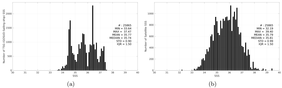
Figure 3: Histograms of SSS from TSG (GOSUD-Sailing-ship) (a) and SMAP SSS L2 v6 (RSS) (b) considering all match-up pairs per bins of 0.1 over the South Atlantic Ocean Pi-MEP region and for the full satellite product period.
