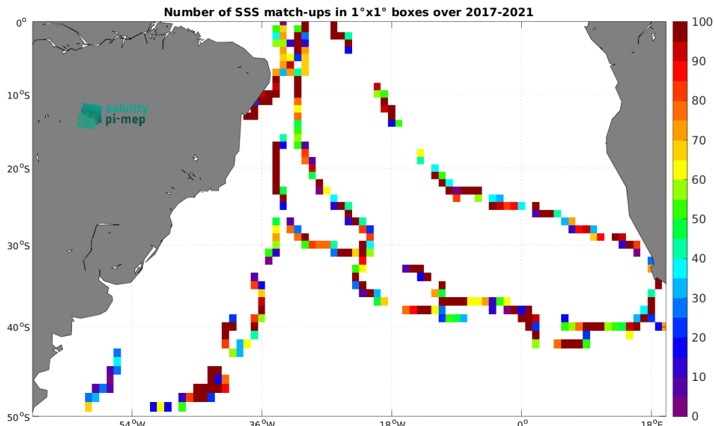
Figure 5: Number of SSS match-ups between TSG (GOSUD-Sailing-ship) SSS and the SMAP SSS L2 v6 (RSS) SSS product for the South Atlantic Ocean Pi-MEP region over 1^\circ \times 1^\circ boxes and for the full satellite product period.
