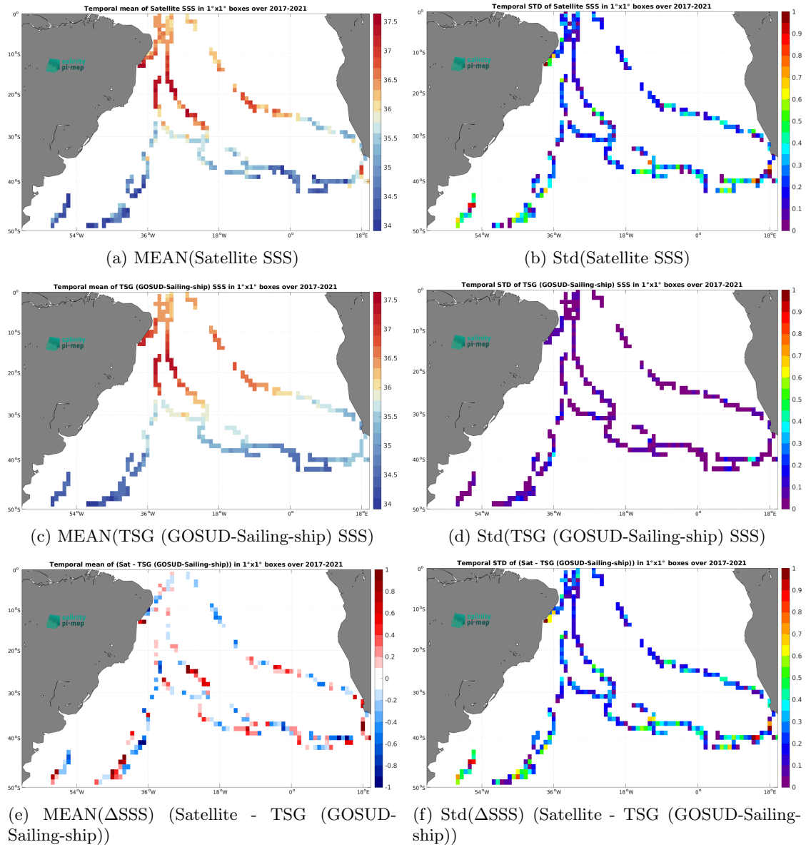
Figure 7: Temporal mean (left) and Std (right) of SSS from SMAP SSS L2 v6 (RSS) (top), TSG (GOSUD-Sailing-ship) (middle), and of \Delta SSS (Satellite - TSG (GOSUD-Sailing-ship)). Only match-up pairs are used to generate these maps.
