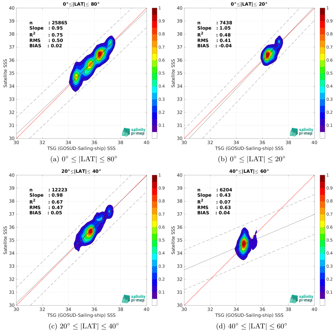
Figure 10: Contour maps of the concentration of SMAP SSS L2 v6 (RSS) SSS (y-axis) versus TSG (GOSUD-Sailing-ship) SSS (x-axis) at match-up pairs for different latitude bands. For each plot, the red line shows x=y . The black thin and dashed lines indicate a linear fit through the data cloud and the \pm 95\% confidence levels, respectively. The number match-up pairs n , the slope and R^2 coefficient of the linear fit, the root mean square (RMS) and the mean bias between satellite and in situ data are indicated for each latitude band in each plots.
