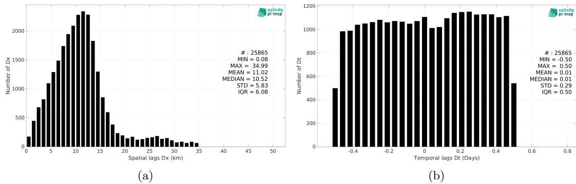
Figure 6: Histograms of the spatial (a) and temporal (b) lags between the location/time of the TSG (GOSUD-Sailing-ship) measurement and the date of the corresponding SMAP SSS L2 v6 (RSS) SSS pixel.
