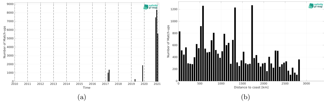
Figure 2: Number of match-ups between TSG (GOSUD-Sailing-ship) and SMAP SSS L2 v6 (RSS) SSS as a function of time (a) and as function of the distance to coast (b) over the South Atlantic Ocean Pi-MEP region and for the full satellite product period.
