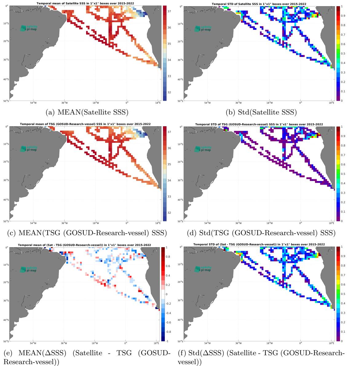
Figure 7: Temporal mean (left) and Std (right) of SSS from SMAP SSS L2 v6 (RSS) (top), TSG (GOSUD-Research-vessel) (middle), and of \Delta SSS (Satellite - TSG (GOSUD-Research-vessel)). Only match-up pairs are used to generate these maps.
