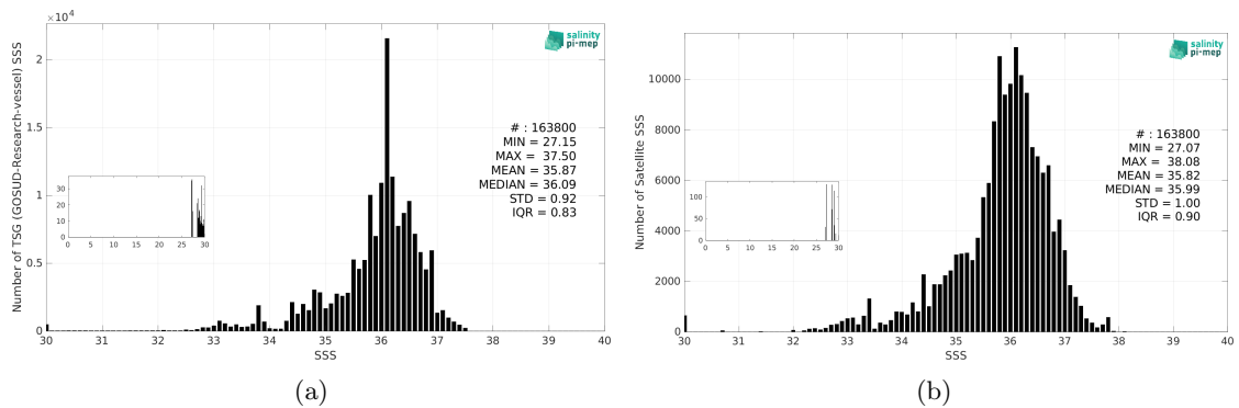
Figure 3: Histograms of SSS from TSG (GOSUD-Research-vessel) (a) and SMAP SSS L2 v6 (RSS) (b) considering all match-up pairs per bins of 0.1 over the South Atlantic Ocean Pi-MEP region and for the full satellite product period.
