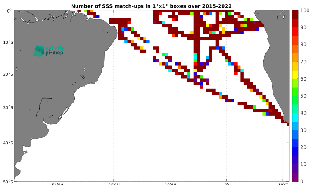
Figure 5: Number of SSS match-ups between TSG (GOSUD-Research-vessel) SSS and the SMAP SSS L2 v6 (RSS) SSS product for the South Atlantic Ocean Pi-MEP region over 1^\circ \times 1^\circ boxes and for the full satellite product period.
