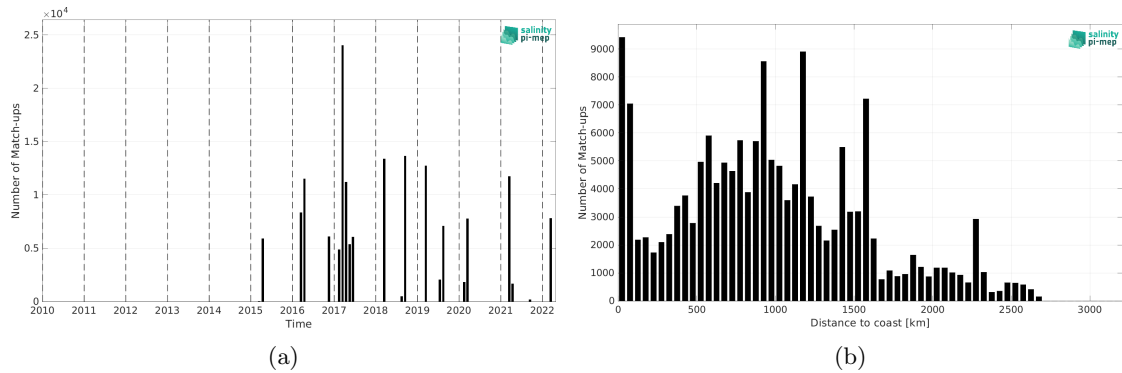
Figure 2: Number of match-ups between TSG (GOSUD-Research-vessel) and SMAP SSS L2 v6 (RSS) SSS as a function of time (a) and as function of the distance to coast (b) over the South Atlantic Ocean Pi-MEP region and for the full satellite product period.
