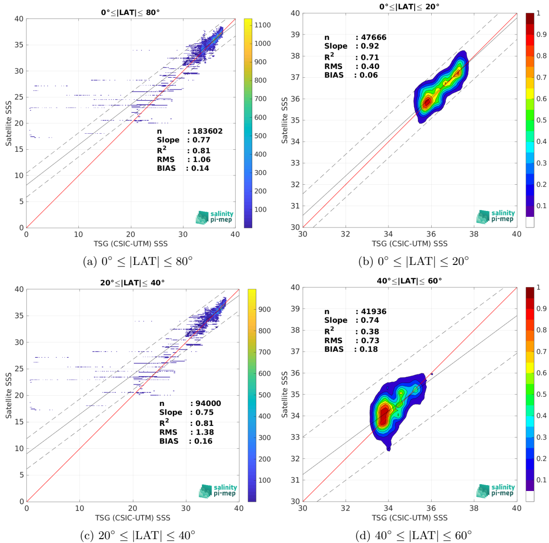
Figure 10: Contour maps of the concentration of SMAP SSS L2 v6 (RSS) SSS ( y -axis) versus TSG (CSIC-UTM) SSS ( x -axis) at match-up pairs for different latitude bands. For each plot, the red line shows x=y . The black thin and dashed lines indicate a linear fit through the data cloud and the \pm 95\% confidence levels, respectively. The number match-up pairs n , the slope and R^2 coefficient of the linear fit, the root mean square (RMS) and the mean bias between satellite and in situ data are indicated for each latitude band in each plots.
