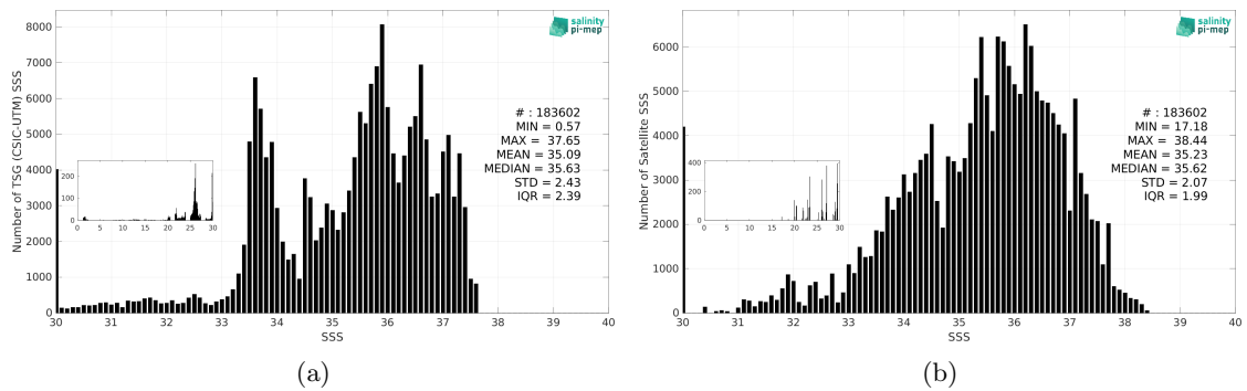
Figure 3: Histograms of SSS from TSG (CSIC-UTM) (a) and SMAP SSS L2 v6 (RSS) (b) considering all match-up pairs per bins of 0.1 over the South Atlantic Ocean Pi-MEP region and for the full satellite product period.
