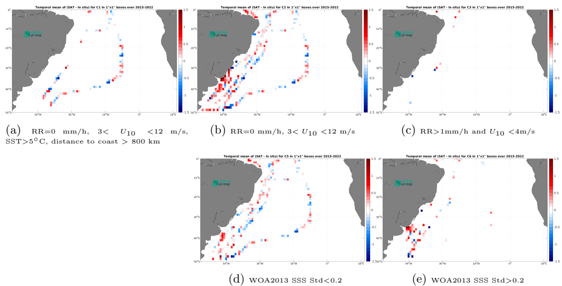
Figure 14: Temporal mean gridded over spatial boxes of size 1^\circ \times 1^\circ of \Delta SSS (SMAP SSS L2 v6 (RSS) - TSG (CSIC-UTM)) for 5 different subdatasets corresponding to:RR=0 mm/h, 3 < U_{10} < 12 m/s, SST >5^\circ\text{C} , distance to coast > 800 km (a), RR=0 mm/h, 3 < U_{10} < 12 m/s (b), RR >1 mm/h and U_{10} < 4 m/s (c), WOA2013 SSS Std <0.2 (d), WOA2013 SSS Std >0.2 (e).
