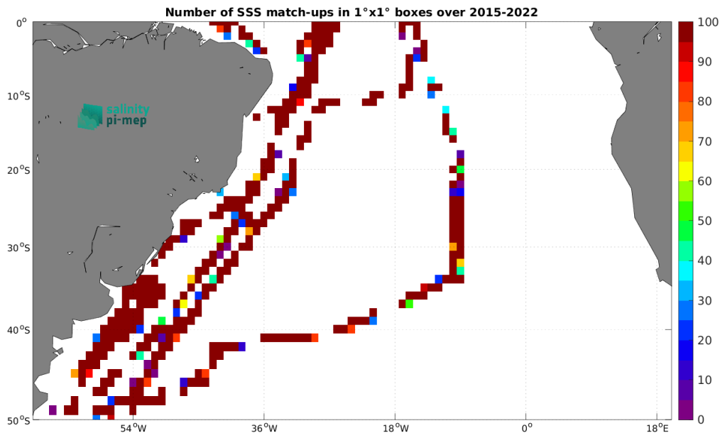
Figure 5: Number of SSS match-ups between TSG (CSIC-UTM) SSS and the SMAP SSS L2 v6 (RSS) SSS product for the South Atlantic Ocean Pi-MEP region over 1^\circ \times 1^\circ boxes and for the full satellite product period.
