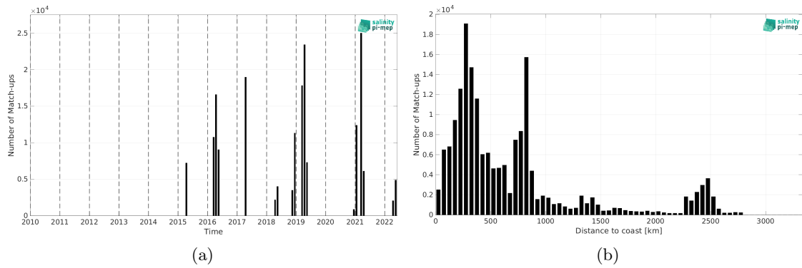
Figure 2: Number of match-ups between TSG (CSIC-UTM) and SMAP SSS L2 v6 (RSS) SSS as a function of time (a) and as function of the distance to coast (b) over the South Atlantic Ocean Pi-MEP region and for the full satellite product period.
