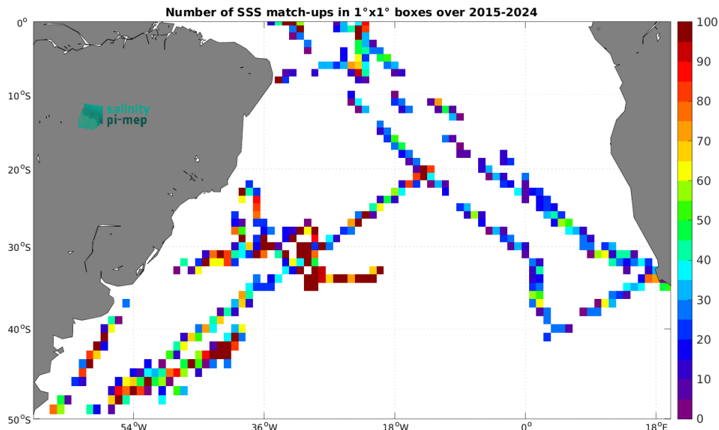
Figure 5: Number of SSS match-ups between TSG (SAMOS) SSS and the SMAP SSS L2 v6 - 40 km (RSS) SSS product for the South Atlantic Ocean Pi-MEP region over 1^\circ \times 1^\circ boxes and for the full satellite product period.
