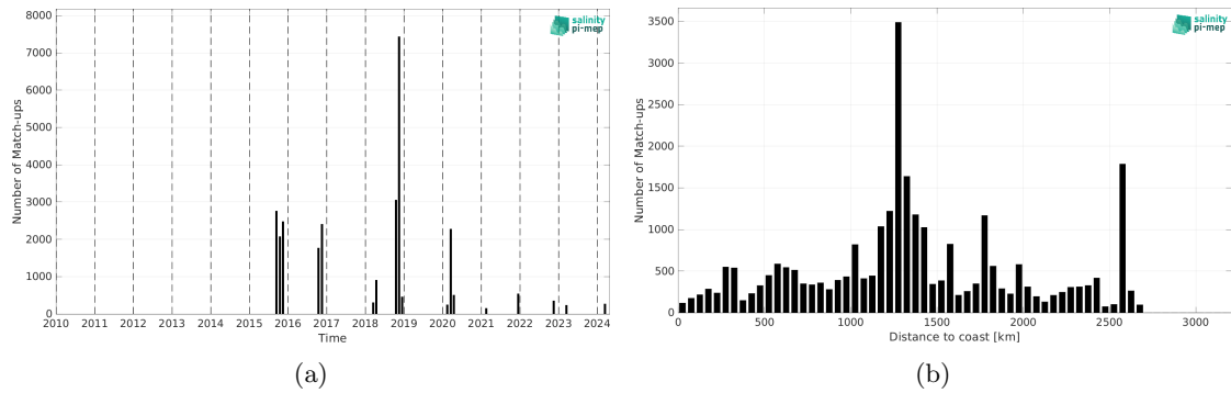
Figure 2: Number of match-ups between TSG (SAMOS) and SMAP SSS L2 v6 - 40 km (RSS) SSS as a function of time (a) and as function of the distance to coast (b) over the South Atlantic Ocean Pi-MEP region and for the full satellite product period.
