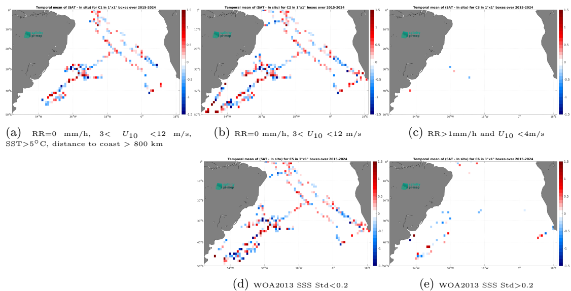
Figure 14: Temporal mean gridded over spatial boxes of size 1^\circ \times 1^\circ of \Delta\text{SSS} (SMAP SSS L2 v6 - 40 km (RSS) - TSG (SAMOS)) for 5 different subdatasets corresponding to:RR=0 mm/h, 3 < U_{10} < 12 m/s, SST >5^\circ\text{C} , distance to coast > 800 km (a), RR=0 mm/h, 3 < U_{10} < 12 m/s (b), RR >1 mm/h and U_{10} < 4 m/s (c), WOA2013 SSS Std <0.2 (d), WOA2013 SSS Std >0.2 (e).
