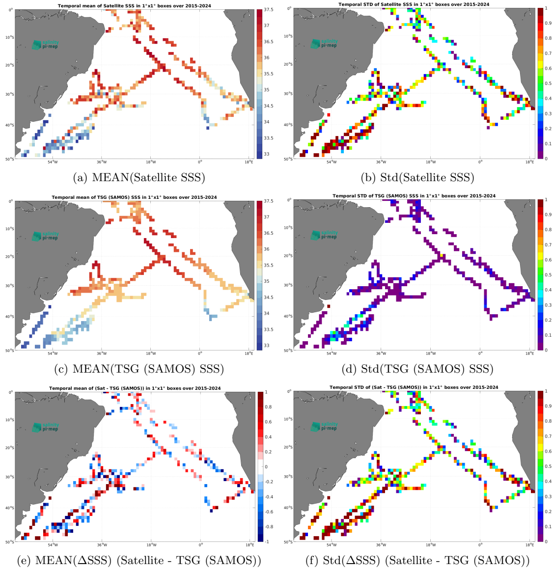
Figure 7: Temporal mean (left) and Std (right) of SSS from SMAP SSS L2 v6 - 40 km (RSS) (top), TSG (SAMOS) (middle), and of \Delta SSS (Satellite - TSG (SAMOS)). Only match-up pairs are used to generate these maps.
