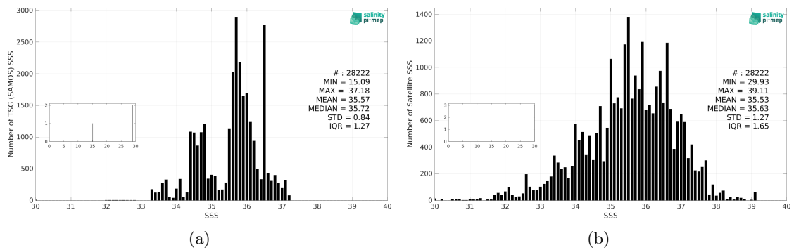
Figure 3: Histograms of SSS from TSG (SAMOS) (a) and SMAP SSS L2 v6 - 40 km (RSS) (b) considering all match-up pairs per bins of 0.1 over the South Atlantic Ocean Pi-MEP region and for the full satellite product period.
