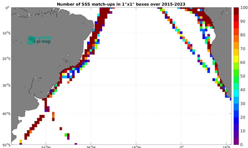
Figure 5: Number of SSS match-ups between TSG (LEGOS-DM) SSS and the SMAP SSS L2 v6 - 40 km (RSS) SSS product for the South Atlantic Ocean Pi-MEP region over 1^\circ \times 1^\circ boxes and for the full satellite product period.
