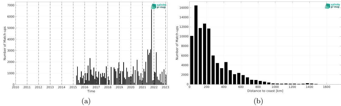
Figure 2: Number of match-ups between TSG (LEGOS-DM) and SMAP SSS L2 v6 - 40 km (RSS) SSS as a function of time (a) and as function of the distance to coast (b) over the South Atlantic Ocean Pi-MEP region and for the full satellite product period.
