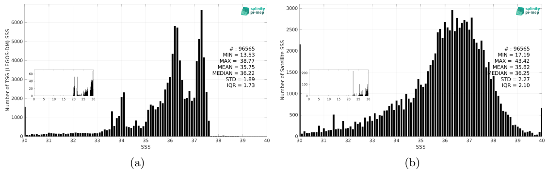
Figure 3: Histograms of SSS from TSG (LEGOS-DM) (a) and SMAP SSS L2 v6 - 40 km (RSS) (b) considering all match-up pairs per bins of 0.1 over the South Atlantic Ocean Pi-MEP region and for the full satellite product period.
