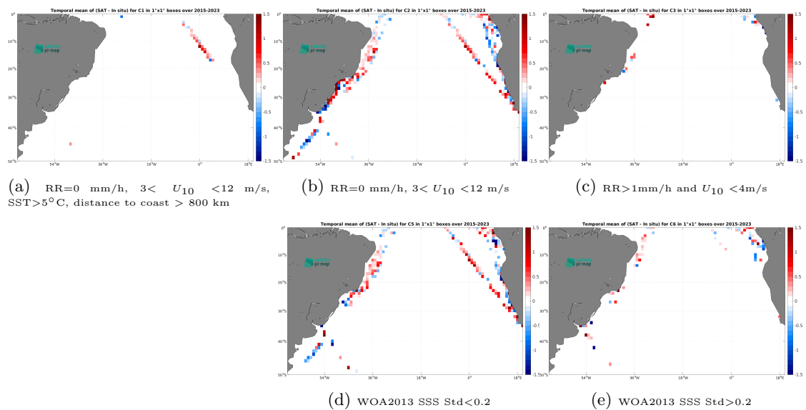
Figure 14: Temporal mean gridded over spatial boxes of size 1^\circ \times 1^\circ of \Delta\text{SSS} (SMAP SSS L2 v6 - 40 km (RSS) - TSG (LEGOS-DM)) for 5 different subdatasets corresponding to:RR=0 mm/h, 3 < U_{10} < 12 m/s, SST >5^\circ\text{C} , distance to coast > 800 km (a), RR=0 mm/h, 3 < U_{10} < 12 m/s (b), RR >1 mm/h and U_{10} < 4 m/s (c), WOA2013 SSS Std <0.2 (d), WOA2013 SSS Std >0.2 (e).
