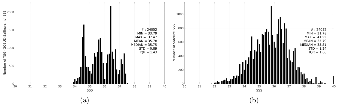
Figure 3: Histograms of SSS from TSG (GOSUD-Sailing-ship) (a) and SMAP SSS L2 v6 - 40 km (RSS) (b) considering all match-up pairs per bins of 0.1 over the South Atlantic Ocean Pi-MEP region and for the full satellite product period.
