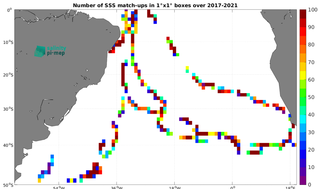
Figure 5: Number of SSS match-ups between TSG (GOSUD-Sailing-ship) SSS and the SMAP SSS L2 v6 - 40 km (RSS) SSS product for the South Atlantic Ocean Pi-MEP region over 1^\circ \times 1^\circ boxes and for the full satellite product period.
