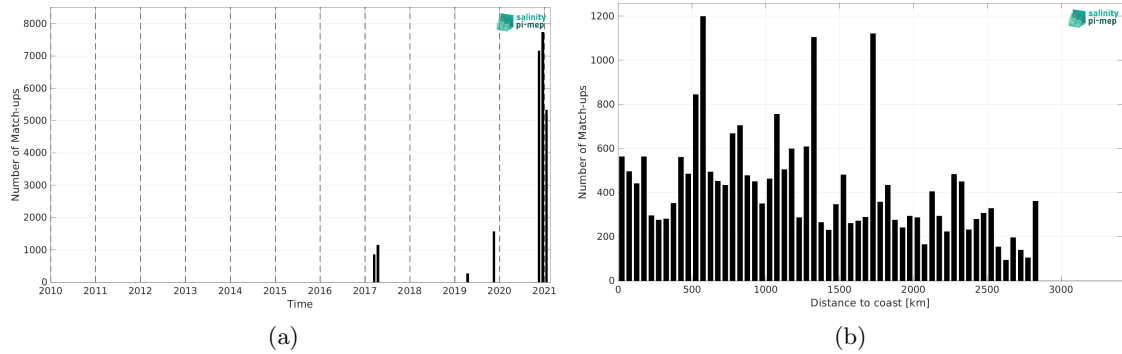
Figure 2: Number of match-ups between TSG (GOSUD-Sailing-ship) and SMAP SSS L2 v6 - 40 km (RSS) SSS as a function of time (a) and as function of the distance to coast (b) over the South Atlantic Ocean Pi-MEP region and for the full satellite product period.
