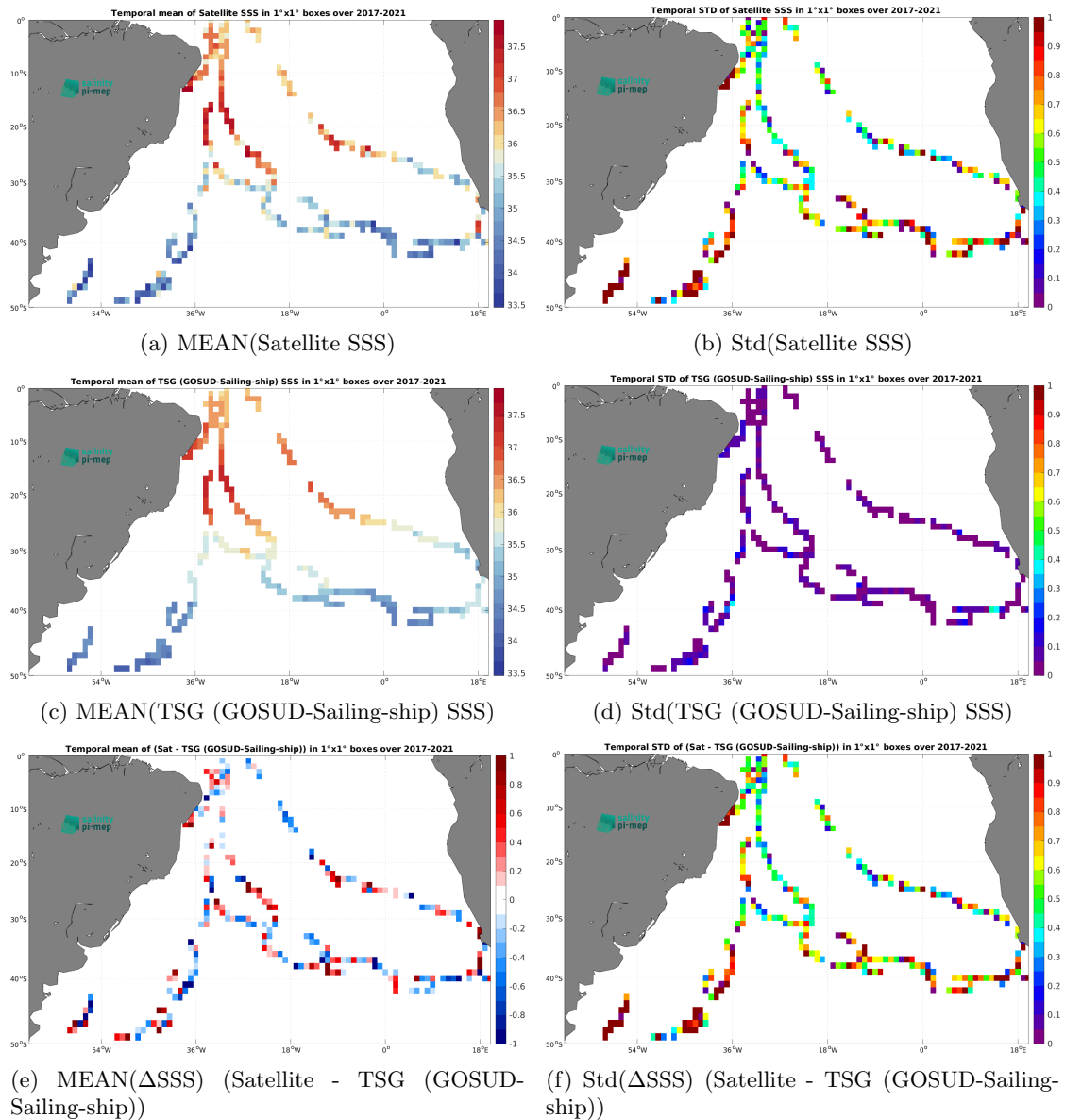
Figure 7: Temporal mean (left) and Std (right) of SSS from SMAP SSS L2 v6 - 40 km (RSS) (top), TSG (GOSUD-Sailing-ship) (middle), and of \Delta SSS (Satellite - TSG (GOSUD-Sailing-ship)). Only match-up pairs are used to generate these maps.
