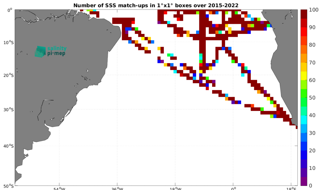
Figure 5: Number of SSS match-ups between TSG (GOSUD-Research-vessel) SSS and the SMAP SSS L2 v6 - 40 km (RSS) SSS product for the South Atlantic Ocean Pi-MEP region over 1^\circ \times 1^\circ boxes and for the full satellite product period.
