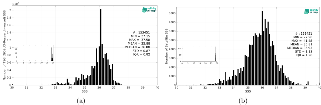
Figure 3: Histograms of SSS from TSG (GOSUD-Research-vessel) (a) and SMAP SSS L2 v6 - 40 km (RSS) (b) considering all match-up pairs per bins of 0.1 over the South Atlantic Ocean Pi-MEP region and for the full satellite product period.
