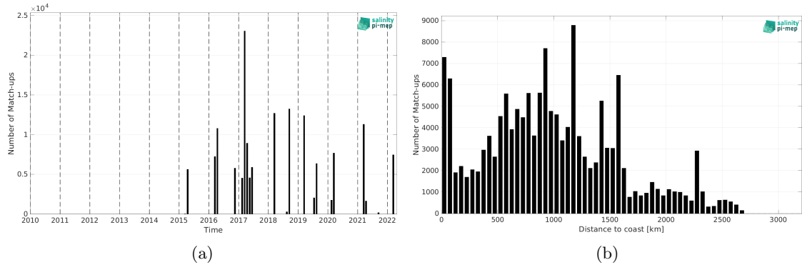
Figure 2: Number of match-ups between TSG (GOSUD-Research-vessel) and SMAP SSS L2 v6 - 40 km (RSS) SSS as a function of time (a) and as function of the distance to coast (b) over the South Atlantic Ocean Pi-MEP region and for the full satellite product period.
