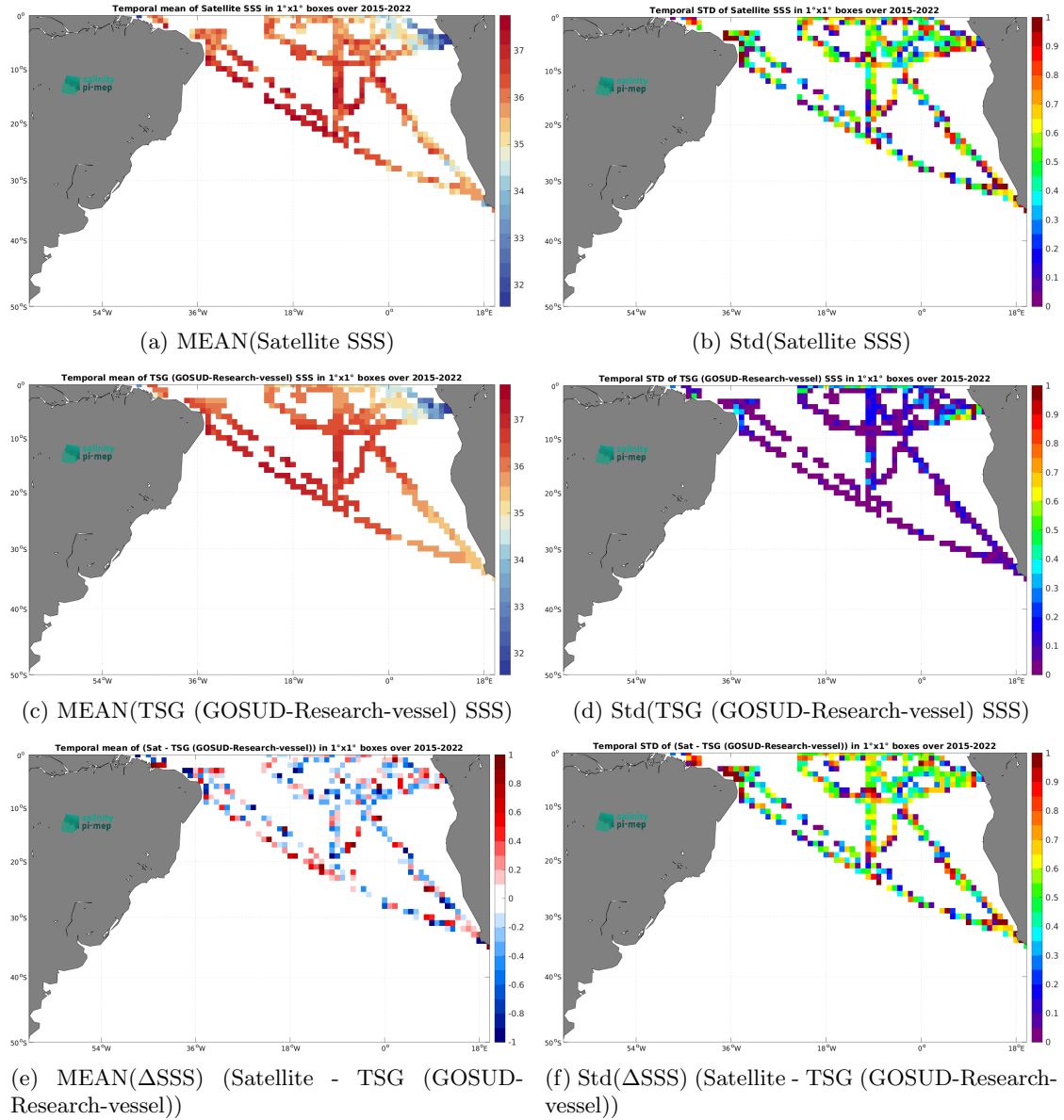
Figure 7: Temporal mean (left) and Std (right) of SSS from SMAP SSS L2 v6 - 40 km (RSS) (top), TSG (GOSUD-Research-vessel) (middle), and of \Delta SSS (Satellite - TSG (GOSUD-Research-vessel)). Only match-up pairs are used to generate these maps.
