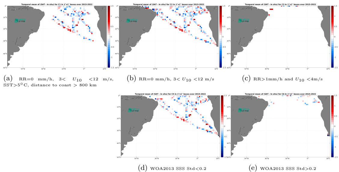
Figure 14: Temporal mean gridded over spatial boxes of size 1^\circ \times 1^\circ of \Delta SSS (SMAP SSS L2 v6 - 40 km (RSS) - TSG (GOSUD-Research-vessel)) for 5 different subdatasets corresponding to:RR=0 mm/h, 3 < U_{10} < 12 m/s, SST>5°C, distance to coast > 800 km (a), RR=0 mm/h, 3 < U_{10} < 12 m/s (b), RR>1mm/h and U_{10} < 4 m/s (c), WOA2013 SSS Std<0.2 (d), WOA2013 SSS Std>0.2 (e).
